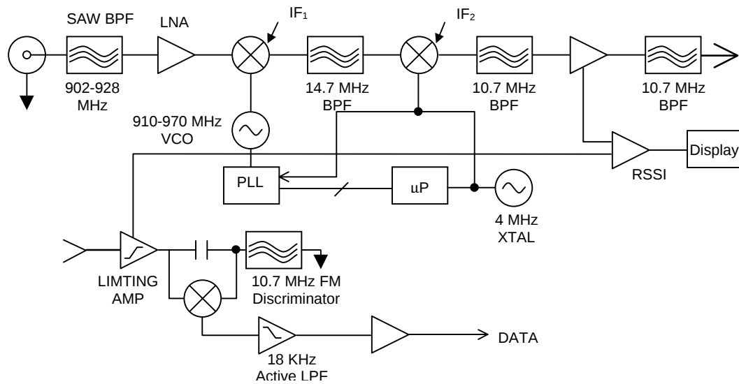
900 MHz Receiver Block Diagram
