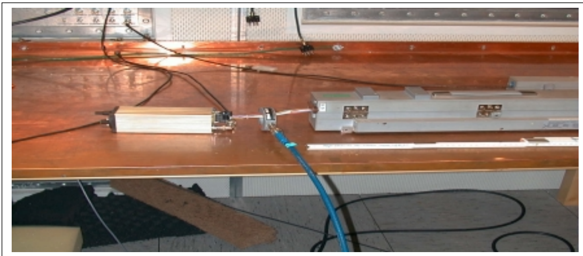
FSG 2T Test Setup for 200 MHz – 400 MHz (FISCHER CUSTOM Communications Model F-62)
