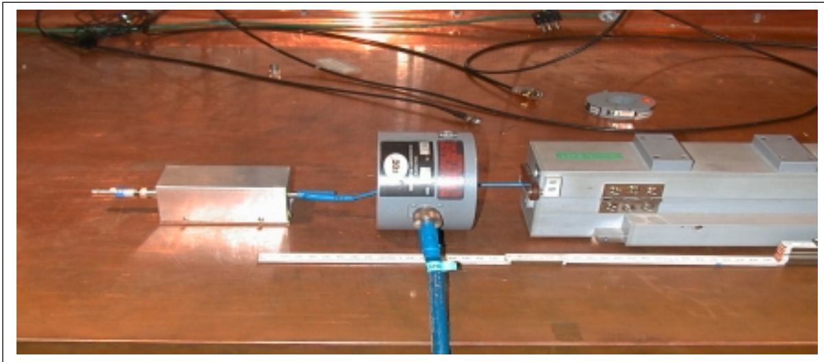
Monitor Probe Calibration 10 kHz –200 MHz (FISCHER CUSTOM Communications Model F-120-4) using a 50-Ohm Load. This results in a Category T Voltage of 1.125 V for 7.5 mA Test Current, and for 200 MHz – 400 MHz (FISCHER CUSTOM Communications Model F-62)
