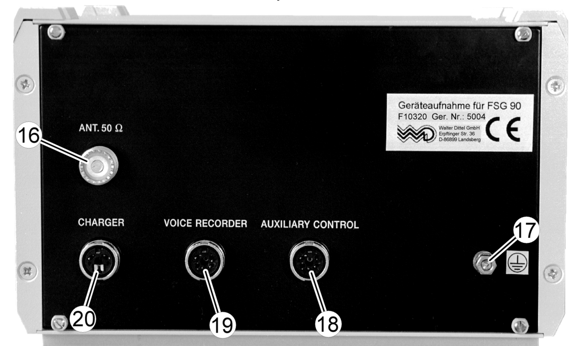
Desktop Base Station Front and rear view with transceiver FSG 90 installed
