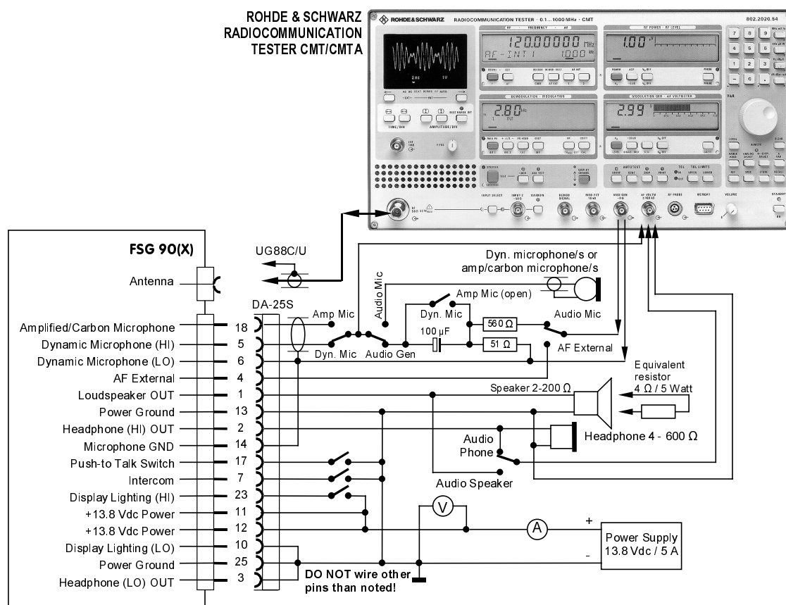
Figure 8-3 Recommended Test Setup
