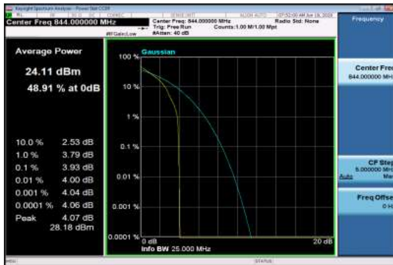
Band5-10MHz-QPSK-20600-50RB#0
