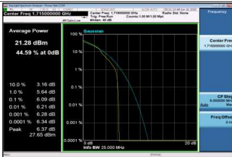
Band4-10MHz-16QAM-20000-50RB#0
