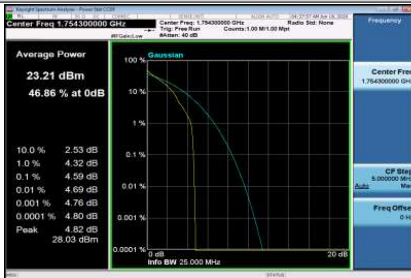
Band4-1.4MHz-QPSK-20393-6RB#0
