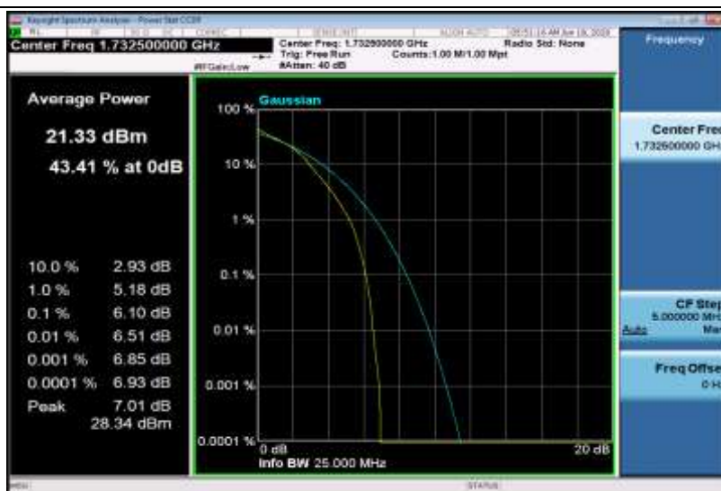
Band4-15MHz-16QAM-20325-1RB#0
