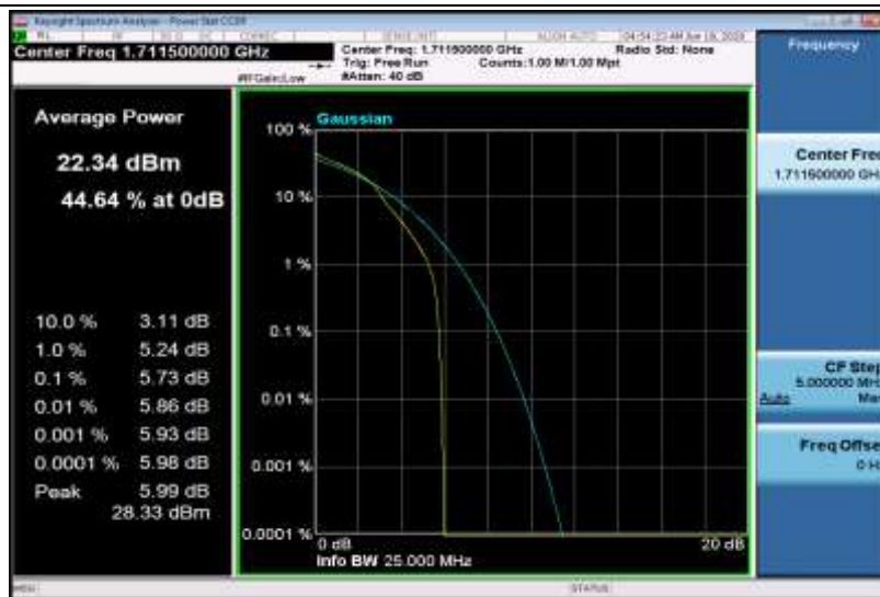
Band4-3MHz-16QAM-19965-15RB#0
