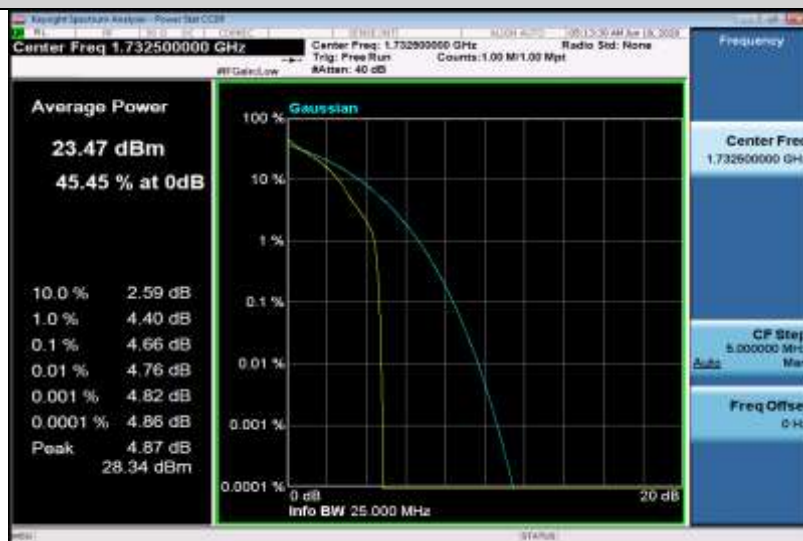
Band4-5MHz-QPSK-20175-25RB#0
