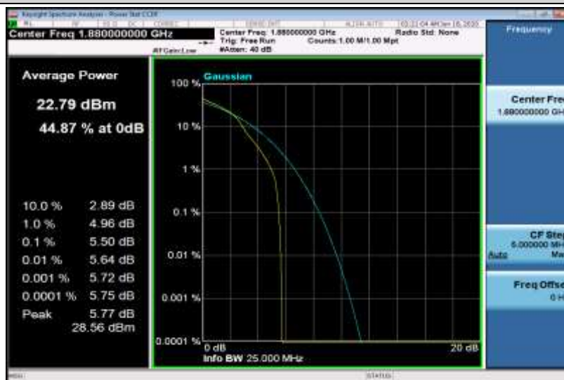
Band2-1.4MHz-16QAM-18900-6RB#0
