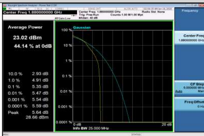
Band2-5MHz-16QAM-18900-25RB#0
