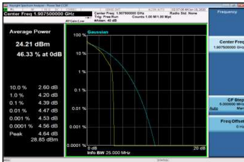
Band2-5MHz-QPSK-19175-25RB#0
