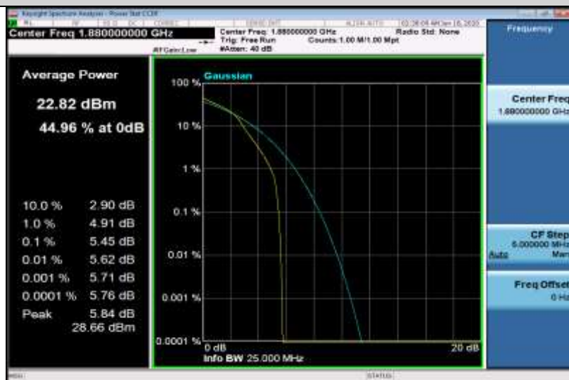
Band2-3MHz-16QAM-18900-15RB#0
