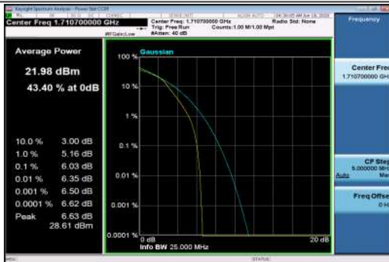
Band4-1.4MHz-16QAM-20175-1RB#0
