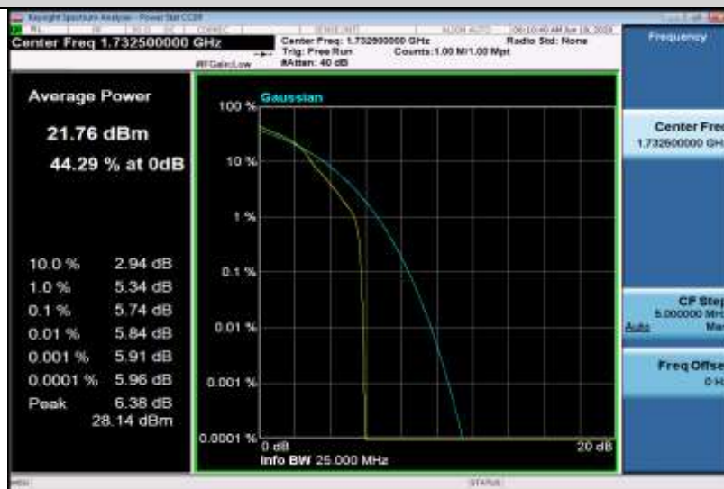
Band4-20MHz-16QAM-20175-100RB#0
