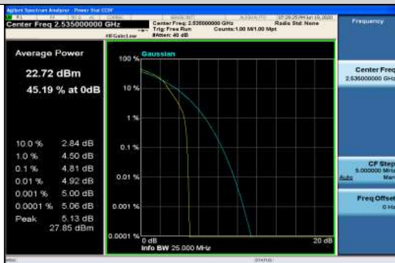
Band7-20MHz-16QAM-21100-100RB#0
