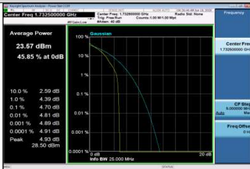
Band4-1.4MHz-QPSK-20175-6RB#0
