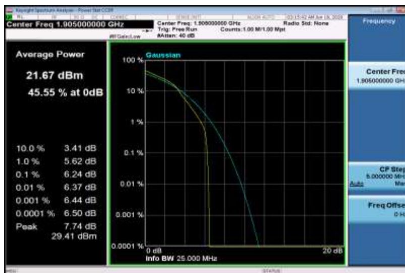
Band2-10MHz-16QAM-19150-50RB#0
