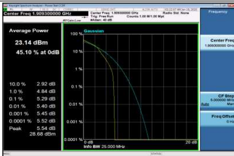
Band2-1.4MHz-16QAM-19193-6RB#0
