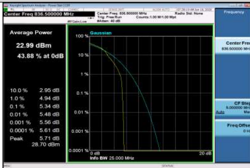
Band5-5MHz-16QAM-20525-25RB#0
