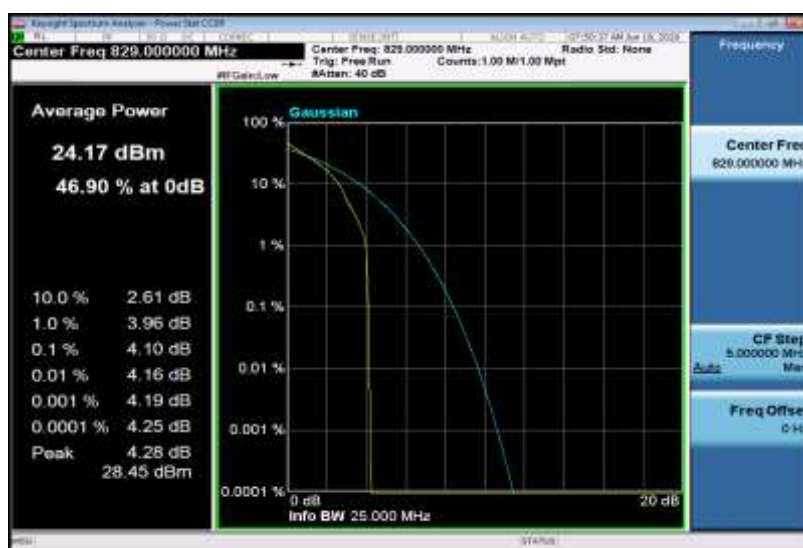
Band5-10MHz-QPSK-20450-50RB#0
