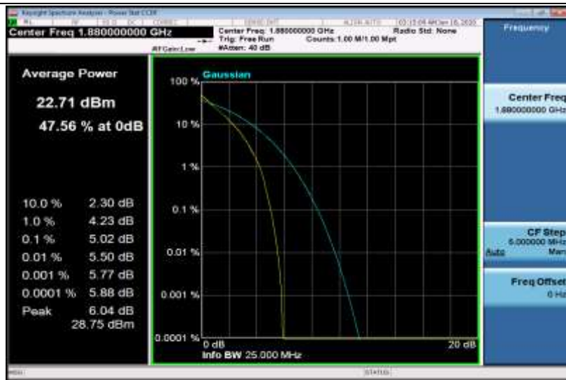
Band2-10MHz-QPSK-19150-1RB#0
