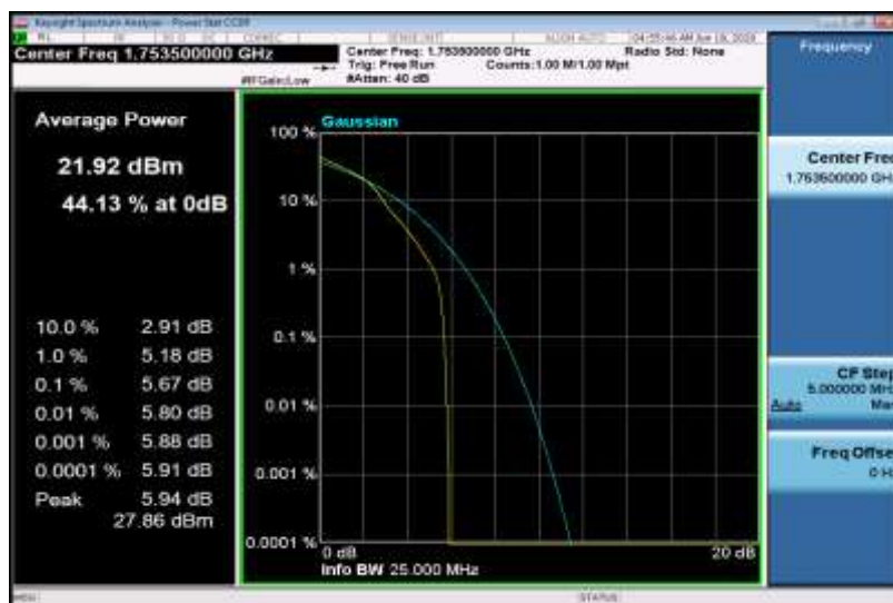
Band4-3MHz-16QAM-20385-15RB#0
