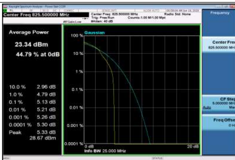
Band5-3MHz-16QAM-20415-15RB#0
