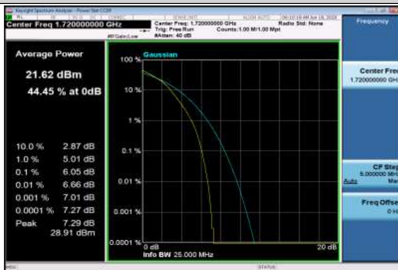
Band4-20MHz-16QAM-20175-1RB#0
