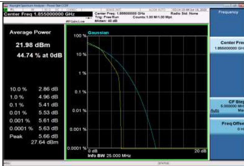
Band2-10MHz-16QAM-18650-50RB#0
