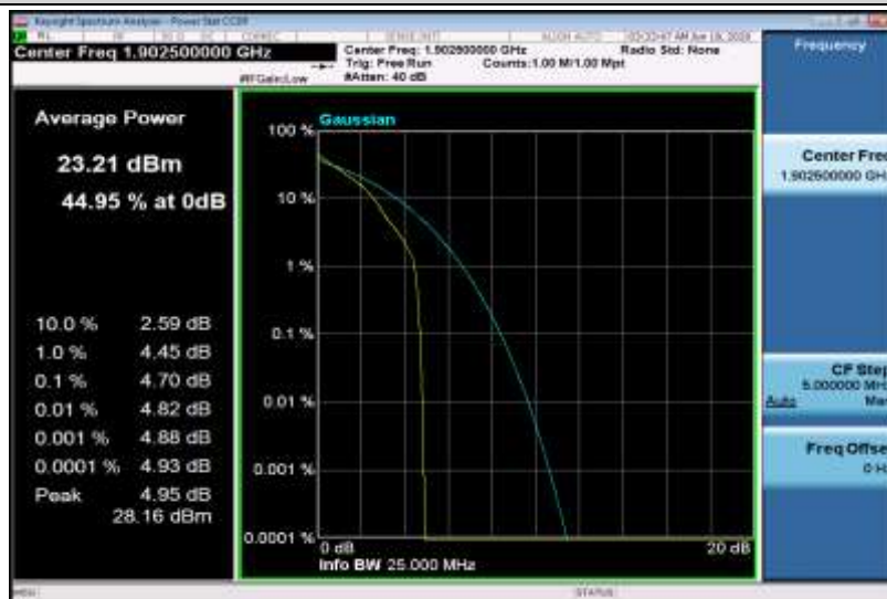
Band2-15MHz-QPSK-19125-75RB#0
