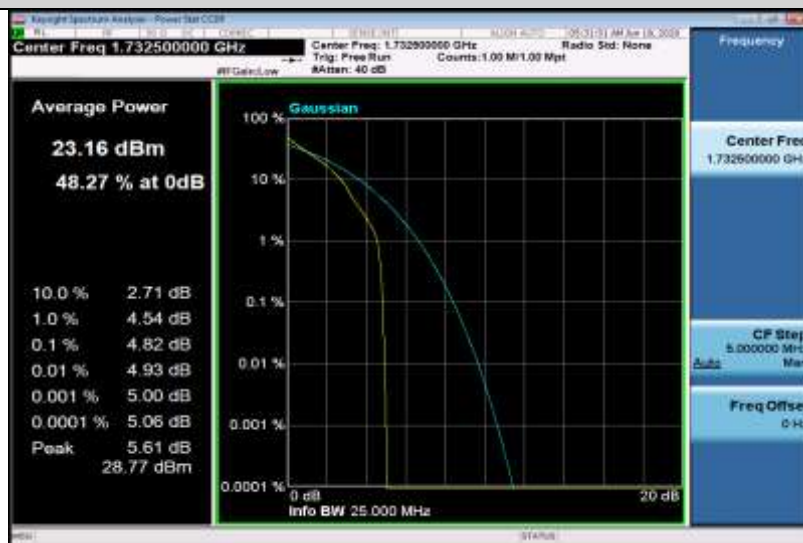
Band4-10MHz-QPSK-20175-50RB#0
