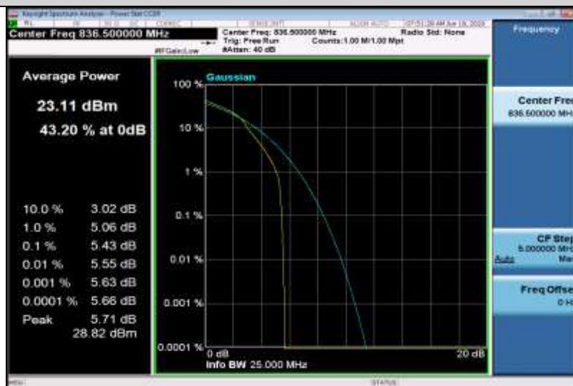
Band5-10MHz-16QAM-20525-50RB#0
