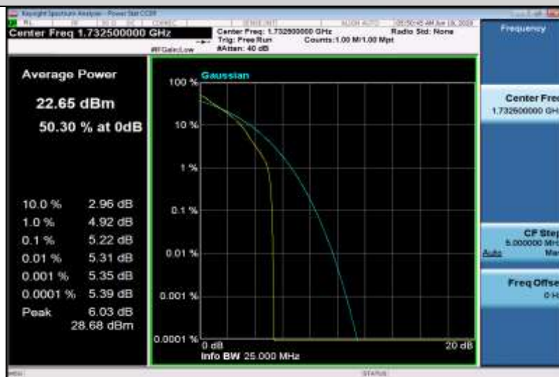
Band4-15MHz-QPSK-20175-75RB#0
