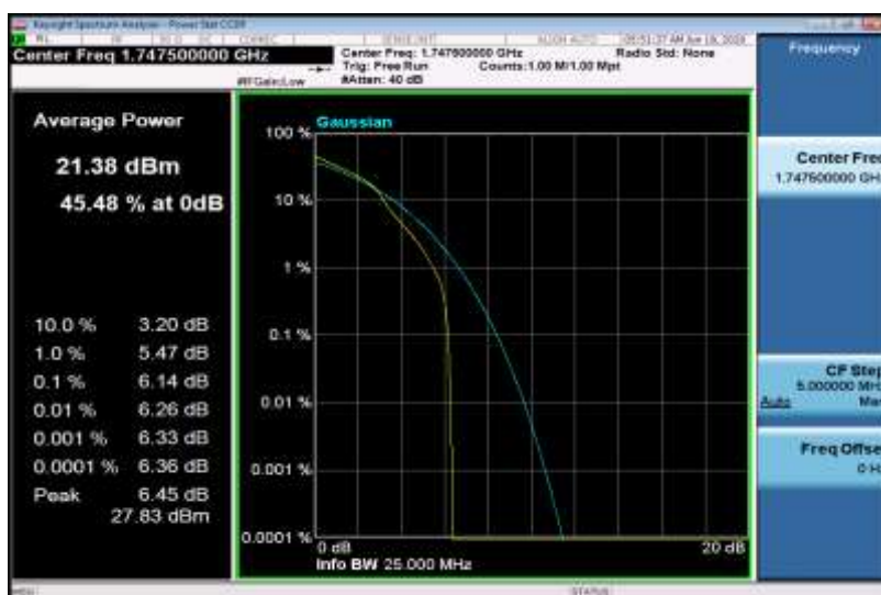
Band4-15MHz-16QAM-20325-75RB#0
