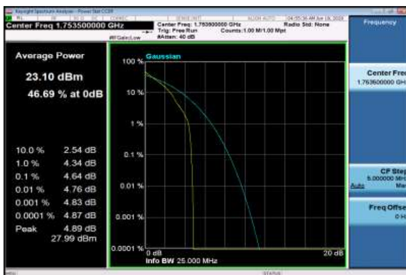
Band4-3MHz-QPSK-20385-15RB#0
