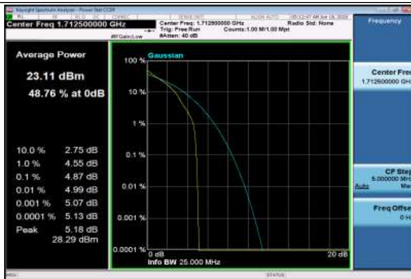
Band4-5MHz-QPSK-19975-25RB#0
