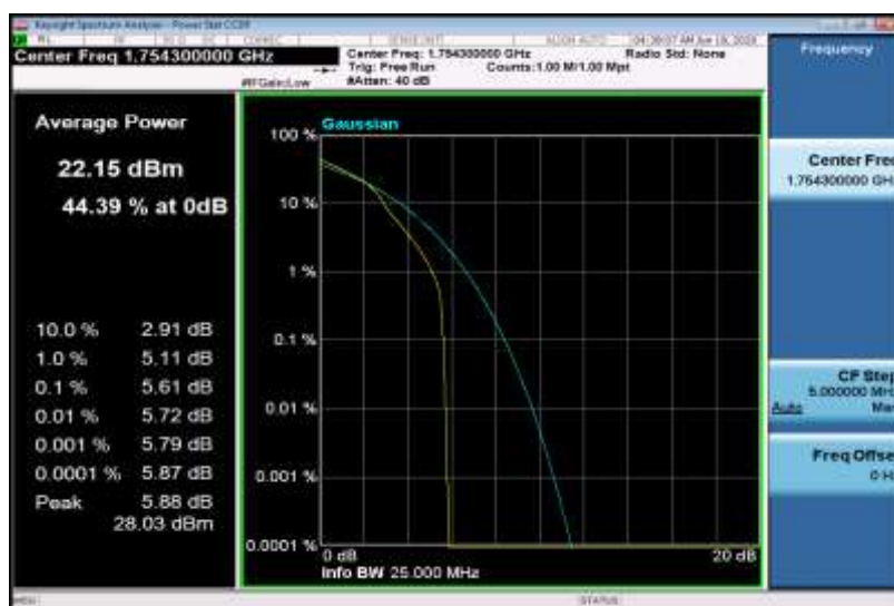
Band4-1.4MHz-16QAM-20393-6RB#0
