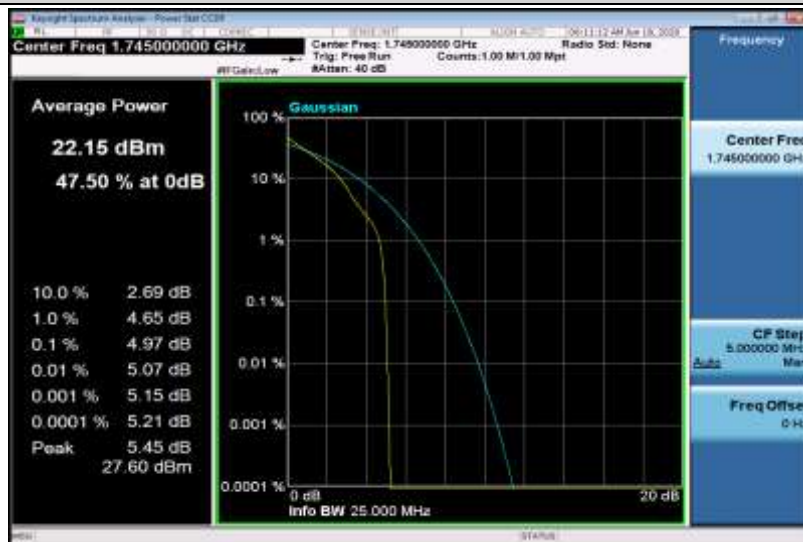
Band4-20MHz-QPSK-20300-100RB#0
