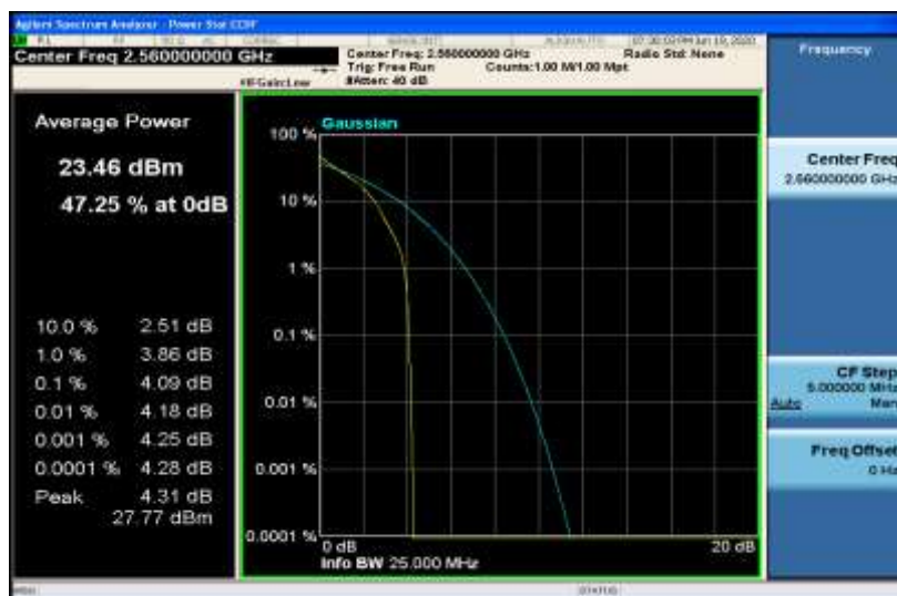
Band7-20MHz-QPSK-21350-100RB#0
