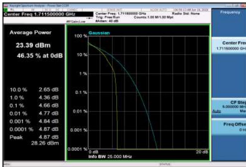
Band4-3MHz-QPSK-19965-15RB#0
