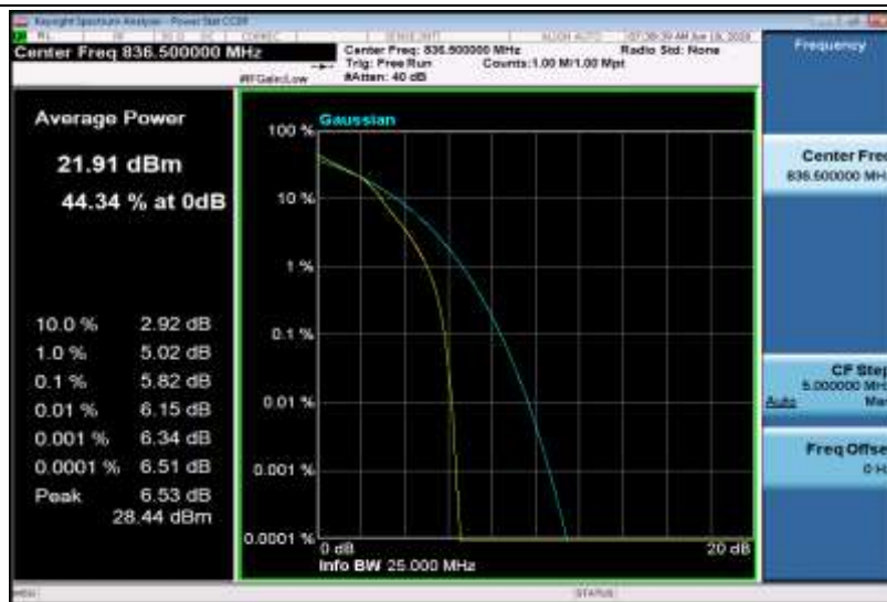
Band5-5MHz-16QAM-20625-1RB#0
