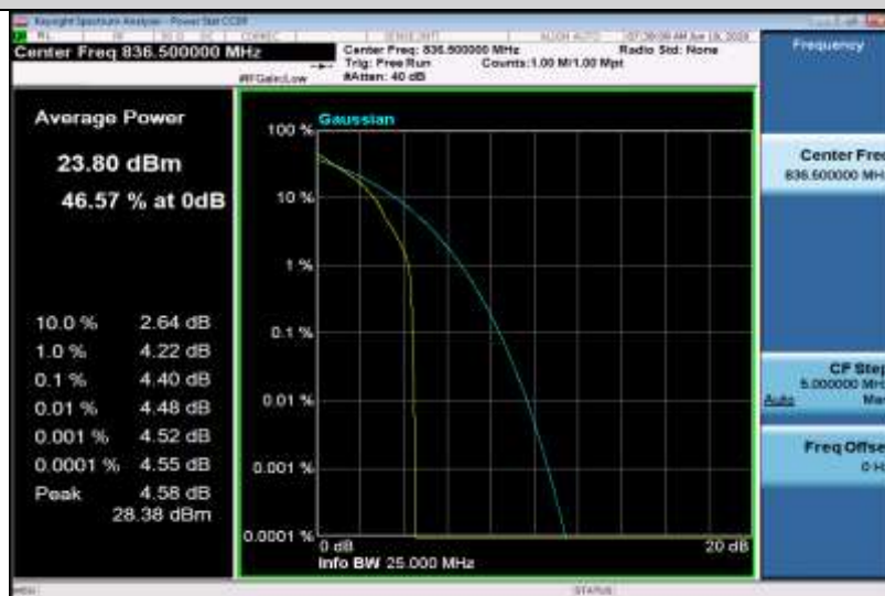
Band5-5MHz-QPSK-20525-25RB#0
