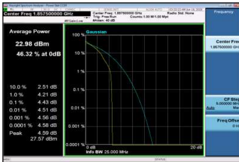
Band2-15MHz-QPSK-18675-75RB#0
