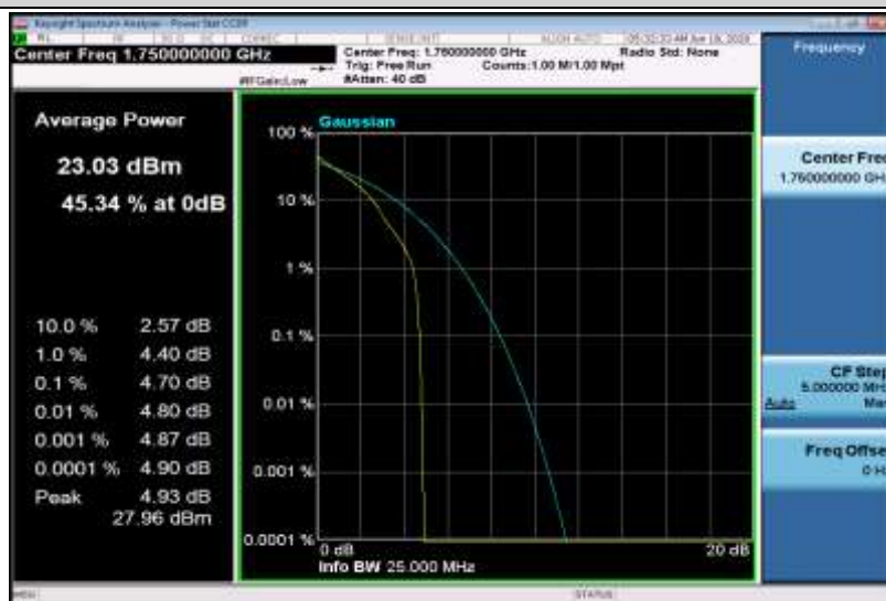
Band4-10MHz-QPSK-20350-50RB#0
