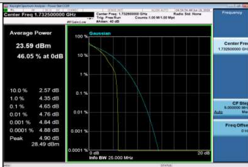
Band4-3MHz-QPSK-20175-15RB#0
