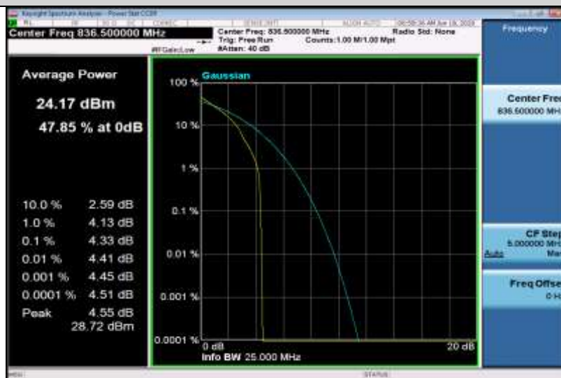
Band5-3MHz-QPSK-20525-15RB#0
