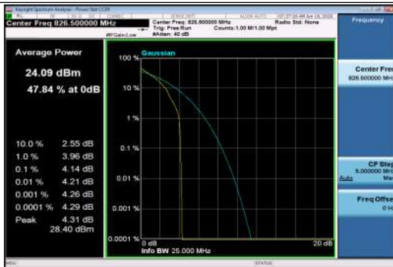
Band5-5MHz-QPSK-20425-25RB#0
