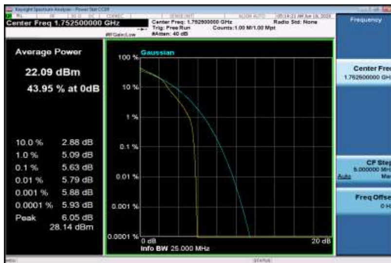
Band4-5MHz-16QAM-20375-25RB#0
