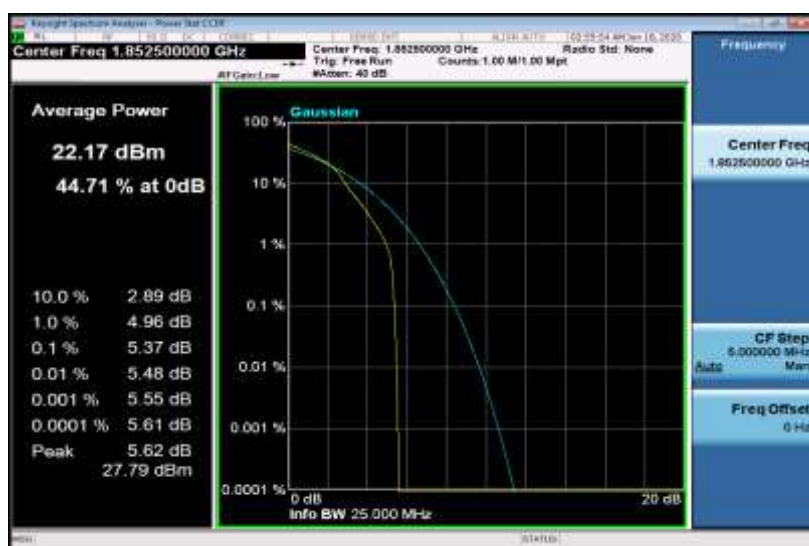
Band2-5MHz-16QAM-18625-25RB#0
