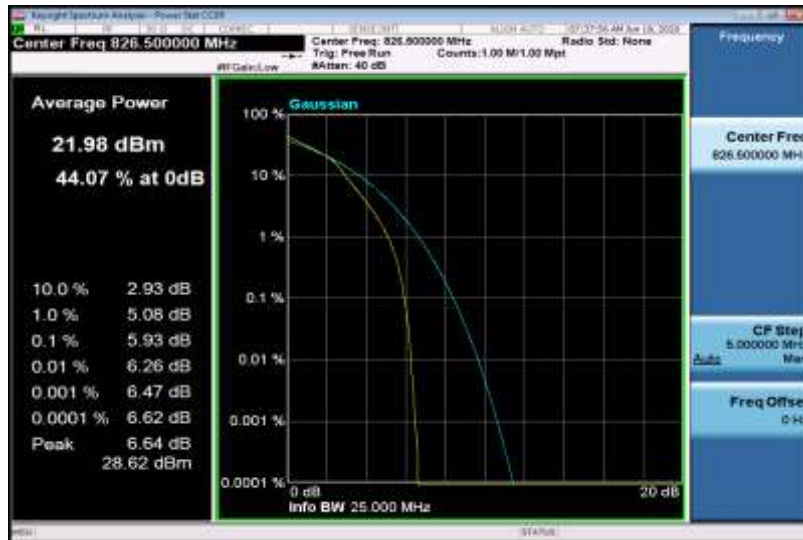
Band5-5MHz-16QAM-20525-1RB#0
