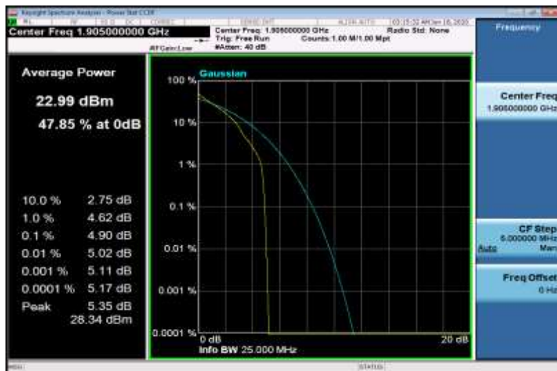
Band2-10MHz-QPSK-19150-50RB#0
