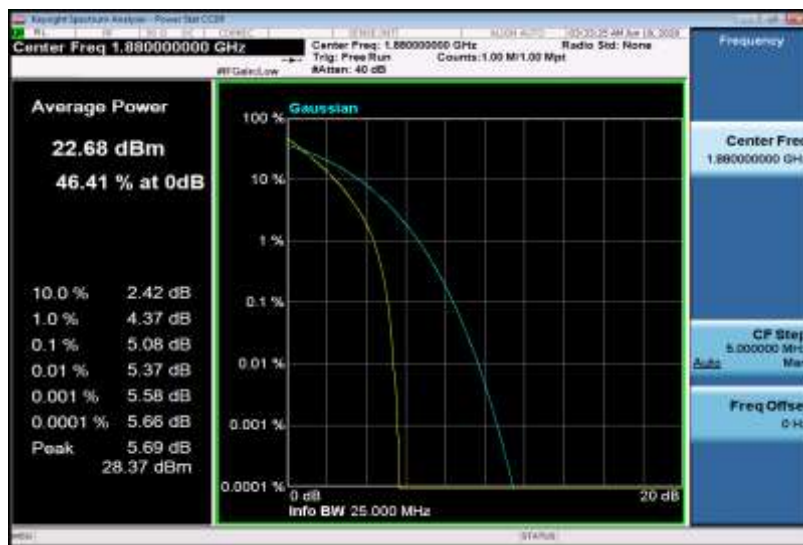
Band2-15MHz-QPSK-19125-1RB#0
