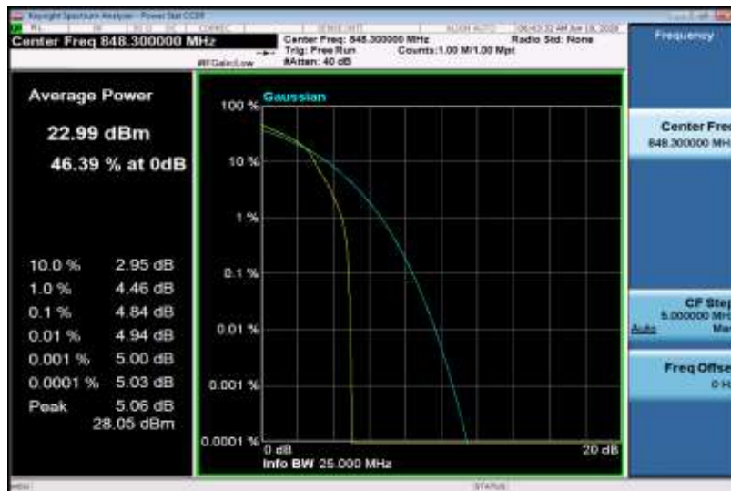
Band5-1.4MHz-16QAM-20643-6RB#0
