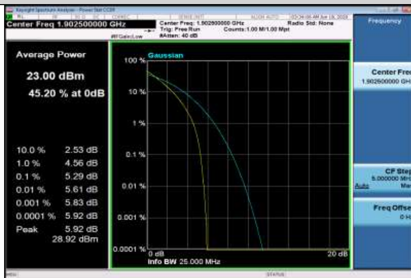
Band2-15MHz-16QAM-18675-1RB#0
