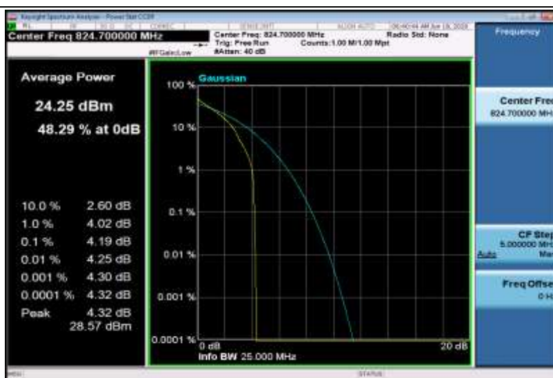
Band5-1.4MHz-QPSK-20407-6RB#0
