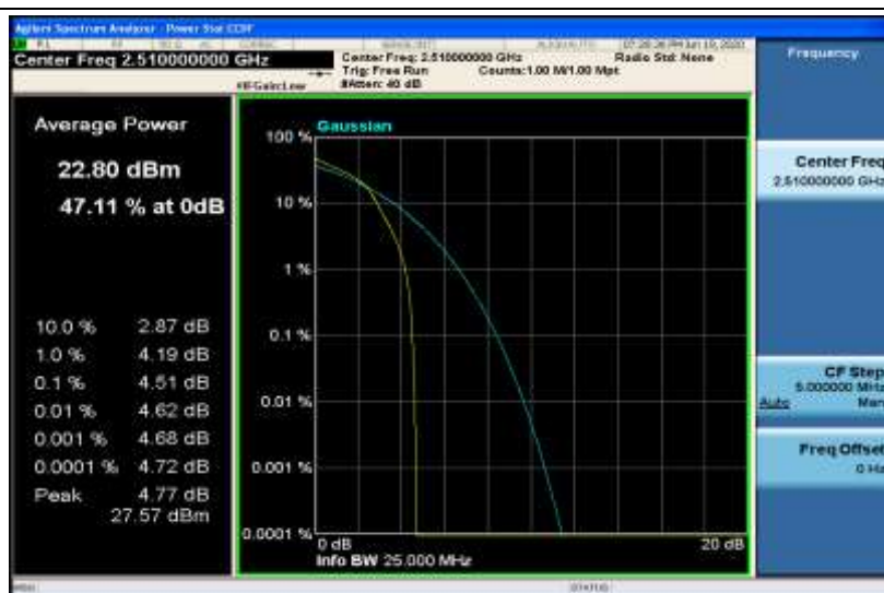
Band7-20MHz-16QAM-20850-100RB#0
