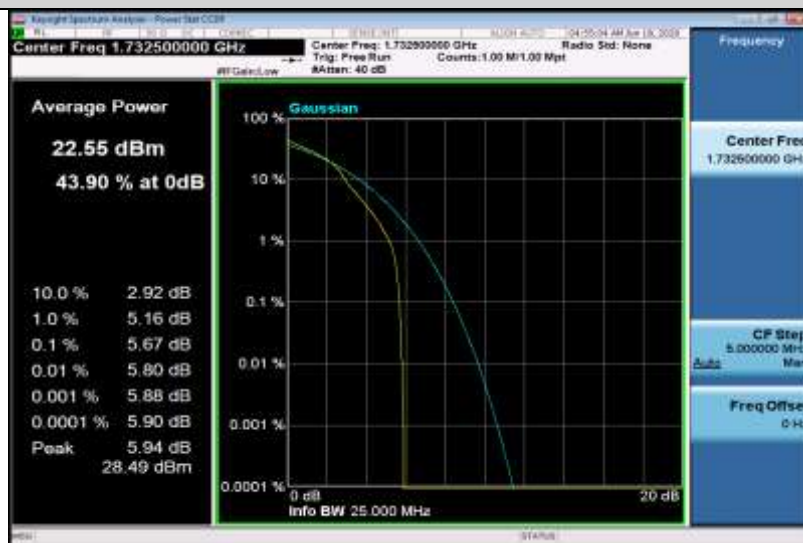
Band4-3MHz-16QAM-20175-15RB#0
