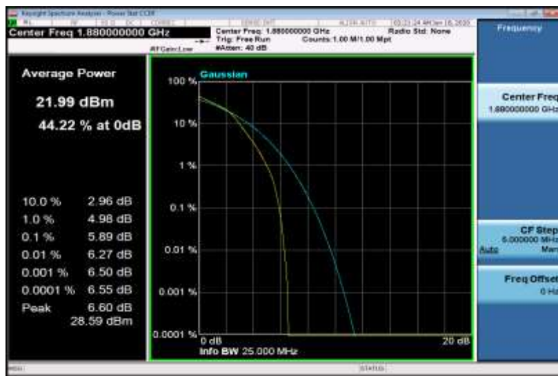
Band2-1.4MHz-16QAM-19193-1RB#0
