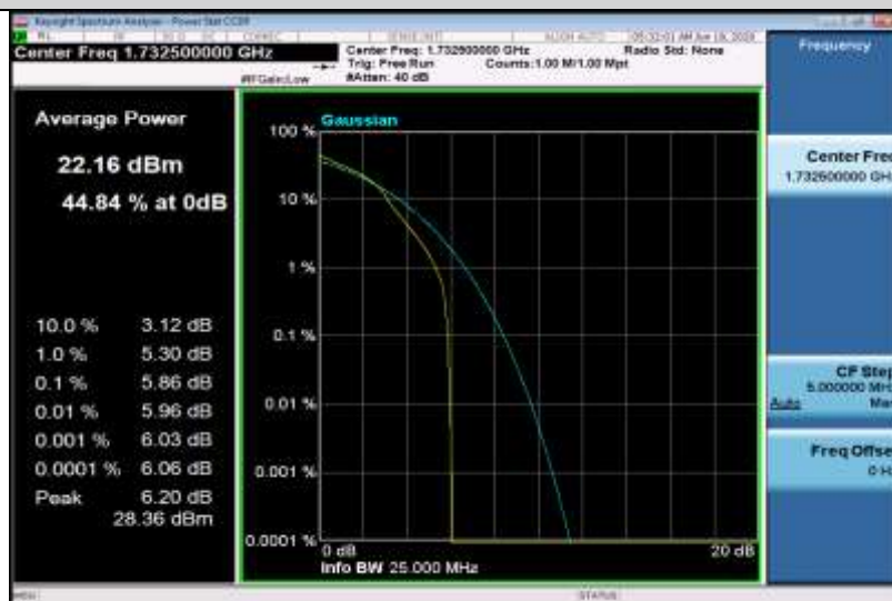
Band4-10MHz-16QAM-20175-50RB#0
