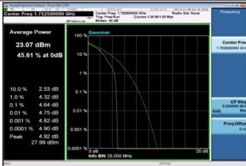
Band4-5MHz-QPSK-20375-25RB#0
