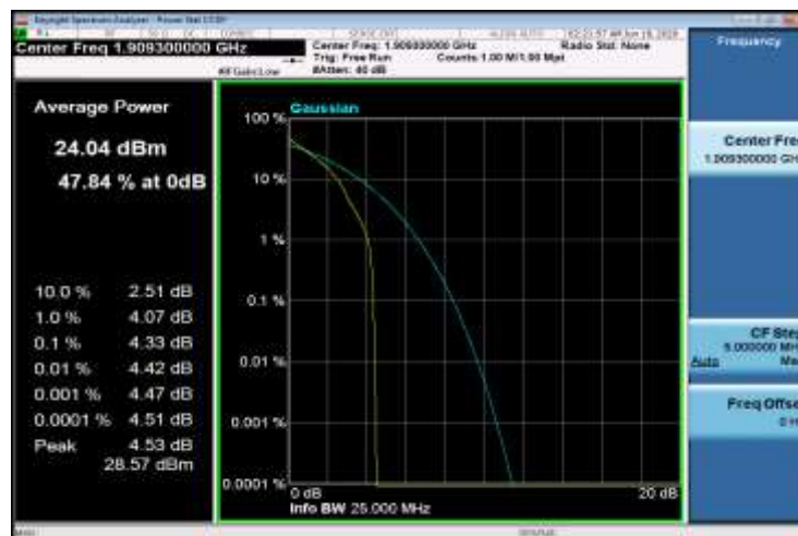
Band2-1.4MHz-QPSK-19193-6RB#0
