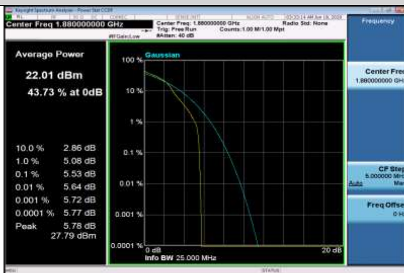
Band2-15MHz-16QAM-18900-75RB#0
