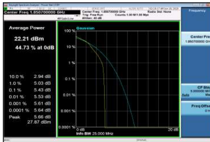
Band2-1.4MHz-16QAM-18607-6RB#0
