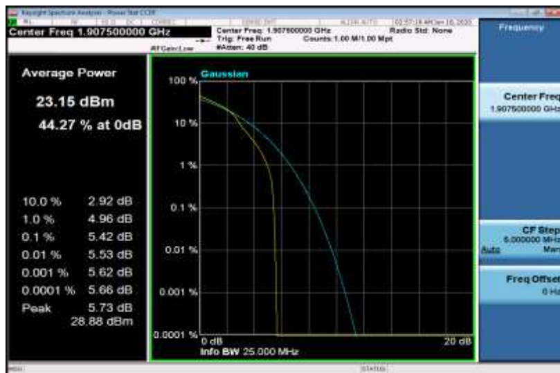
Band2-5MHz-16QAM-19175-25RB#0
