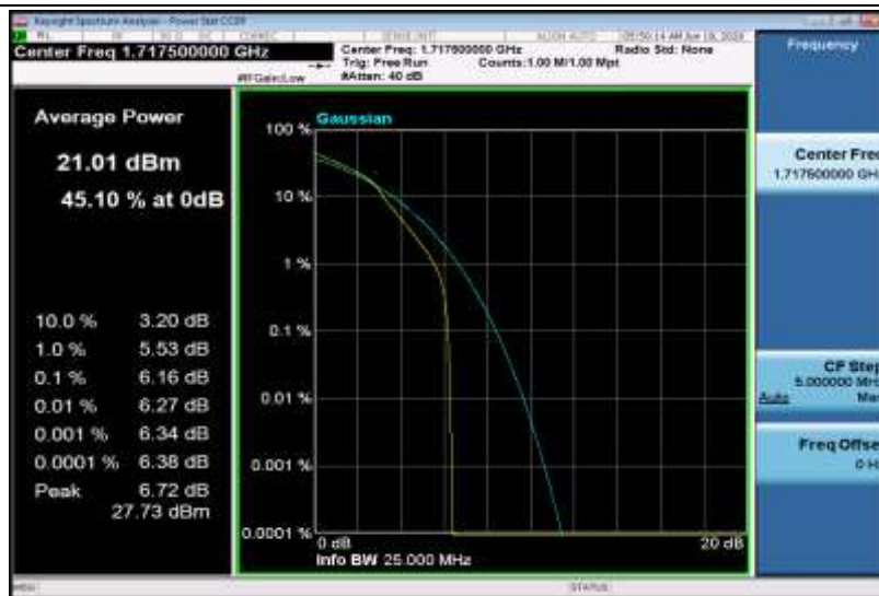
Band4-15MHz-16QAM-20025-75RB#0
