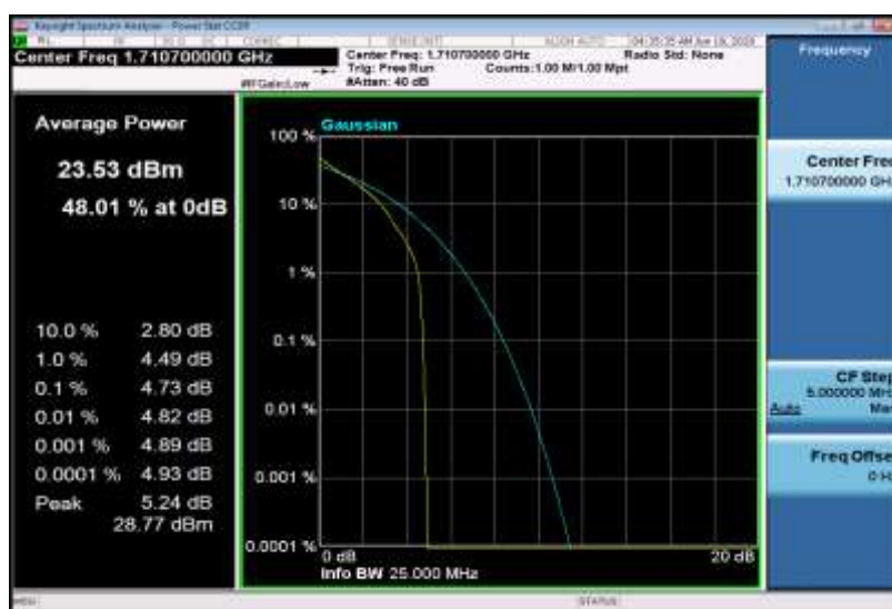
Band4-1.4MHz-QPSK-19957-6RB#0
