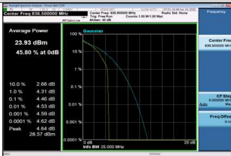
Band5-10MHz-QPSK-20525-50RB#0
