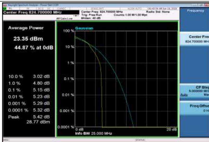
Band5-1.4MHz-16QAM-20407-6RB#0
