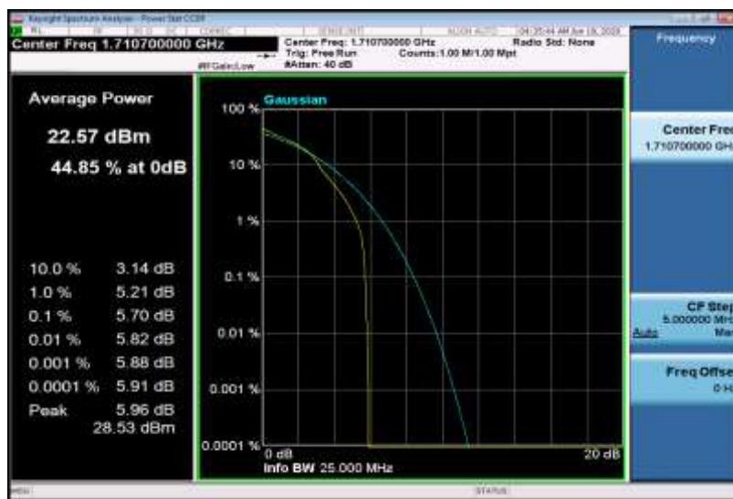
Band4-1.4MHz-16QAM-19957-6RB#0
