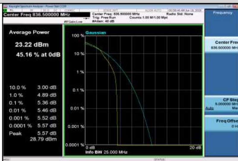
Band5-3MHz-16QAM-20525-15RB#0
