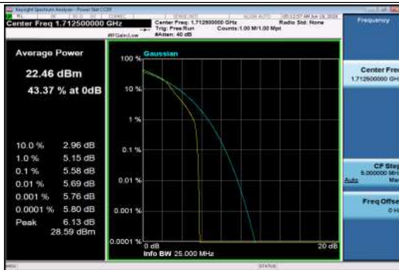
Band4-5MHz-16QAM-19975-25RB#0
