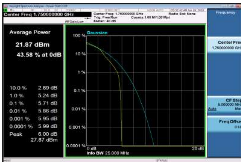
Band4-10MHz-16QAM-20350-50RB#0
