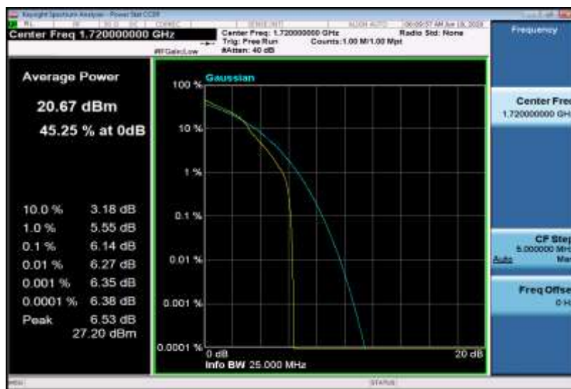
Band4-20MHz-16QAM-20050-100RB#0
