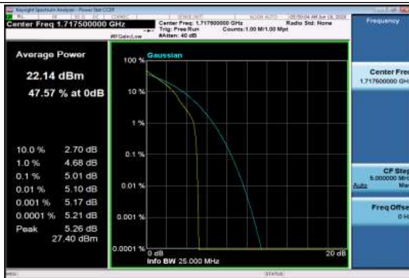
Band4-15MHz-QPSK-20025-75RB#0
