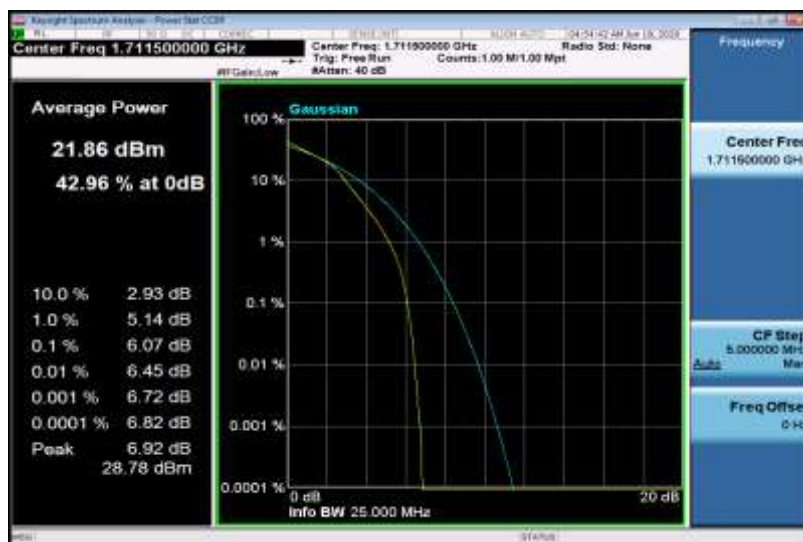
Band4-3MHz-16QAM-20175-1RB#0
