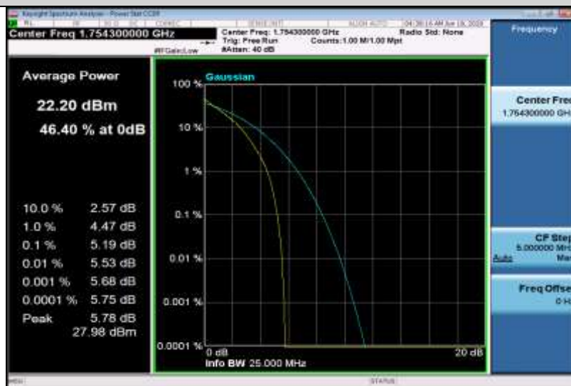
Band4-1.4MHz-16QAM-19957-1RB#0
