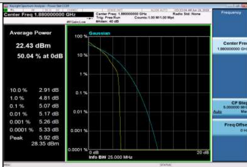
Band2-15MHz-QPSK-18900-75RB#0
