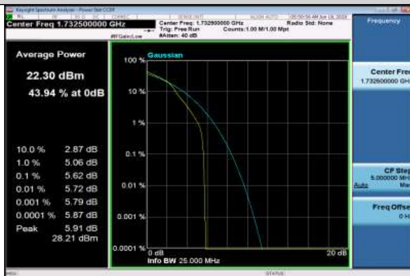
Band4-15MHz-16QAM-20175-75RB#0
