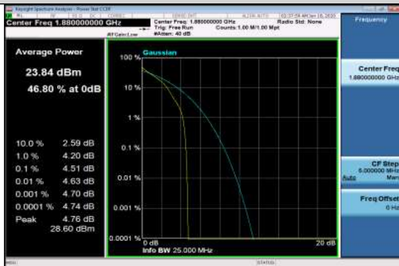
Band2-3MHz-QPSK-18900-15RB#0
