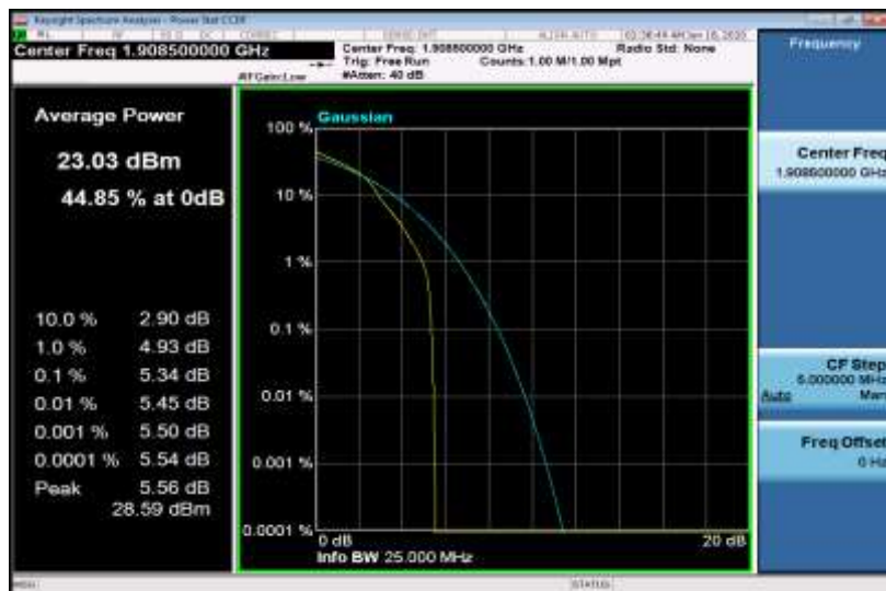
Band2-3MHz-16QAM-19185-15RB#0
