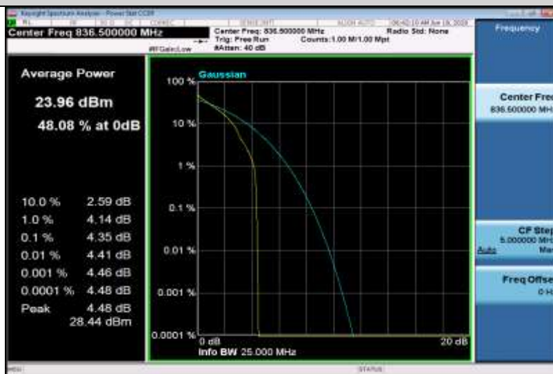
Band5-1.4MHz-QPSK-20525-6RB#0
