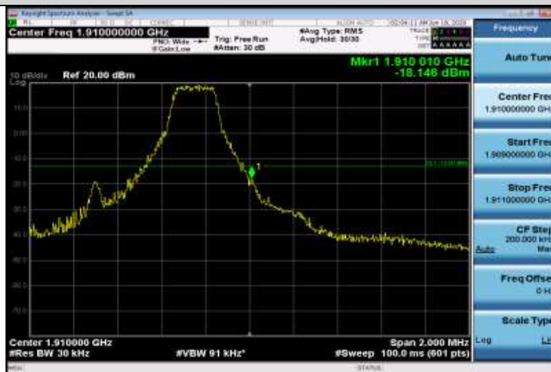
Band2-1.4MHz-16QAM-19193-1RB#5
