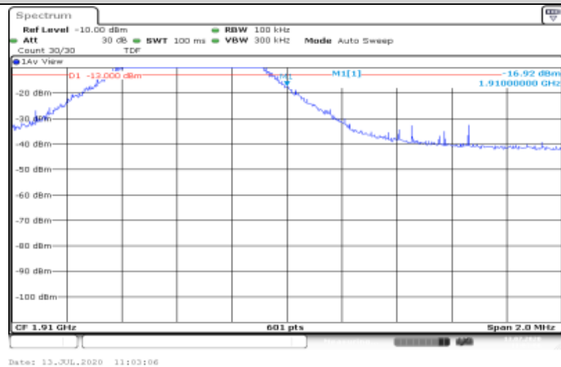
Band2-5MHz-16QAM-19175-1RB#24
