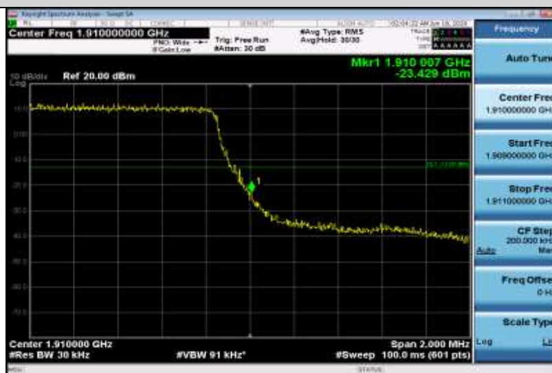
Band2-1.4MHz-QPSK-19193-6RB#0
