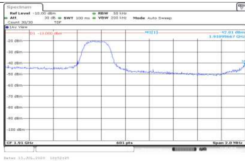
Band2-3MHz-16QAM-19185-1RB#14
