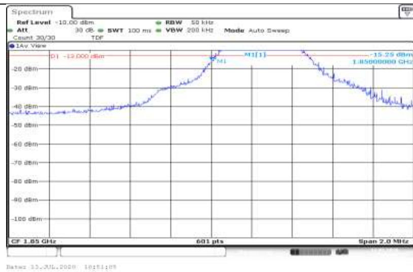
Band2-3MHz-16QAM-18615-1RB#14
