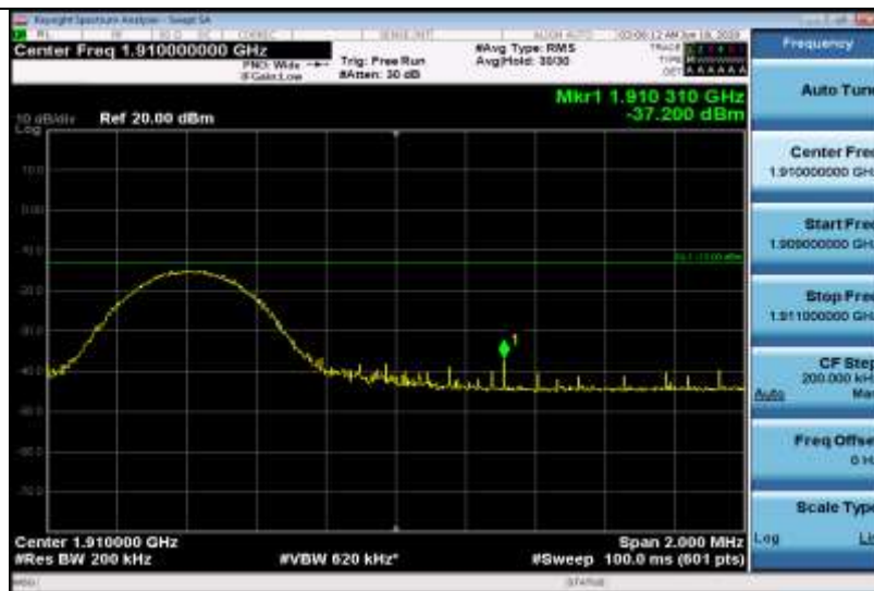
Band2-10MHz-16QAM-19150-1RB#49
