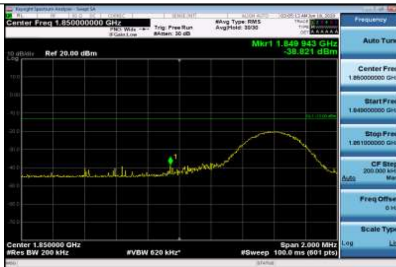
Band2-10MHz-16QAM-18650-1RB#0
