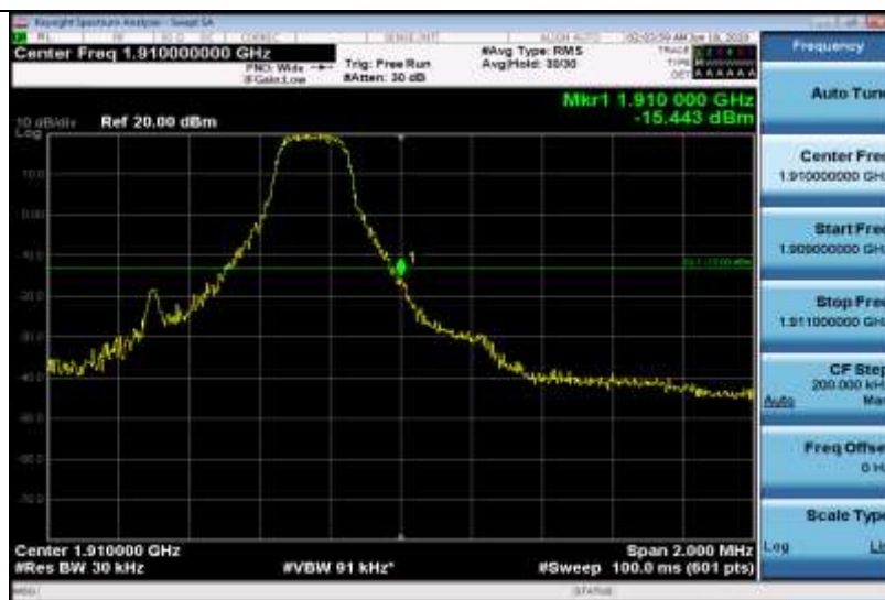
Band2-1.4MHz-QPSK-19193-1RB#0
