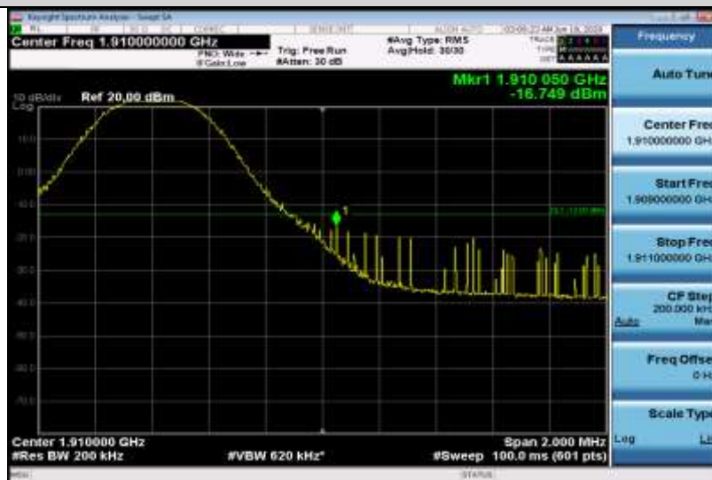
Band2-10MHz-QPSK-19150-1RB#49
