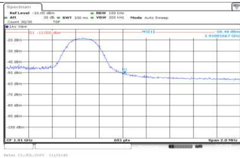
Band2-5MHz-16QAM-19175-1RB#24
