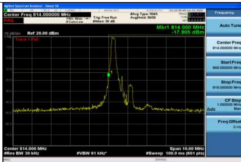
Band26-1.4MHz-16QAM-26697-1RB#5
