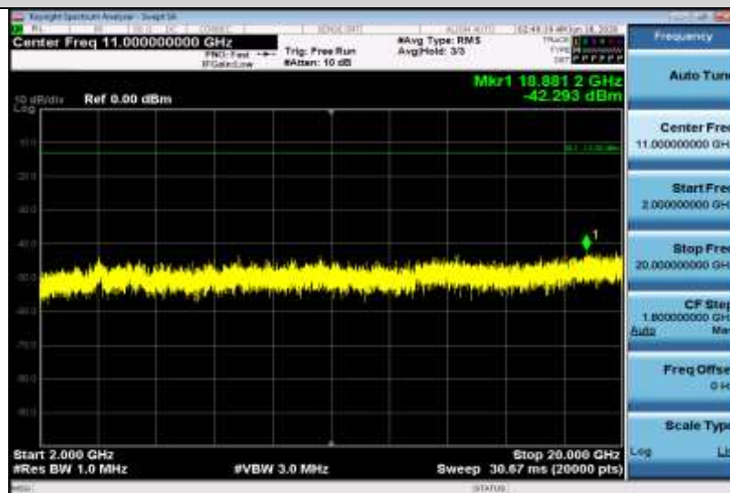
Band2-5MHz-QPSK-18625-1RB#0-Range3:2000~20000MHz
