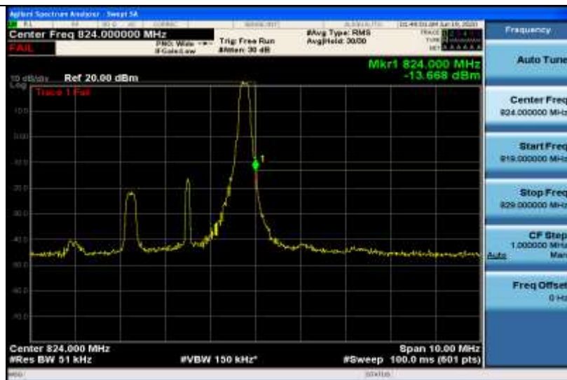
Band26-3MHz-QPSK-26775-1RB#0
