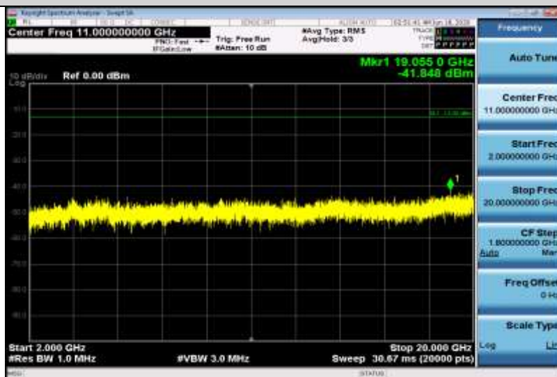
Band2-5MHz-16QAM-19175-1RB#0-Range3:2000~20000MHz
