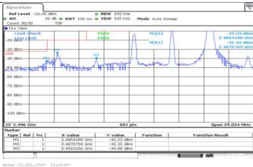
Band41-10MHz-16QAM-39700-1RB#0
