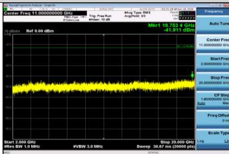
Band2-3MHz-16QAM-18615-1RB#0-Range3:2000~20000MHz
