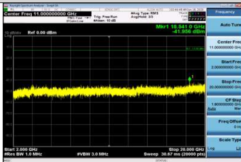
Band2-20MHz-QPSK-19100-1RB#0-Range3:2000~20000MHz
