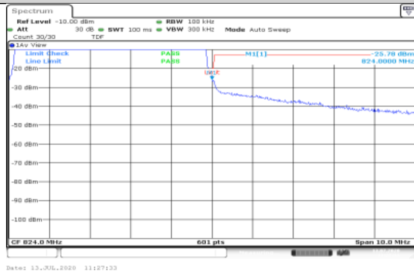
Band26-5MHz-16QAM-26765-25RB#0
