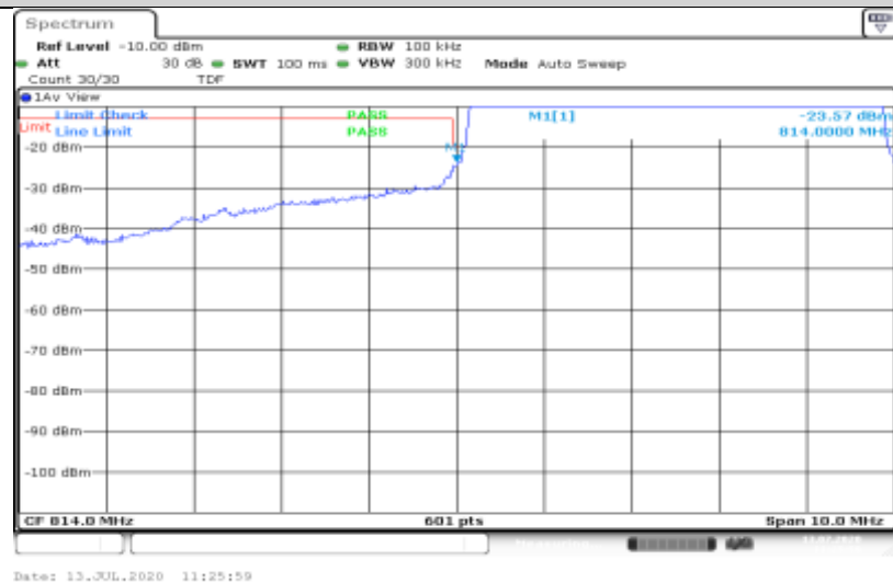
Band26-5MHz-QPSK-26715-25RB#0
