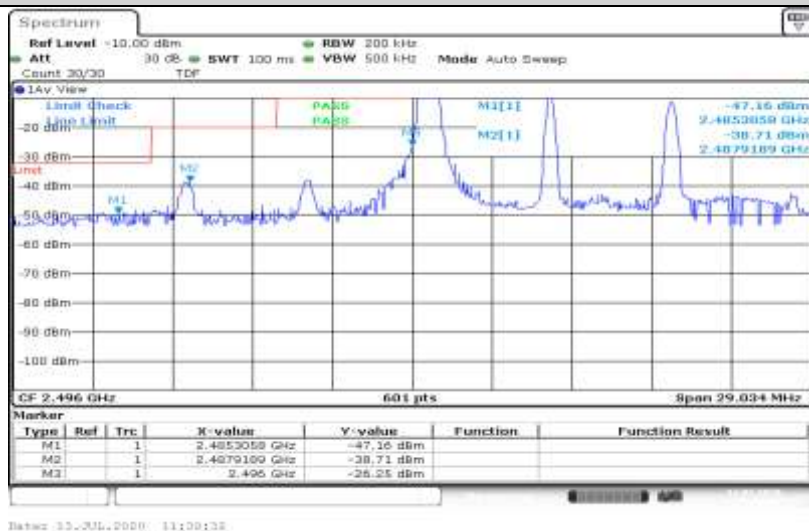
Band41-10MHz-16QAM-39700-50RB#0
