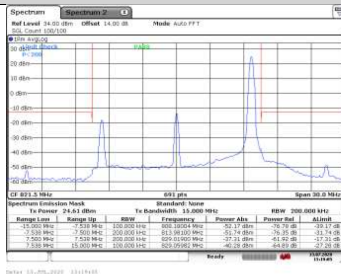
Band26-15MHz-16QAM-26765-1RB#74
