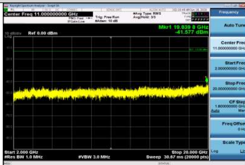
Band2-1.4MHz-16QAM-19193-1RB#0-Range3:2000~20000MHz
