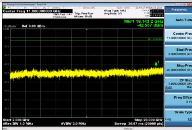
Band2-20MHz-16QAM-18900-1RB#0-Range3:2000~20000MHz
