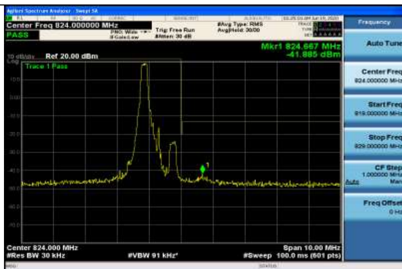
Band26-1.4MHz-16QAM-26783-1RB#5
