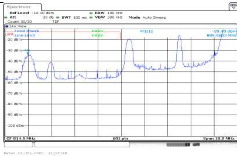
Band26-5MHz-16QAM-26715-1RB#0
