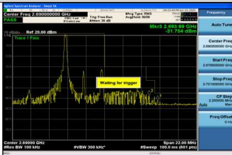
Band41-5MHz-16QAM-41565-25RB#0
