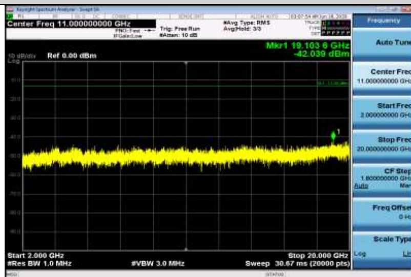
Band2-10MHz-16QAM-18650-1RB#0-Range3:2000~20000MHz
