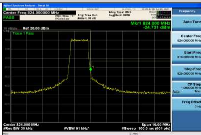
Band26-1.4MHz-16QAM-26783-6RB#0
