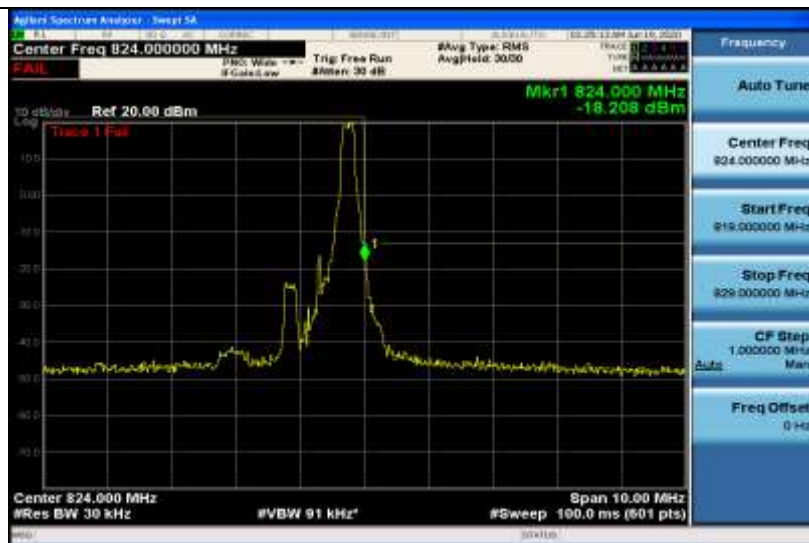
Band26-1.4MHz-QPSK-26783-1RB#0
