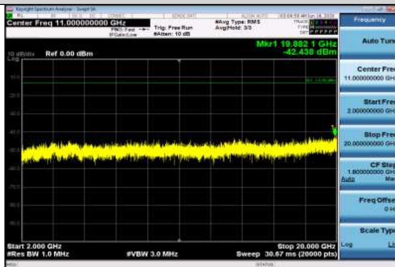
Band2-10MHz-16QAM-19150-1RB#0-Range3:2000~20000MHz
