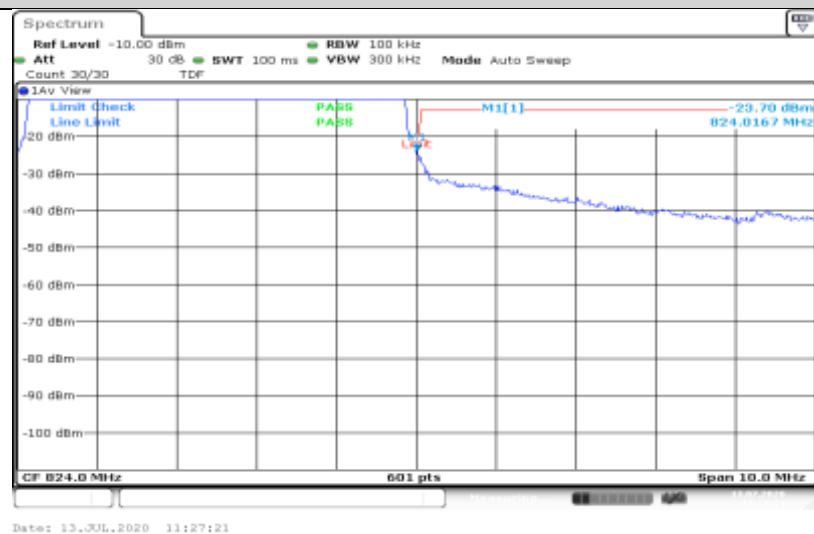
Band26-5MHz-QPSK-26765-25RB#0
