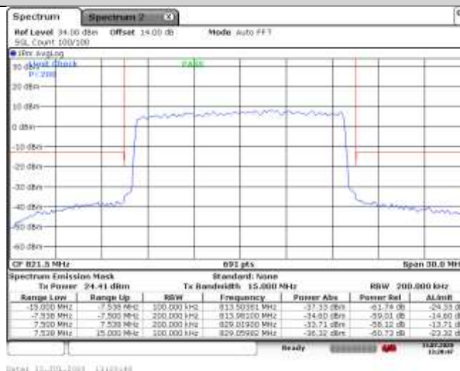
Band26-15MHz-16QAM-26765-75RB#0
