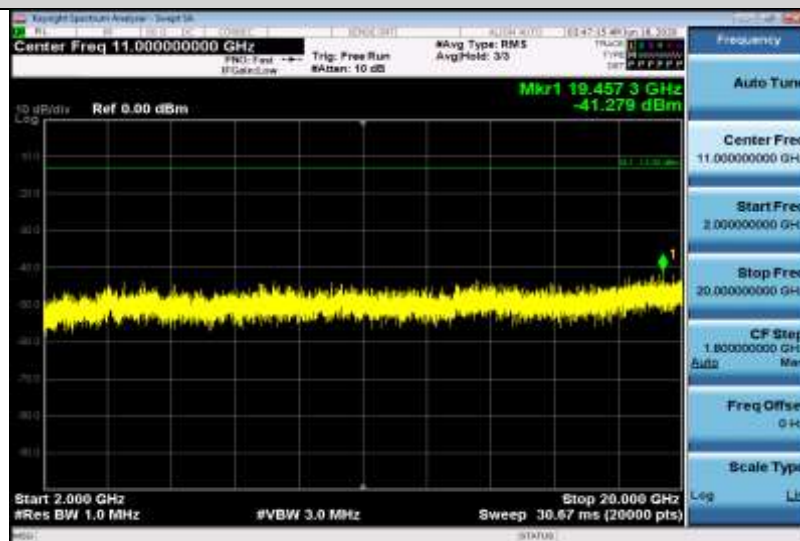
Band2-20MHz-16QAM-19100-1RB#0-Range3:2000~20000MHz
