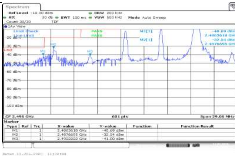
Band41-10MHz-QPSK-39700-1RB#0
