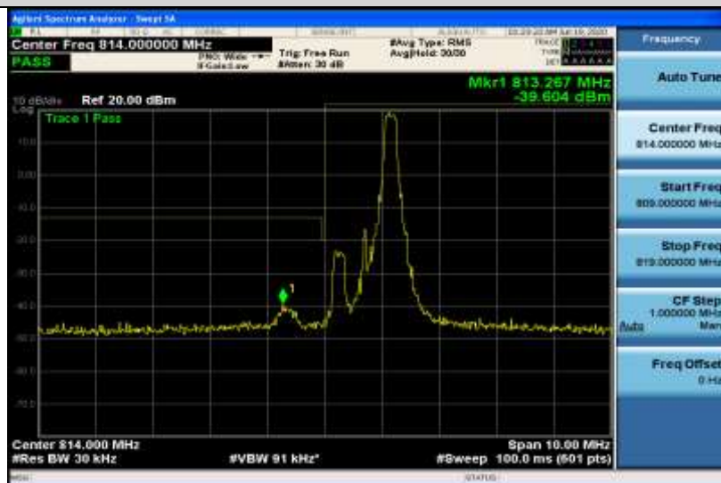
Band26-1.4MHz-16QAM-26697-6RB#0
