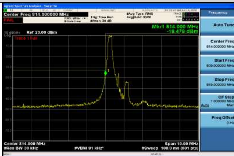
Band26-1.4MHz-QPSK-26697-6RB#0
