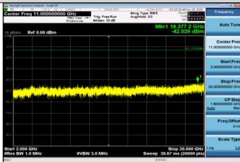
Band2-15MHz-QPSK-18675-1RB#0-Range3:2000~20000MHz
