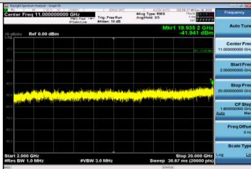
Band2-5MHz-QPSK-18900-1RB#0-Range3:2000~20000MHz
