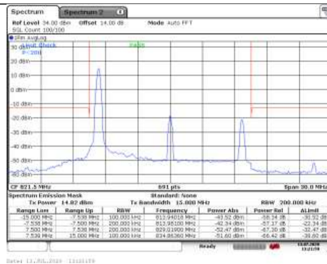
Band26-15MHz-QPSK-26765-1RB#74
