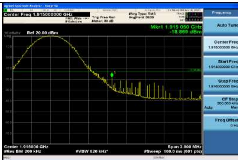
Band25-10MHz-16QAM-26640-1RB#0
