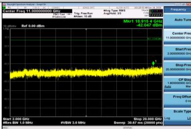
Band2-15MHz-16QAM-18675-1RB#0-Range3:2000~20000MHz
