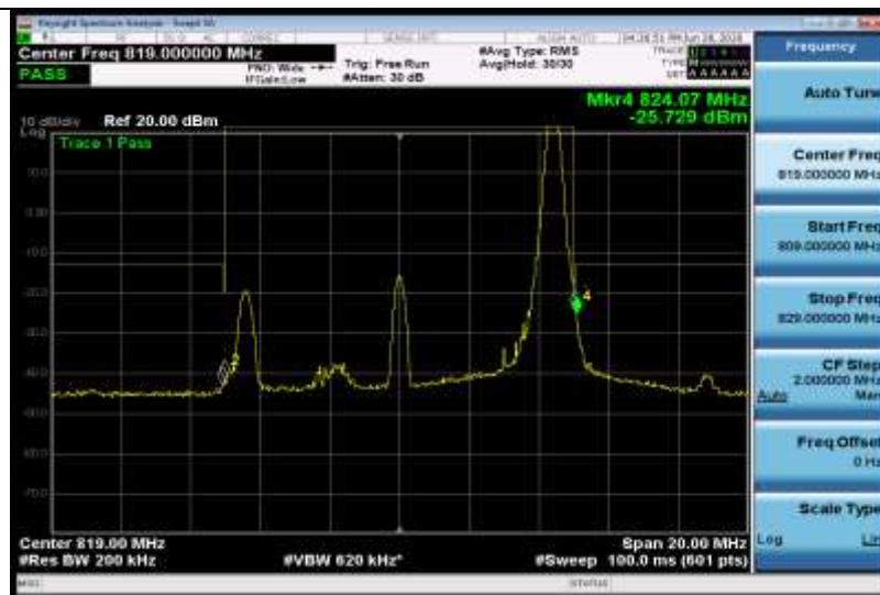
Band26-10MHz-QPSK-26740-1RB#0
