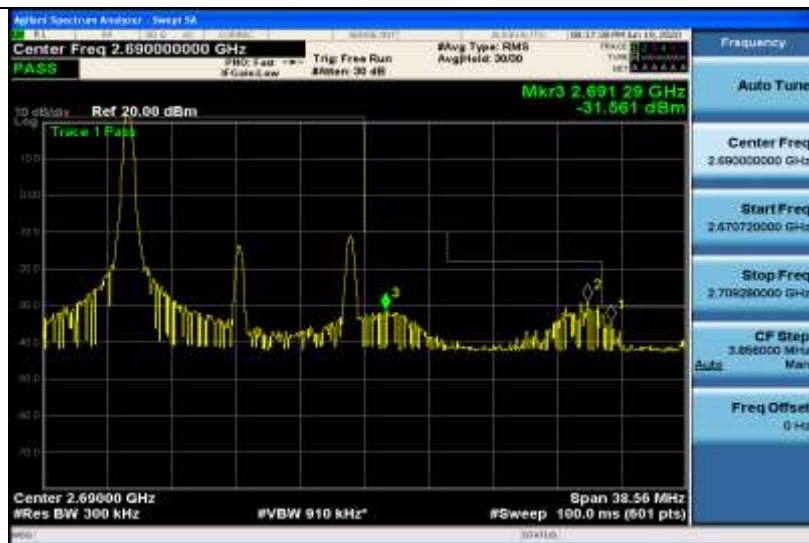
Band41-15MHz-QPSK-41515-1RB#74
