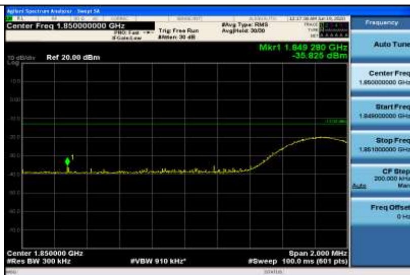
Band25-15MHz-16QAM-26115-1RB#0
