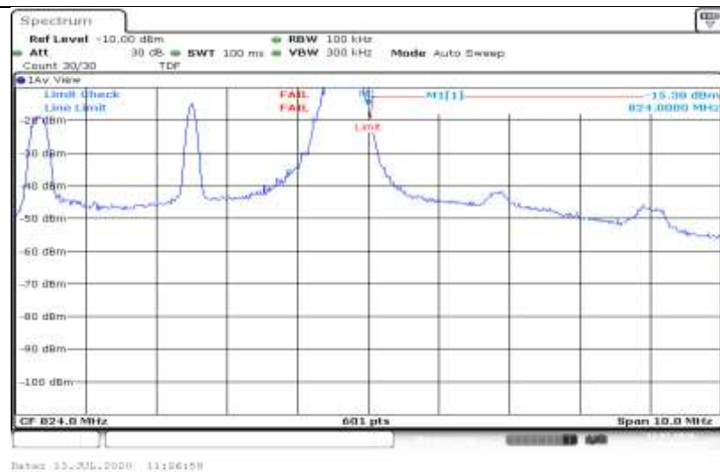
Band26-5MHz-QPSK-26765-1RB#0
