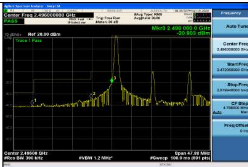
Band41-20MHz-QPSK-39750-1RB#99
