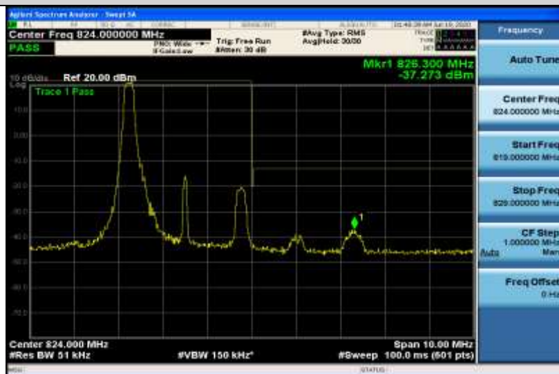
Band26-3MHz-QPSK-26775-15RB#0
