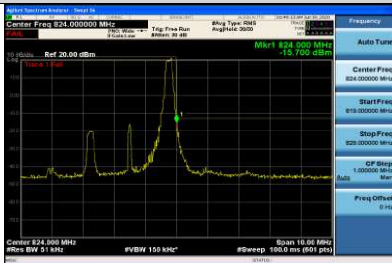
Band26-3MHz-16QAM-26775-15RB#0
