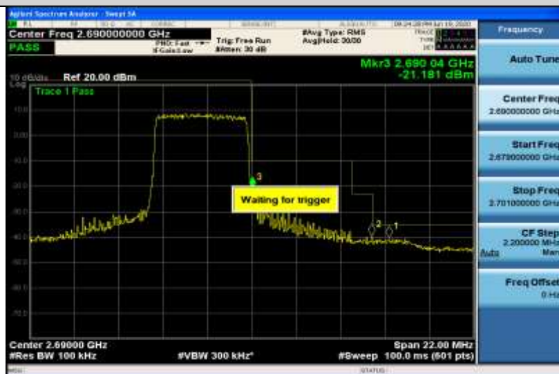
Band41-5MHz-QPSK-41565-25RB#0
