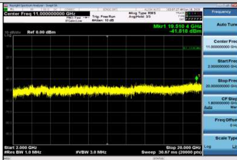
Band2-10MHz-QPSK-18650-1RB#0-Range3:2000~20000MHz
