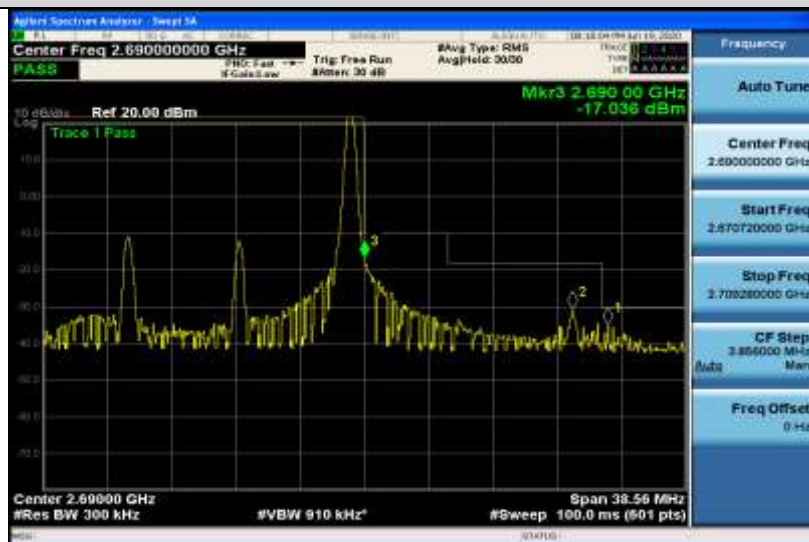
Band41-15MHz-QPSK-41515-75RB#0
