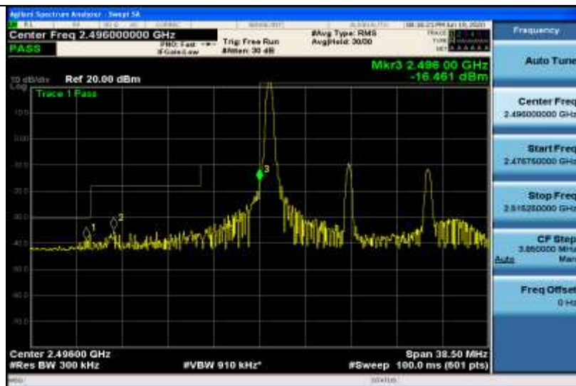
Band41-15MHz-16QAM-39725-1RB#74
