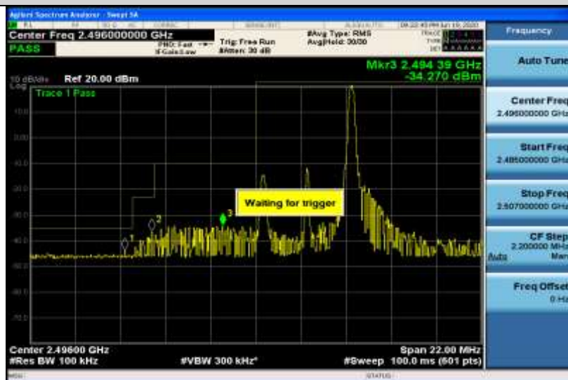
Band41-5MHz-16QAM-39675-25RB#0
