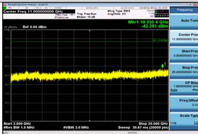
Band2-10MHz-16QAM-18900-1RB#0-Range3:2000~20000MHz
