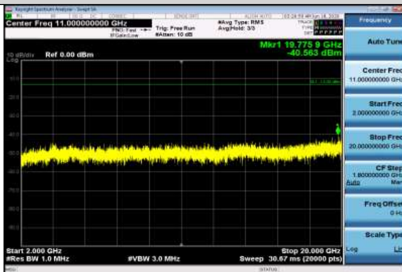
Band2-15MHz-16QAM-18900-1RB#0-Range3:2000~20000MHz
