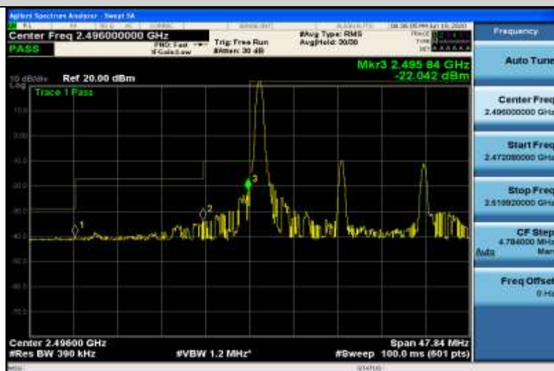
Band41-20MHz-16QAM-39750-100RB#0
