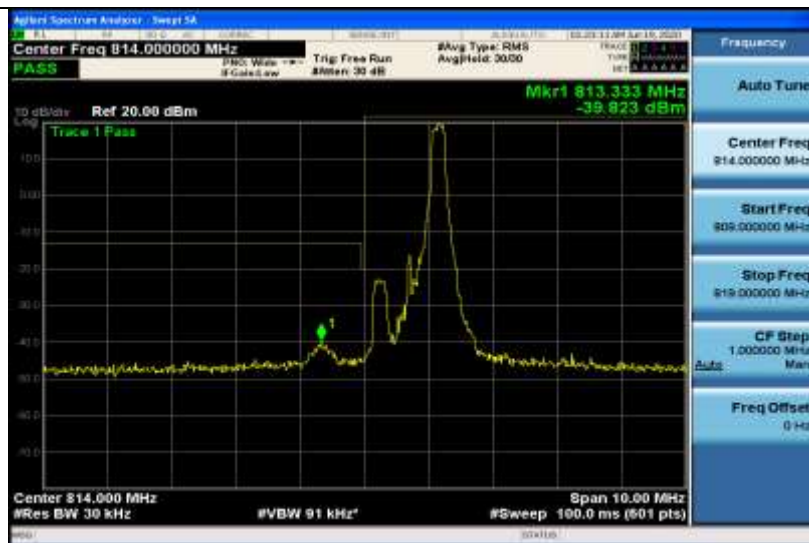
Band26-1.4MHz-QPSK-26697-1RB#0
