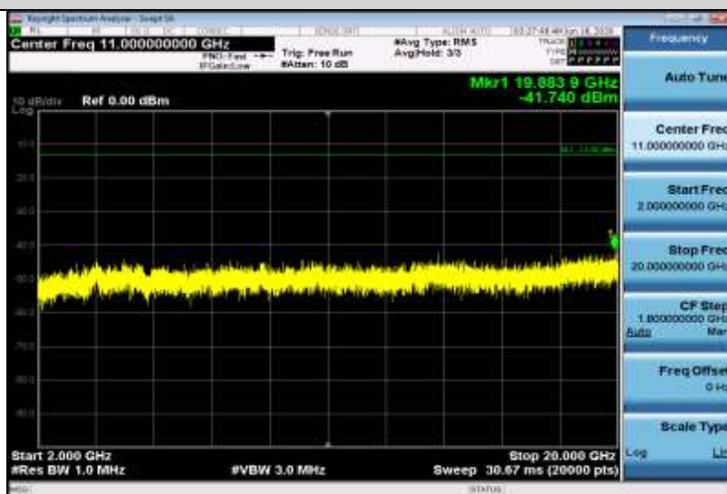
Band2-15MHz-16QAM-19125-1RB#0-Range3:2000~20000MHz
