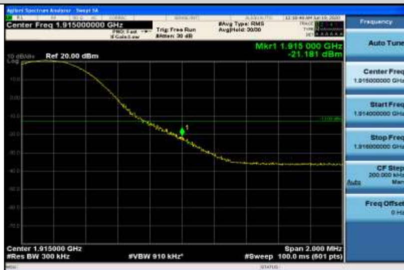
Band25-15MHz-QPSK-26615-75RB#0
