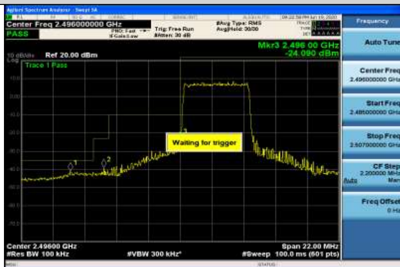
Band41-5MHz-QPSK-39675-25RB#0
