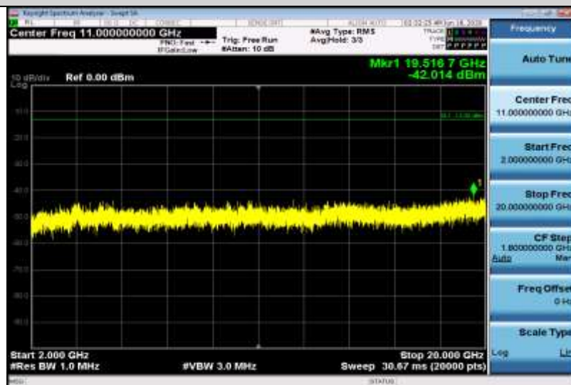
Band2-3MHz-16QAM-18900-1RB#0-Range3:2000~20000MHz
