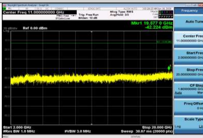
Band2-15MHz-QPSK-18900-1RB#0-Range3:2000~20000MHz
