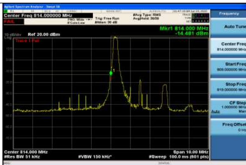
Band26-3MHz-QPSK-26705-1RB#14
