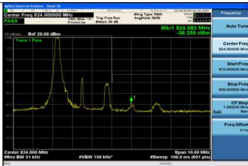
Band26-3MHz-16QAM-26775-1RB#14
