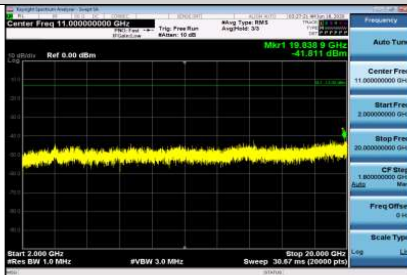
Band2-15MHz-QPSK-19125-1RB#0-Range3:2000~20000MHz
