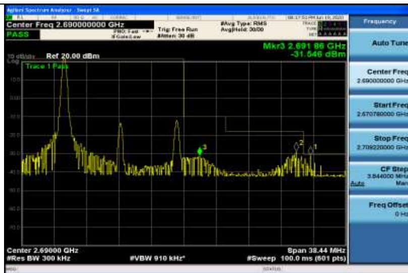
Band41-15MHz-16QAM-41515-1RB#74
