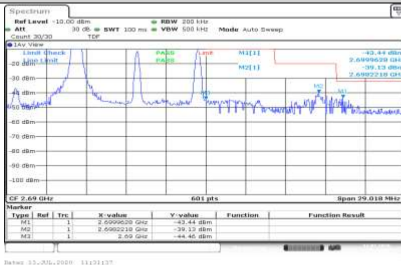
Band41-10MHz-QPSK-41540-50RB#0
