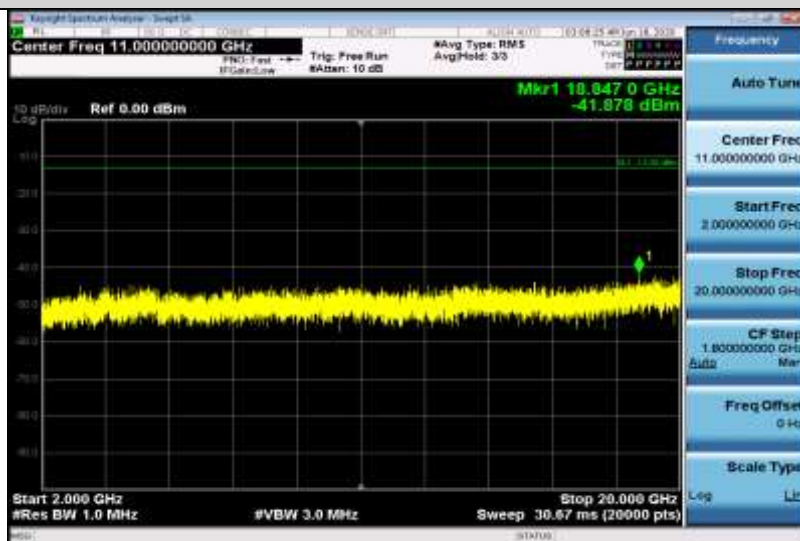
Band2-10MHz-QPSK-18900-1RB#0-Range3:2000~20000MHz
