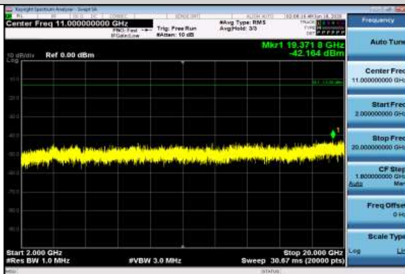
Band2-1.4MHz-QPSK-18900-1RB#0-Range3:2000~20000MHz
