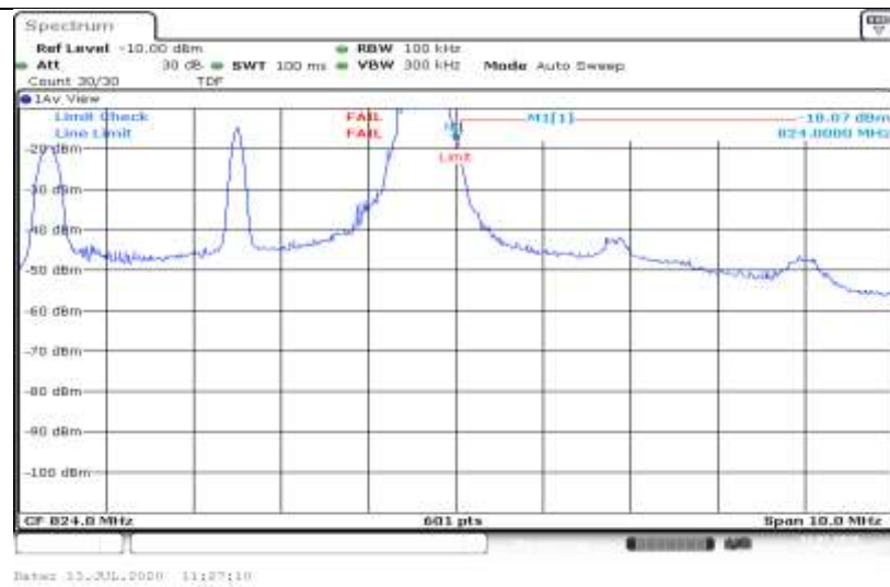
Band26-5MHz-16QAM-26765-1RB#0
