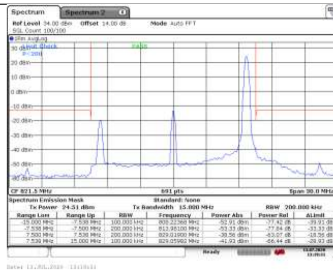
Band26-15MHz-16QAM-26765-1RB#0
