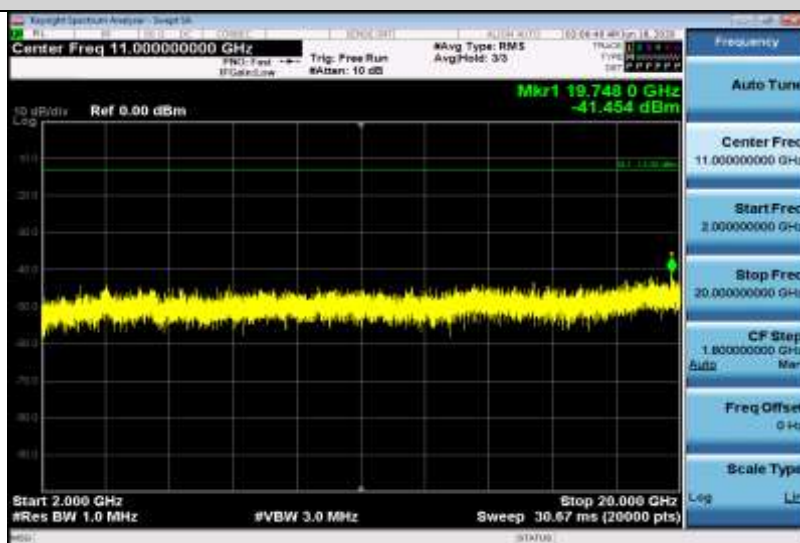
Band2-1.4MHz-16QAM-18607-1RB#0-Range3:2000~20000MHz
