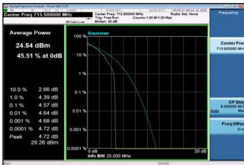
Band12-5MHz-QPSK-23155-25RB#0
