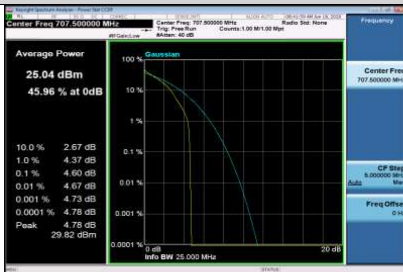
Band12-3MHz-QPSK-23095-15RB#0
