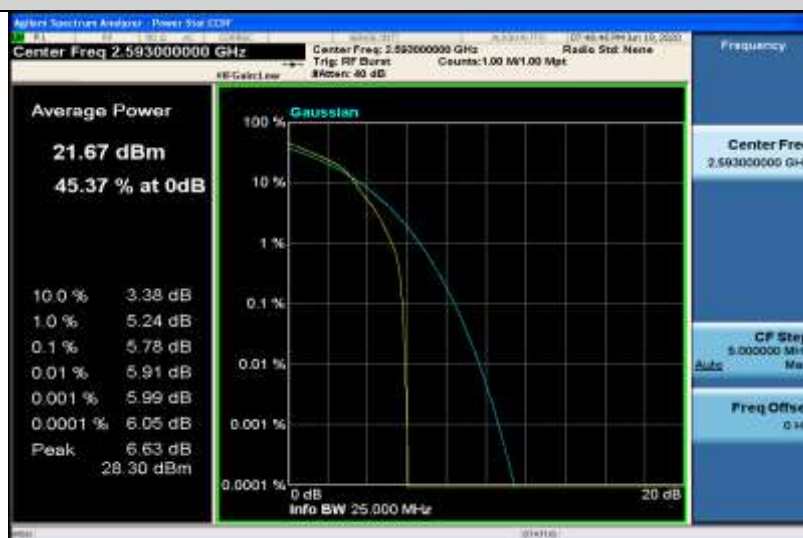
Band41-5MHz-16QAM-40620-25RB#0
