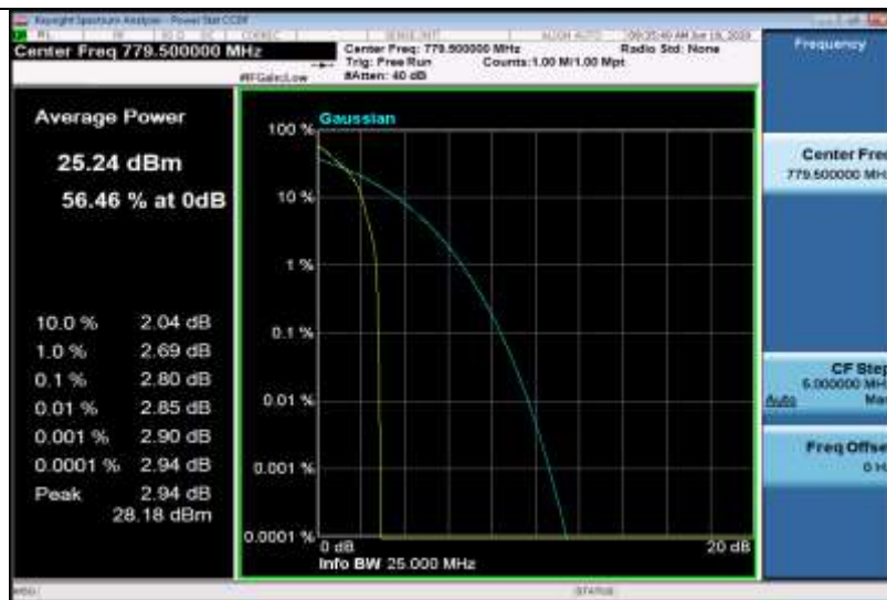
Band13-5MHz-QPSK-23205-25RB#0
