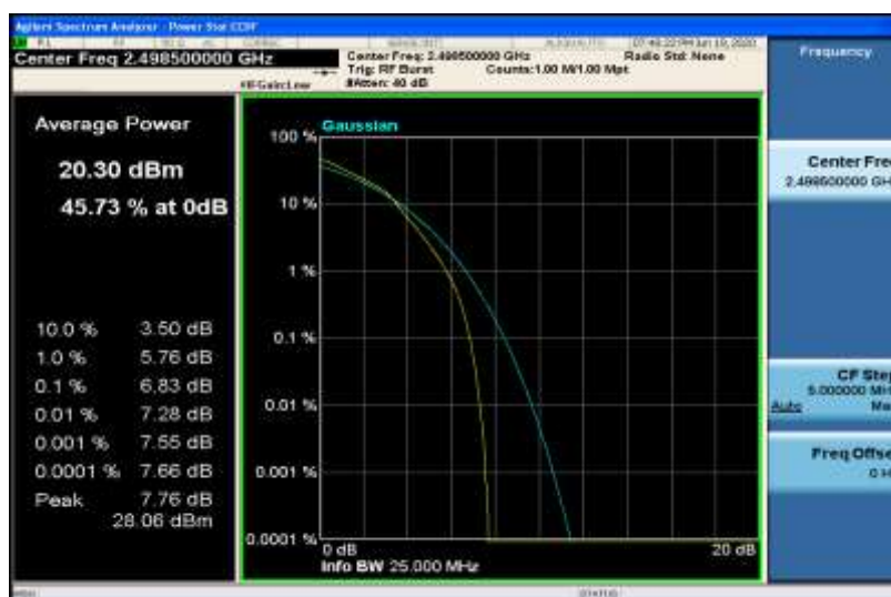
Band41-5MHz-16QAM-40620-1RB#0
