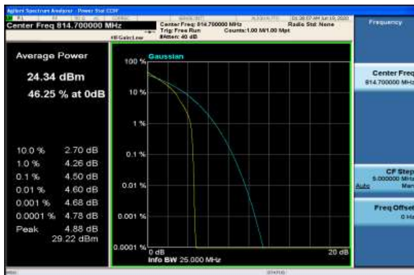
Band26-1.4MHz-QPSK-26697-6RB#0
