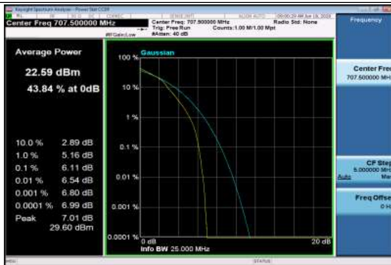
Band12-5MHz-16QAM-23155-1RB#0
