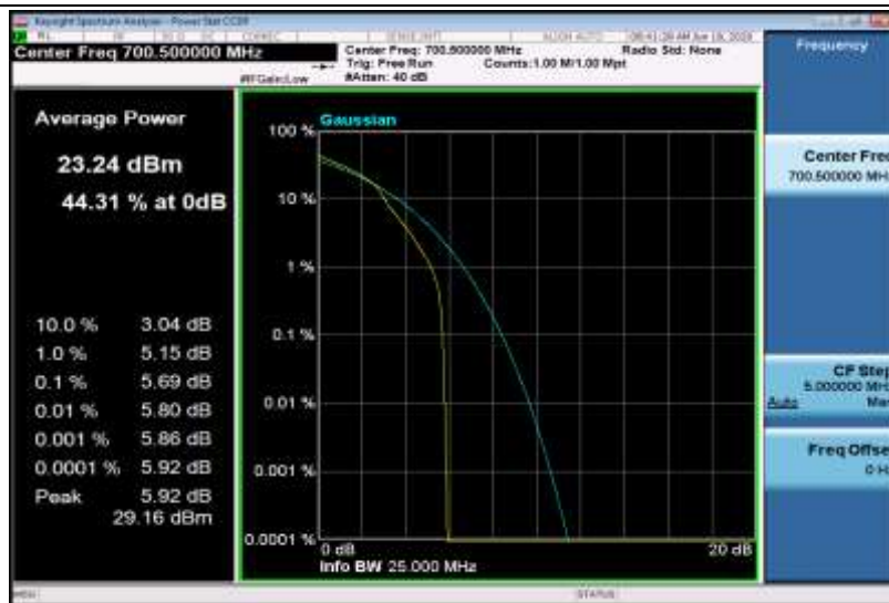
Band12-3MHz-16QAM-23025-15RB#0
