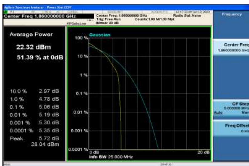
Band25-20MHz-QPSK-26140-100RB#0
