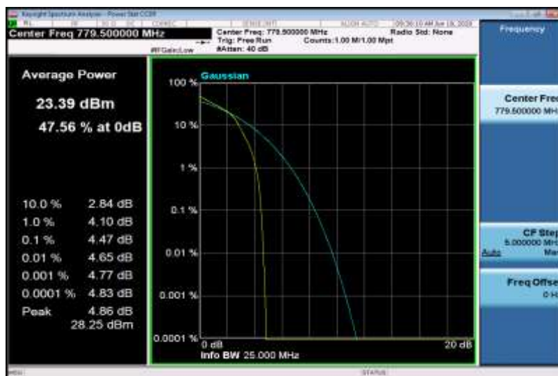
Band13-5MHz-16QAM-23230-1RB#0
