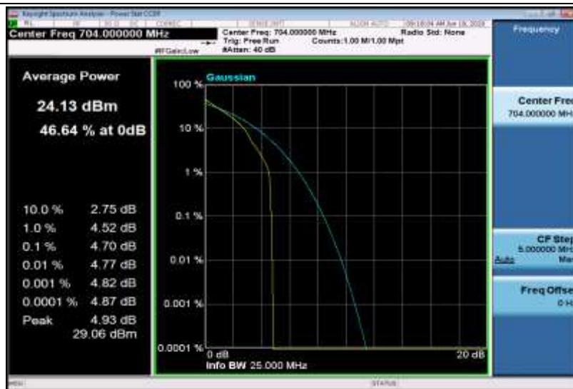
Band12-10MHz-QPSK-23060-50RB#0
