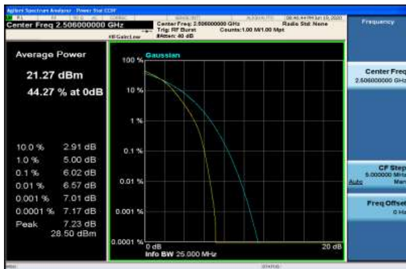
Band41-20MHz-16QAM-40620-1RB#0
