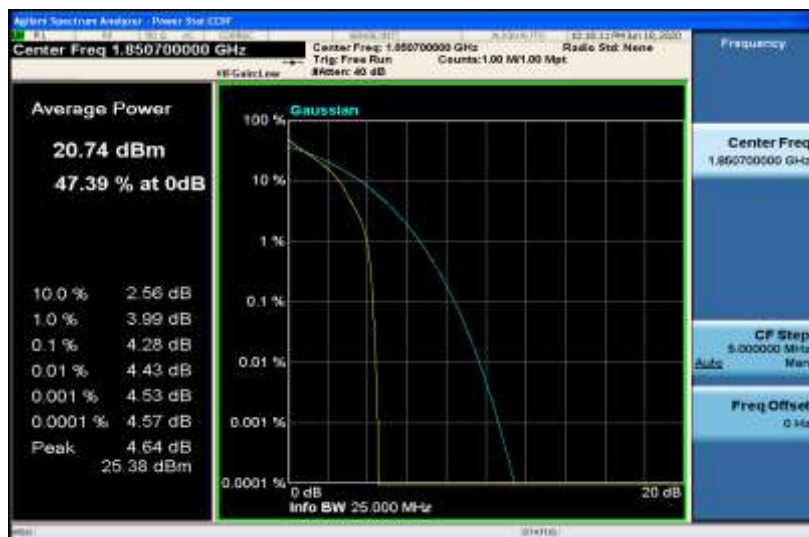
Band25-1.4MHz-QPSK-26047-6RB#0
