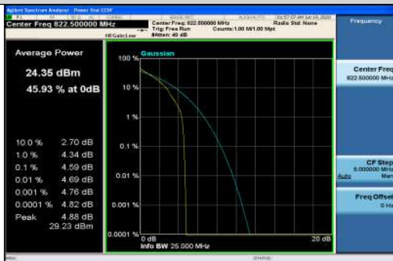
Band26-3MHz-QPSK-26775-15RB#0
