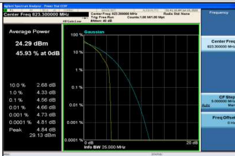
Band26-1.4MHz-QPSK-26783-6RB#0
