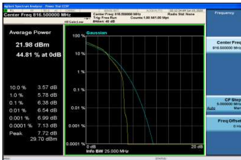
Band26-5MHz-16QAM-26715-25RB#0
