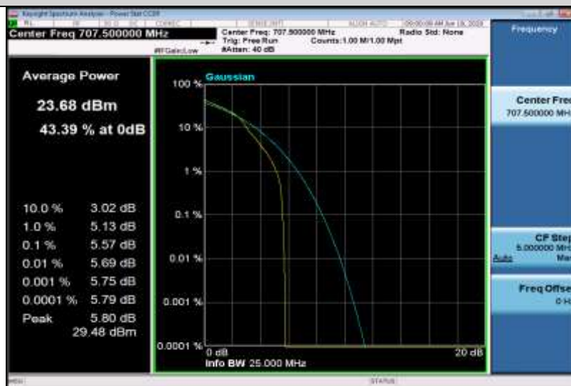
Band12-5MHz-16QAM-23095-25RB#0
