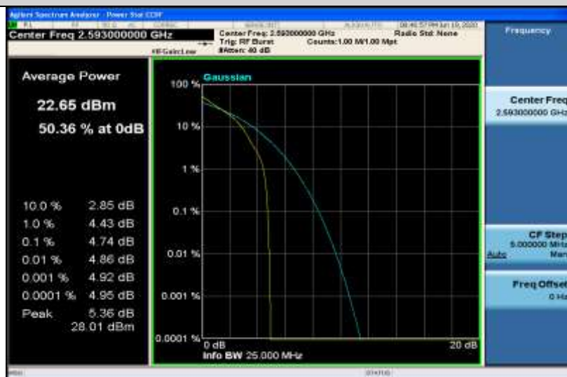
Band41-20MHz-QPSK-40620-100RB#0
