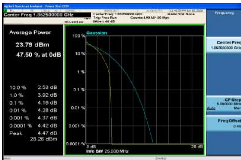
Band25-5MHz-QPSK-26065-25RB#0
