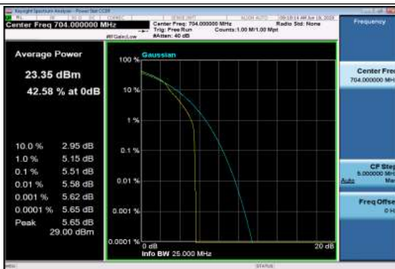
Band12-10MHz-16QAM-23060-50RB#0
