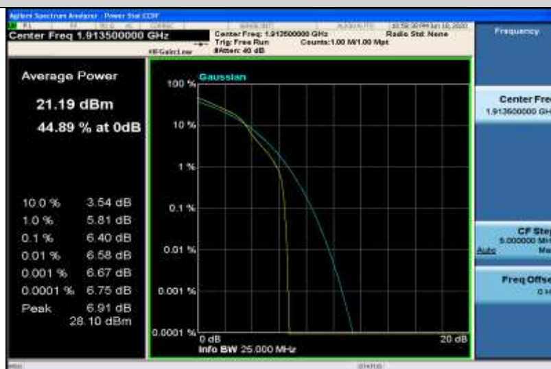
Band25-3MHz-16QAM-26675-15RB#0
