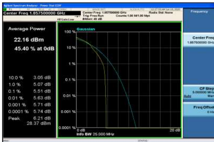
Band25-15MHz-16QAM-26115-75RB#0
