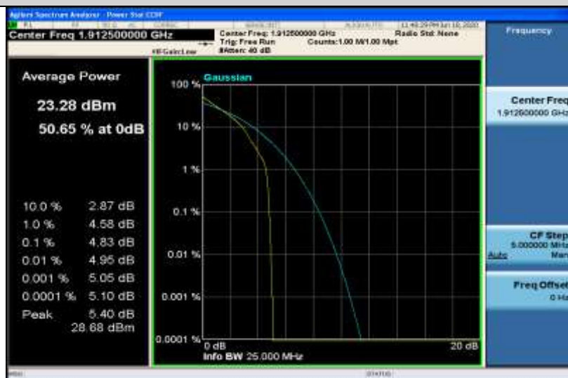
Band25-5MHz-QPSK-26665-25RB#0
