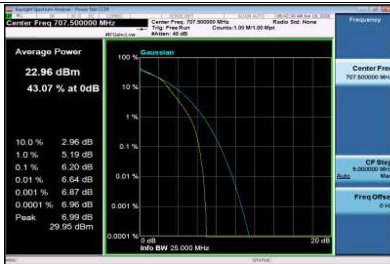
Band12-3MHz-16QAM-23165-1RB#0
