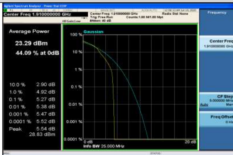
Band25-10MHz-16QAM-26640-50RB#0
