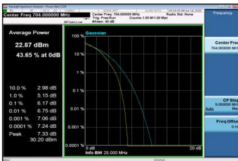
Band12-10MHz-16QAM-23095-1RB#0
