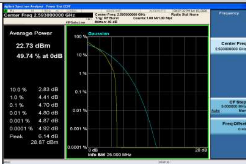
Band41-10MHz-QPSK-40620-50RB#0
