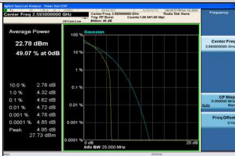
Band41-15MHz-QPSK-40620-75RB#0
