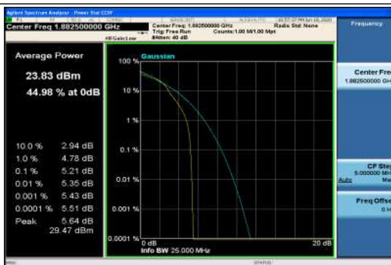
Band25-3MHz-16QAM-26365-15RB#0
