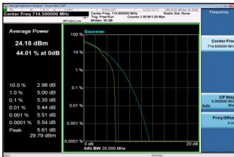
Band12-3MHz-16QAM-23165-15RB#0
