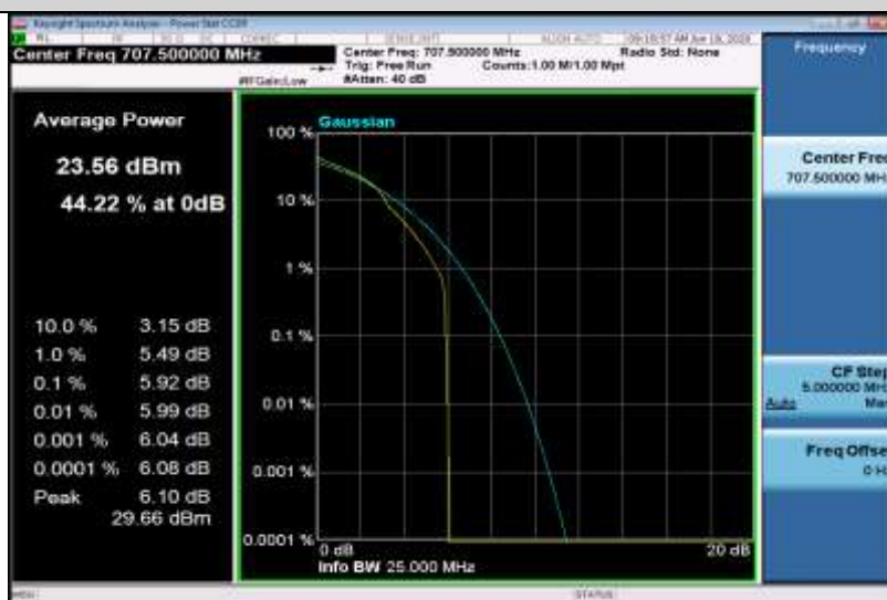
Band12-10MHz-16QAM-23095-50RB#0
