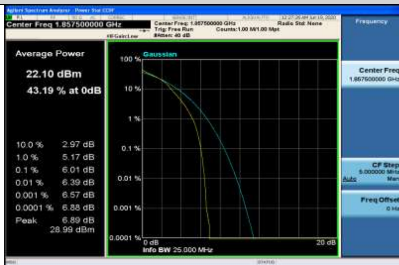
Band25-15MHz-16QAM-26365-1RB#0
