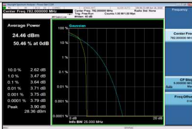
Band13-5MHz-16QAM-23230-25RB#0
