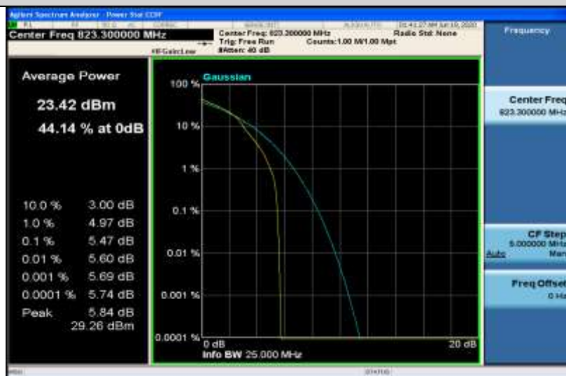
Band26-1.4MHz-16QAM-26783-6RB#0
