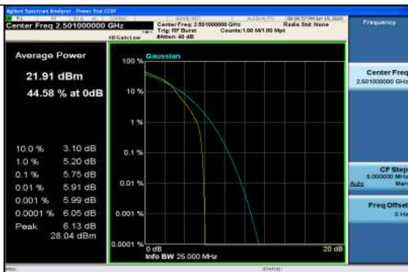
Band41-10MHz-16QAM-39700-50RB#0
