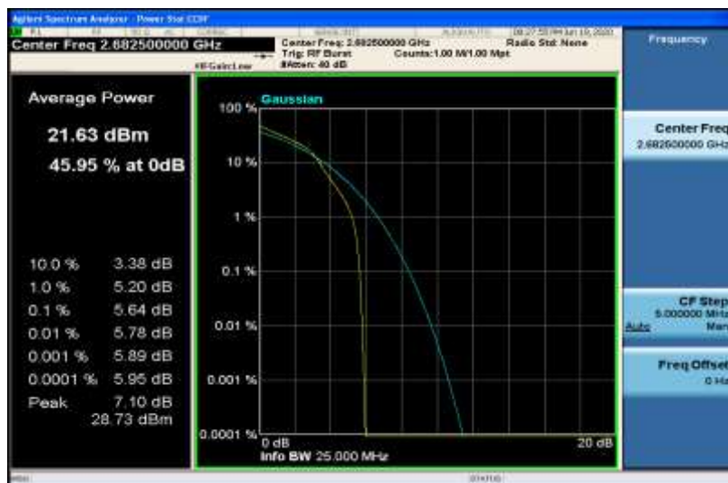
Band41-15MHz-16QAM-41515-75RB#0
