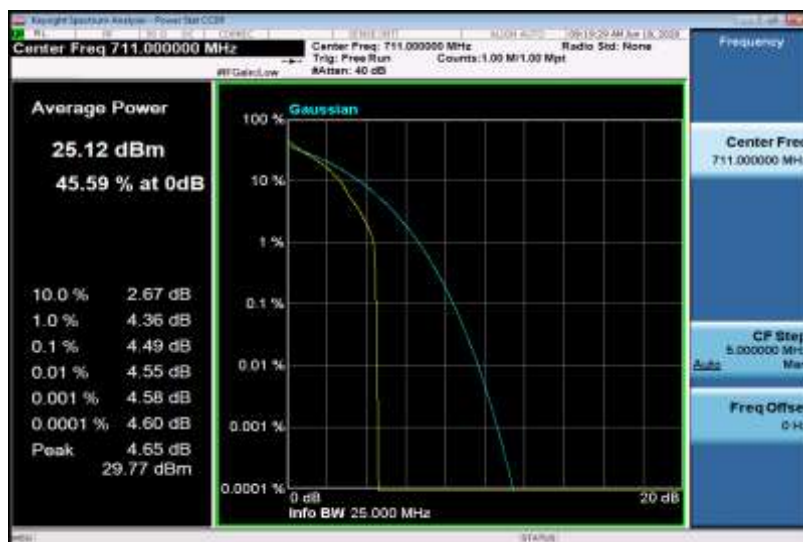
Band12-10MHz-QPSK-23130-50RB#0
