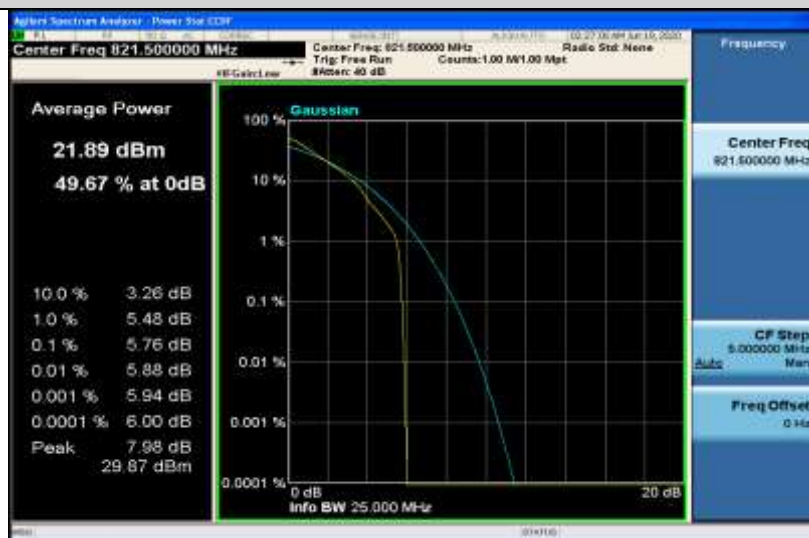
Band26-15MHz-QPSK-26765-75RB#0
