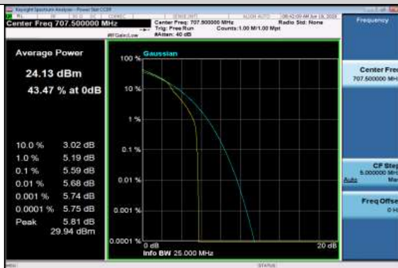
Band12-3MHz-16QAM-23095-15RB#0
