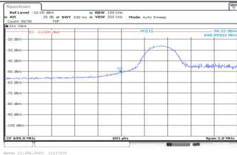
Band12-5MHz-16QAM-23035-25RB#0
