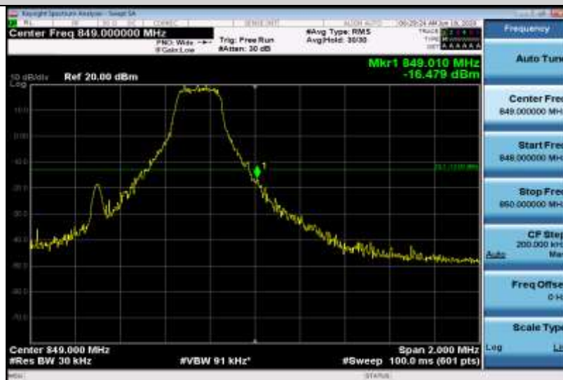
Band5-1.4MHz-16QAM-20643-6RB#0
