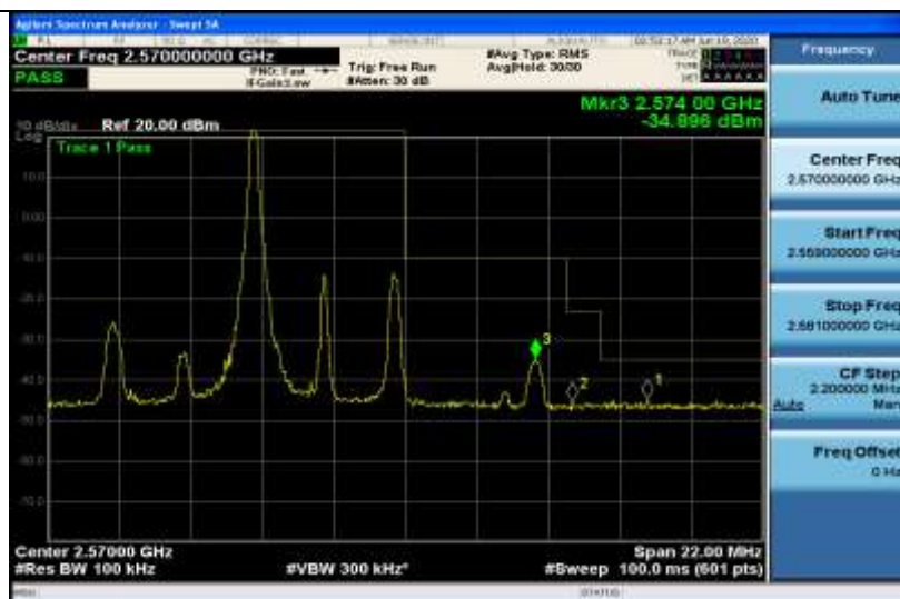
Band7-5MHz-QPSK-21425-1RB#24
