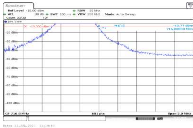
Band12-3MHz-QPSK-23165-1RB#0
