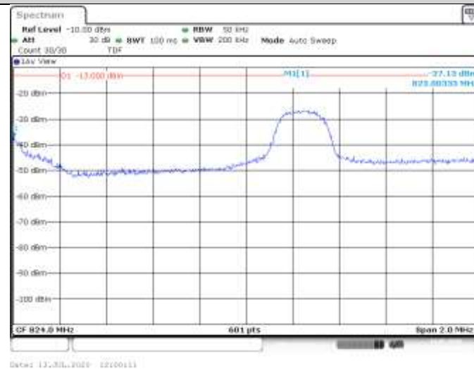
Band5-3MHz-QPSK-20415-15RB#0
