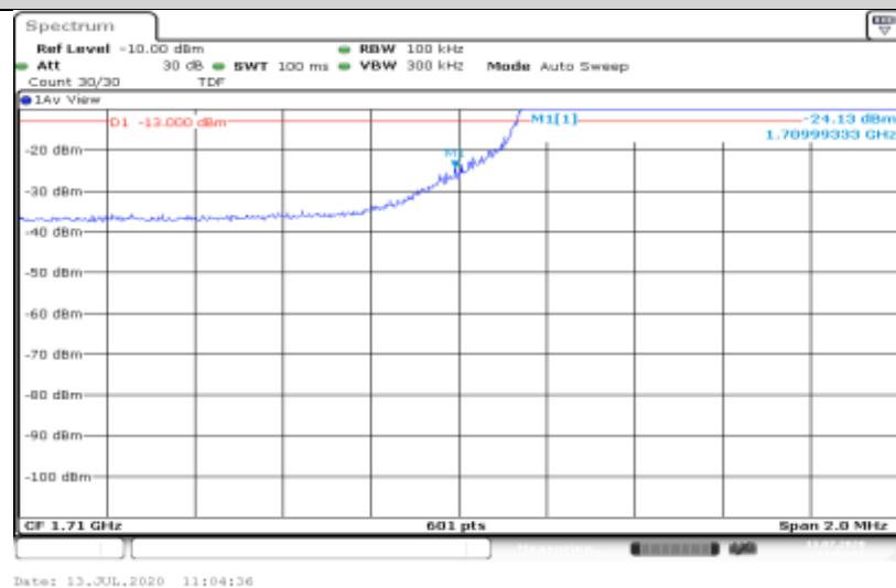
Band4-5MHz-QPSK-19975-25RB#0
