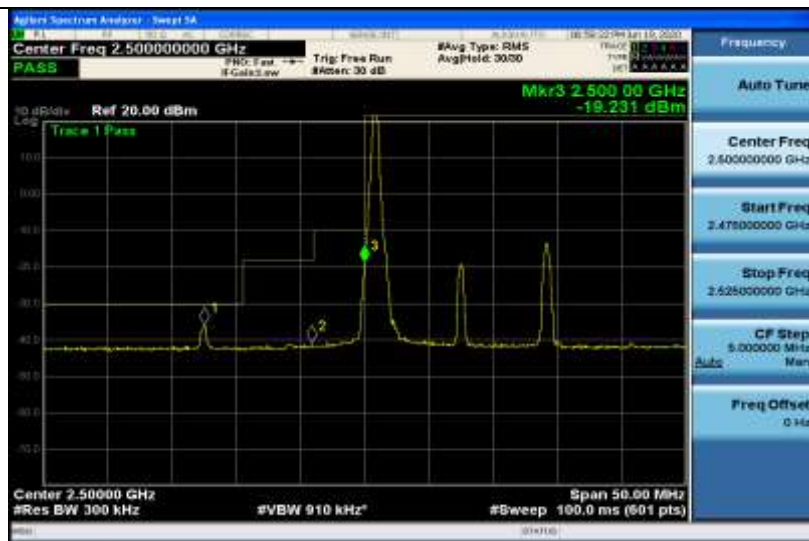
Band7-15MHz-QPSK-20825-1RB#74
