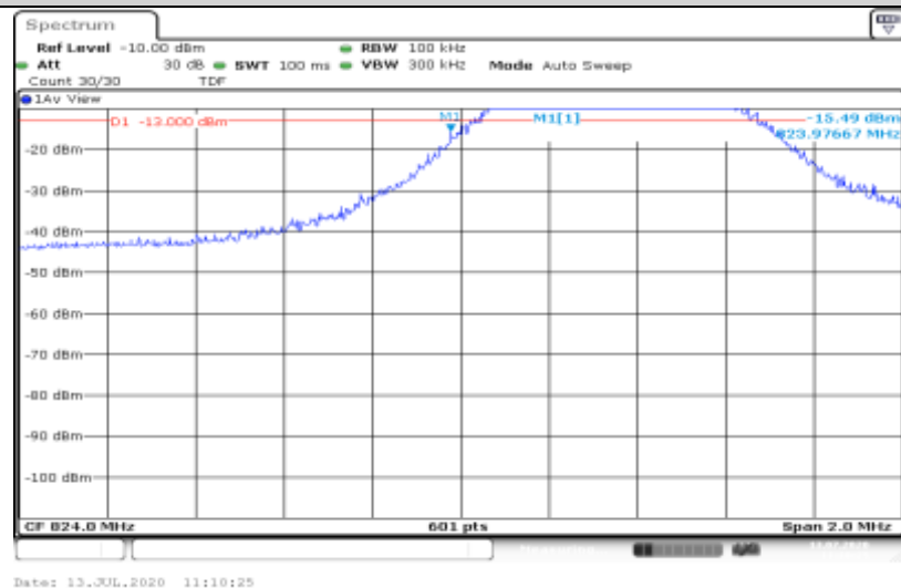
Band5-5MHz-QPSK-20425-1RB#0
