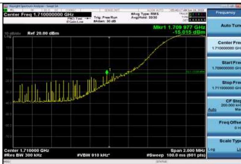
Band4-15MHz-QPSK-20025-1RB#74
