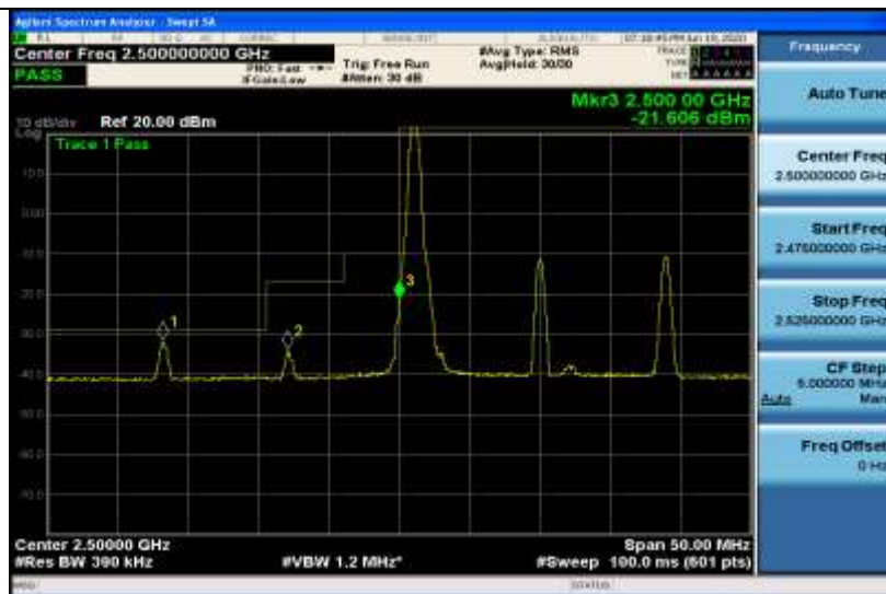
Band7-20MHz-16QAM-20850-1RB#99
