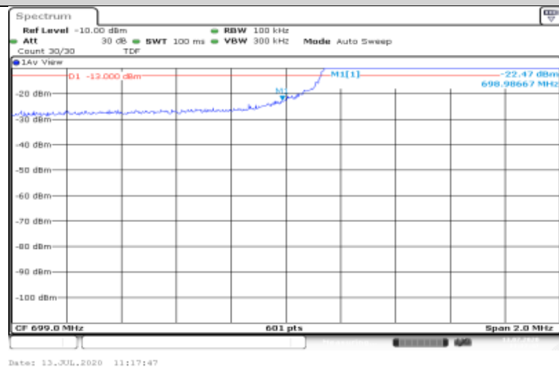
Band12-5MHz-QPSK-23035-25RB#0
