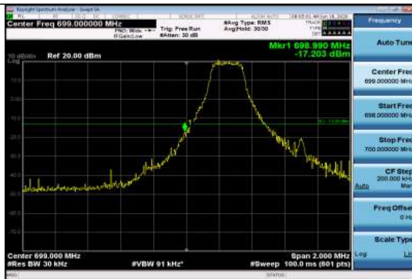
Band12-1.4MHz-QPSK-23017-1RB#5
