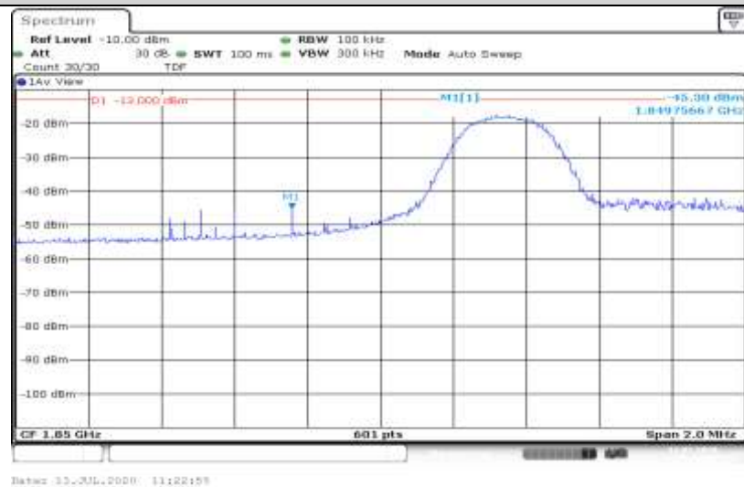
Band25-5MHz-16QAM-26065-25RB#0
