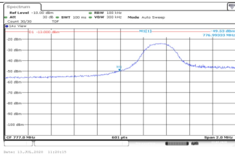
Band13-5MHz-16QAM-23205-1RB#0
