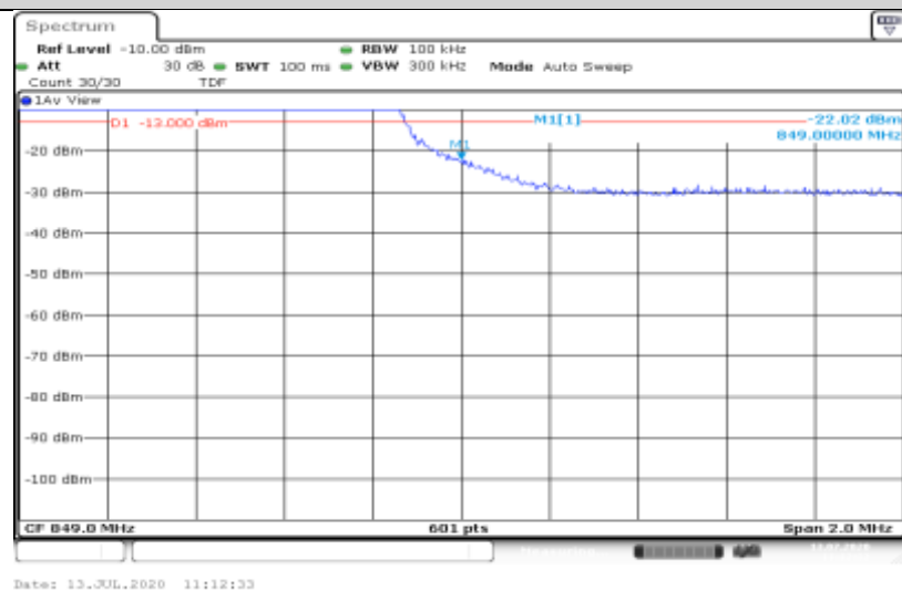
Band5-5MHz-QPSK-20625-25RB#0
