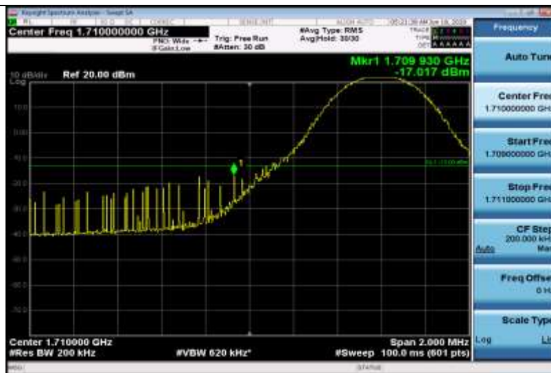
Band4-10MHz-QPSK-20000-1RB#49
