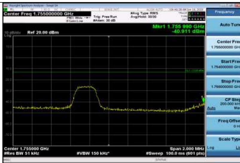
Band4-3MHz-16QAM-20385-1RB#14
