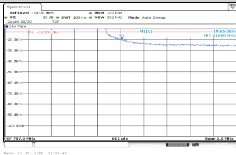
Band13-5MHz-QPSK-23255-25RB#0
