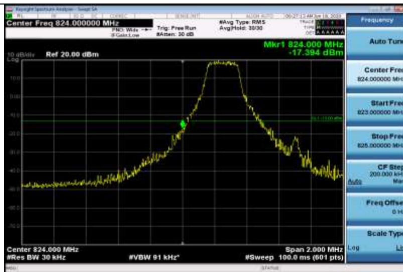
Band5-1.4MHz-16QAM-20407-1RB#5
