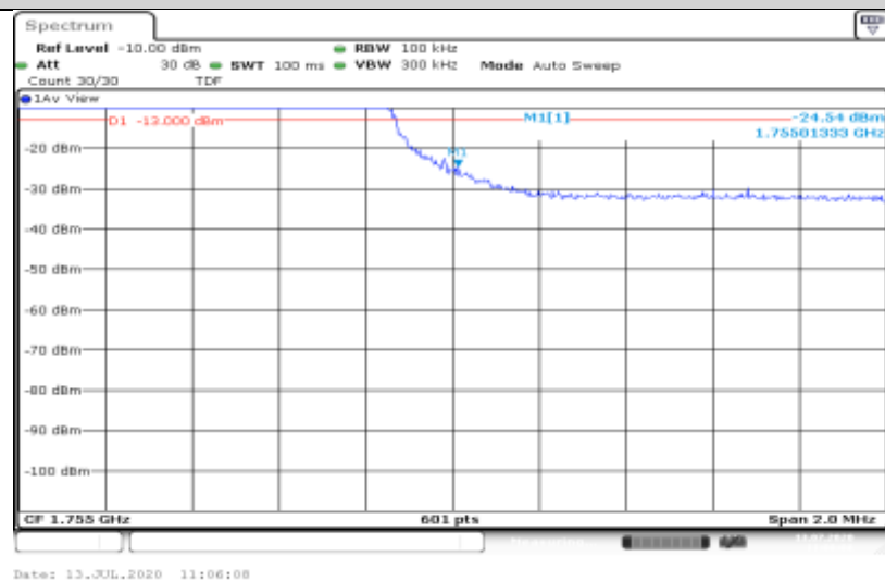
Band4-5MHz-16QAM-20375-25RB#0
