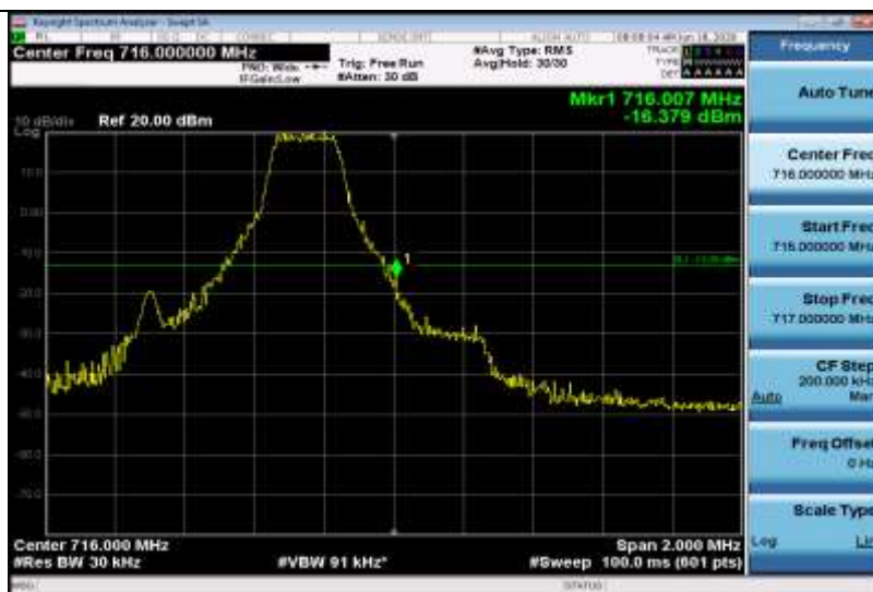
Band12-1.4MHz-16QAM-23173-1RB#0
