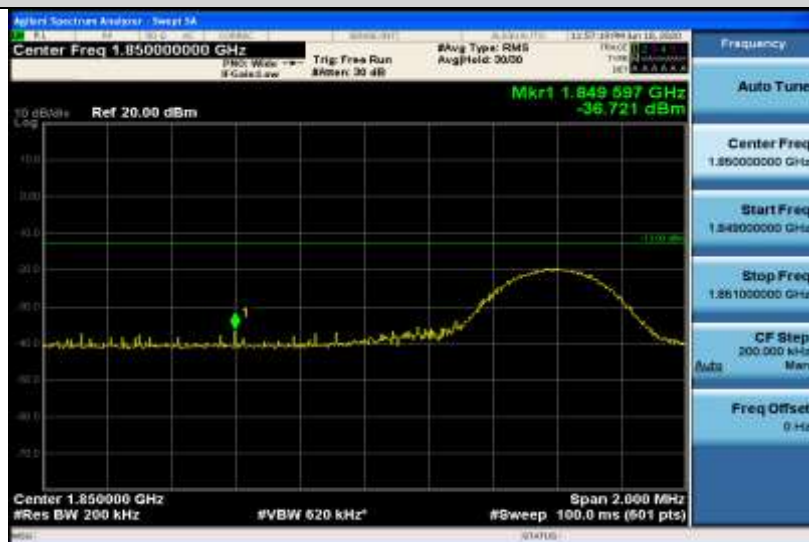
Band25-10MHz-16QAM-26090-50RB#0
