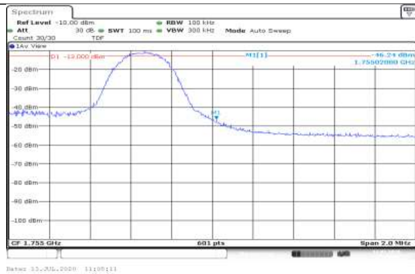
Band4-5MHz-QPSK-20375-1RB#24
