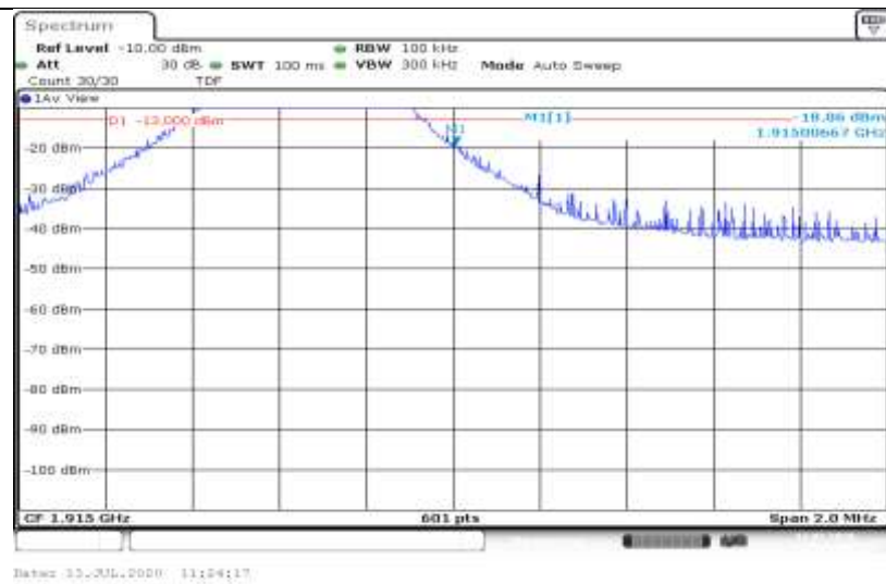
Band25-5MHz-16QAM-26665-1RB#0
