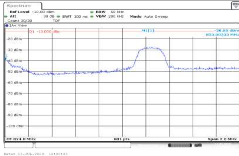
Band5-3MHz-16QAM-20415-15RB#0
