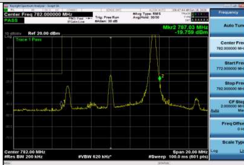
Band13-10MHz-16QAM-23230-50RB#0
