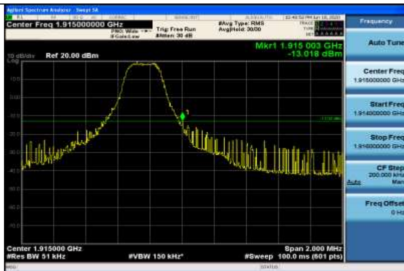
Band25-3MHz-QPSK-26675-1RB#0
