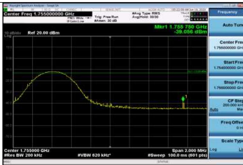
Band4-10MHz-QPSK-20350-1RB#49
