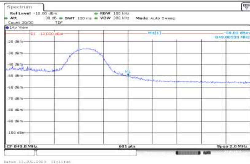
Band5-5MHz-QPSK-20625-25RB#0
