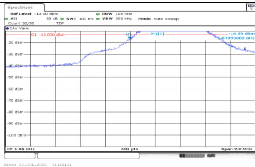
Band25-5MHz-16QAM-26065-1RB#24
