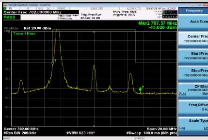
Band13-10MHz-QPSK-23230-50RB#0
