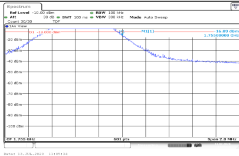
Band4-5MHz-QPSK-20375-25RB#0
