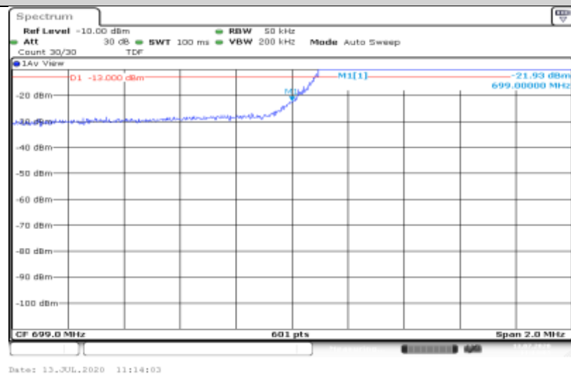
Band12-3MHz-16QAM-23025-15RB#0
