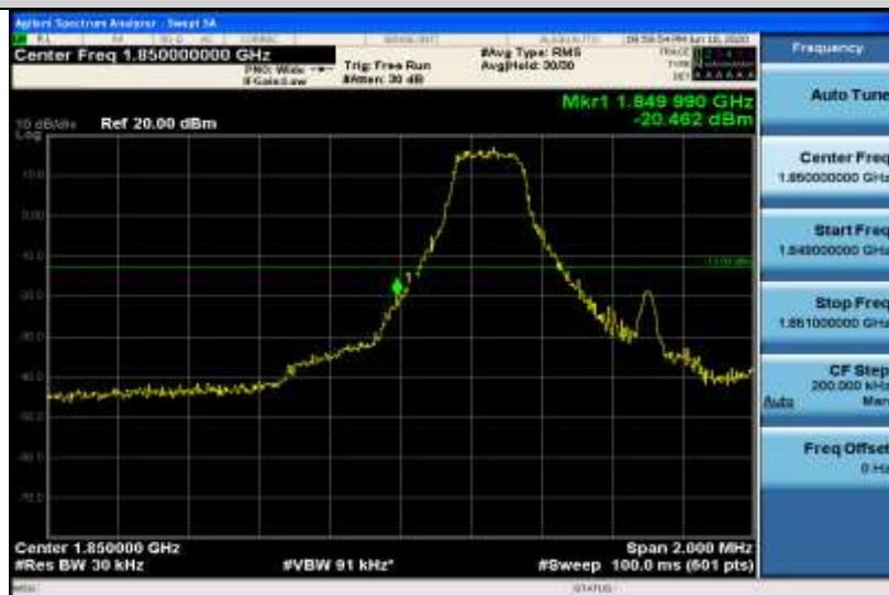
Band25-1.4MHz-QPSK-26047-6RB#0
