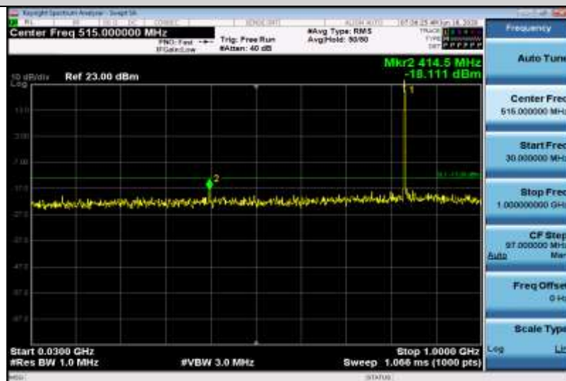
Band5-5MHz-16QAM-20525-1RB#0-Range1:30~1000MHz
