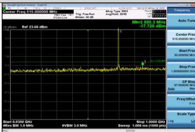
Band12-10MHz-QPSK-23095-1RB#0-Range1:30~1000MHz
