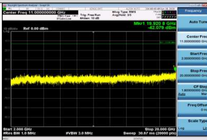
Band4-3MHz-QPSK-20175-1RB#0-Range3:2000~20000MHz
