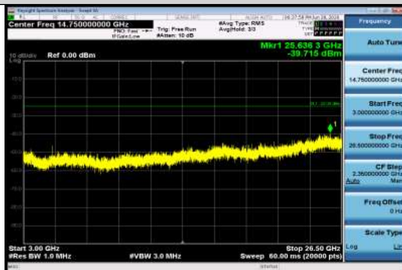
Band7-15MHz-16QAM-21375-1RB#0-Range3:3000~26500MHz
