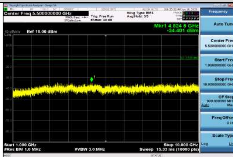
Band5-1.4MHz-QPSK-20643-1RB#0-Range2:1000~10000MHz
