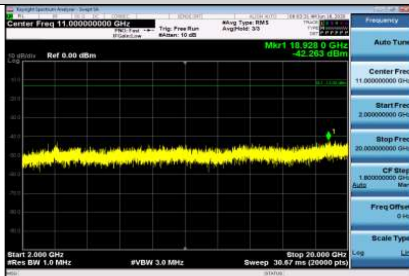
Band4-20MHz-QPSK-20175-1RB#0-Range3:2000~20000MHz
