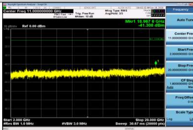
Band4-20MHz-QPSK-20050-1RB#0-Range3:2000~20000MHz
