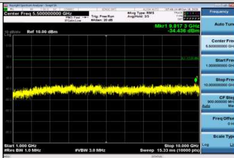
Band5-10MHz-QPSK-20600-1RB#0-Range2:1000~10000MHz
