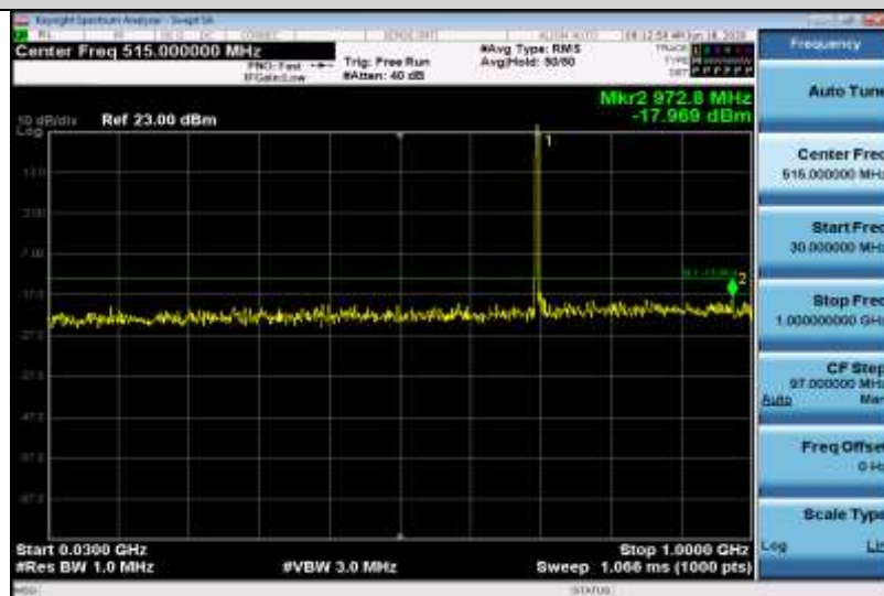
Band12-10MHz-16QAM-23095-1RB#0-Range1:30~1000MHz
