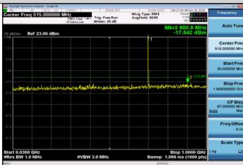
Band12-1.4MHz-16QAM-23095-1RB#0-Range1:30~1000MHz
