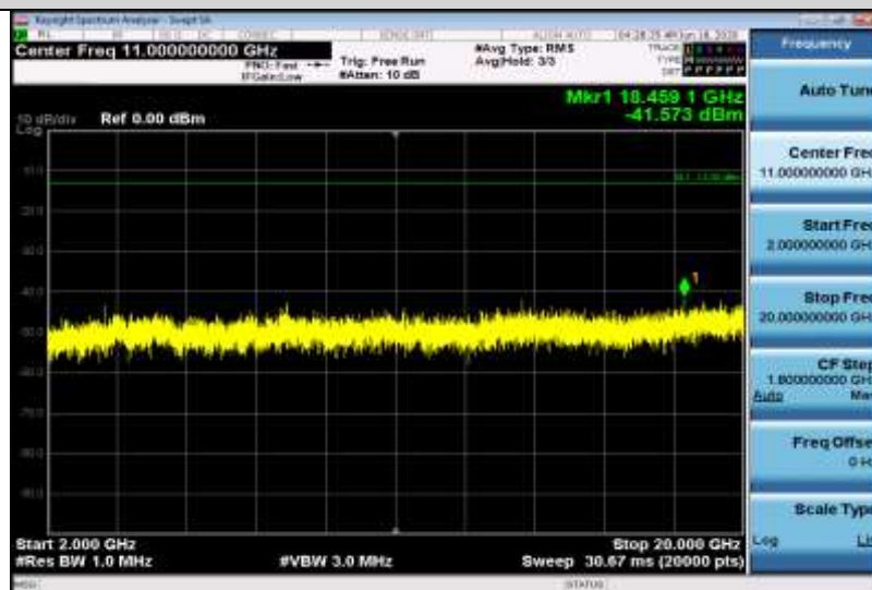
Band4-1.4MHz-QPSK-20175-1RB#0-Range3:2000~20000MHz
