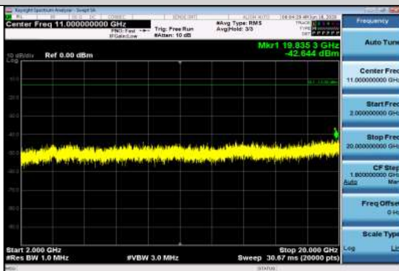
Band4-20MHz-QPSK-20300-1RB#0-Range3:2000~20000MHz
