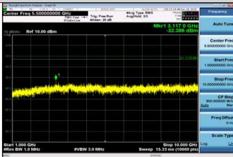
Band12-10MHz-QPSK-23130-1RB#0-Range2:1000~10000MHz
