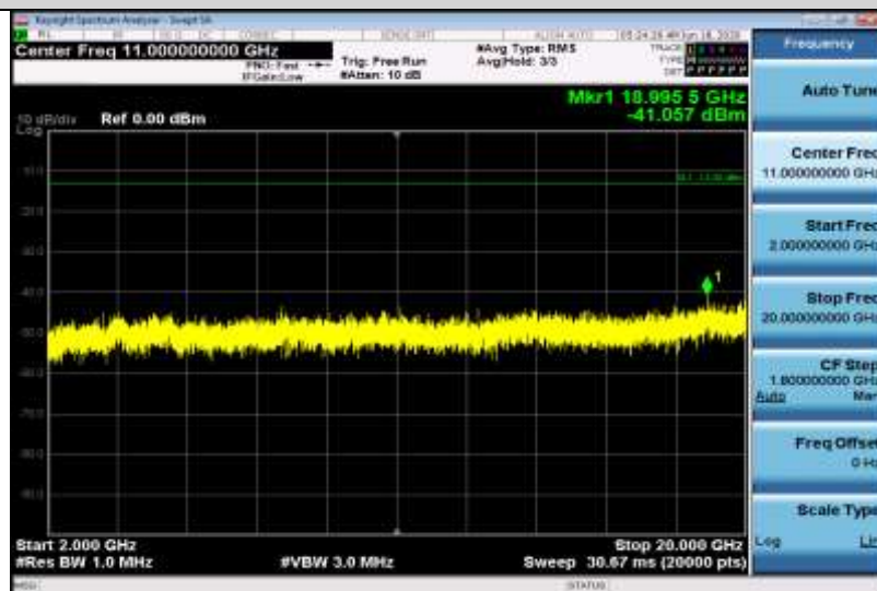
Band4-10MHz-QPSK-20000-1RB#0-Range3:2000~20000MHz
