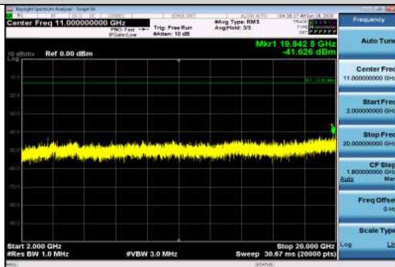
Band4-1.4MHz-16QAM-20393-1RB#0-Range3:2000~20000MHz
