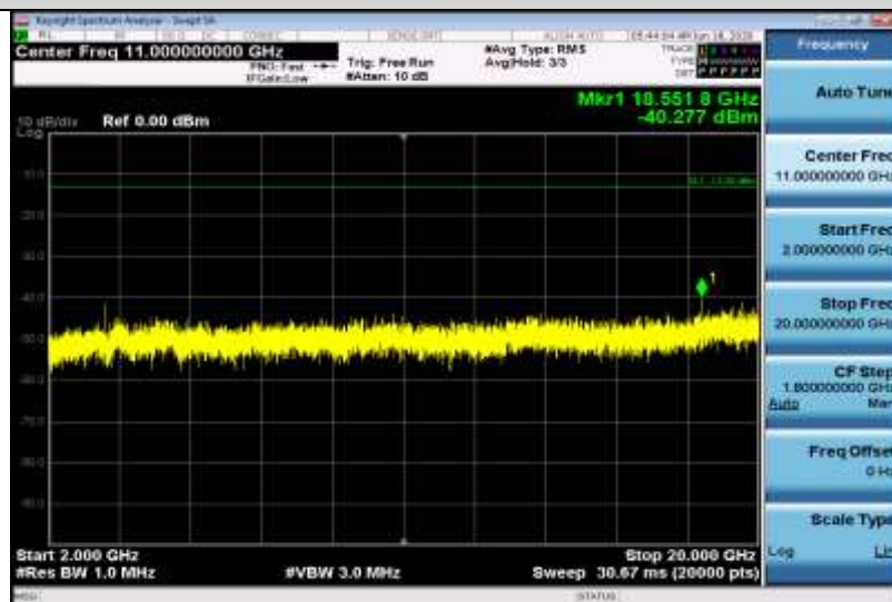
Band4-15MHz-QPSK-20175-1RB#0-Range3:2000~20000MHz
