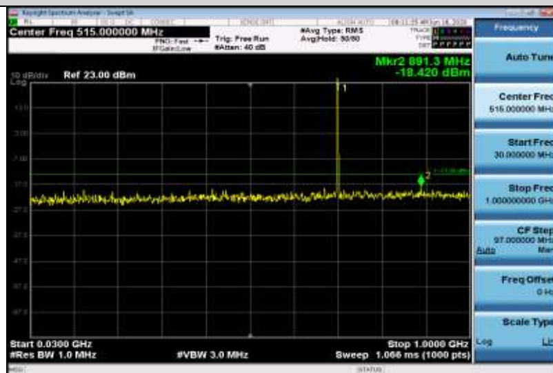
Band12-1.4MHz-QPSK-23095-1RB#0-Range1:30~1000MHz
