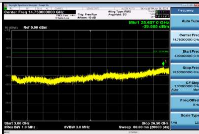
Band7-20MHz-16QAM-21100-1RB#0-Range3:3000~26500MHz
