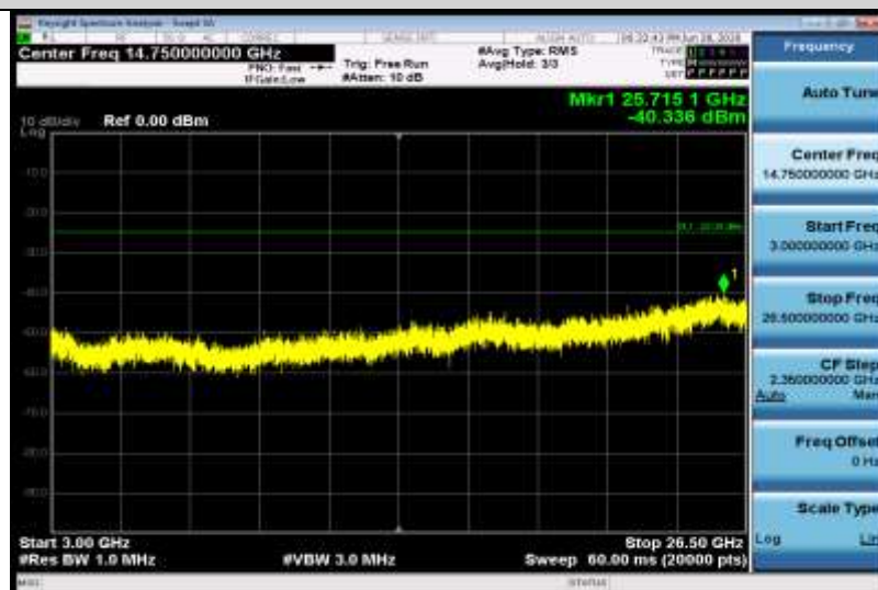
Band7-10MHz-16QAM-21100-1RB#0-Range3:3000~26500MHz
