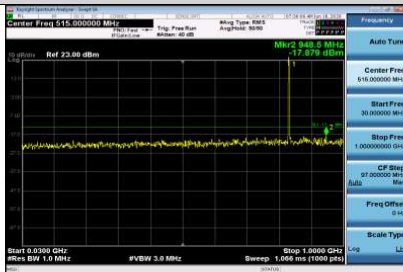
Band5-5MHz-QPSK-20525-1RB#0-Range1:30~1000MHz
