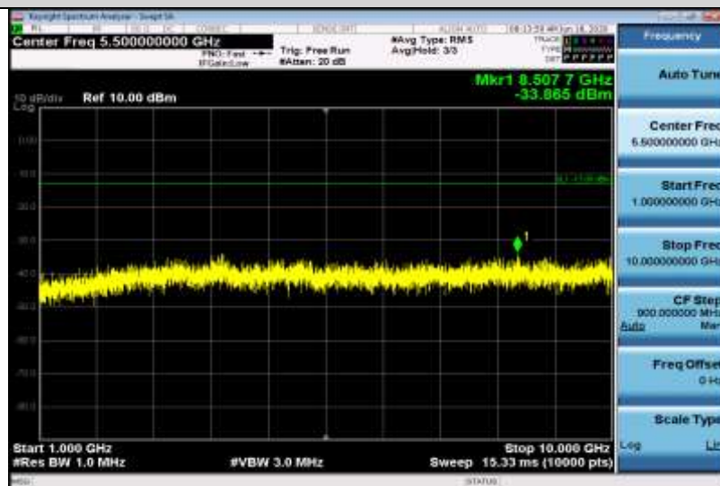
Band12-1.4MHz-16QAM-23173-1RB#0-Range2:1000~10000MHz
