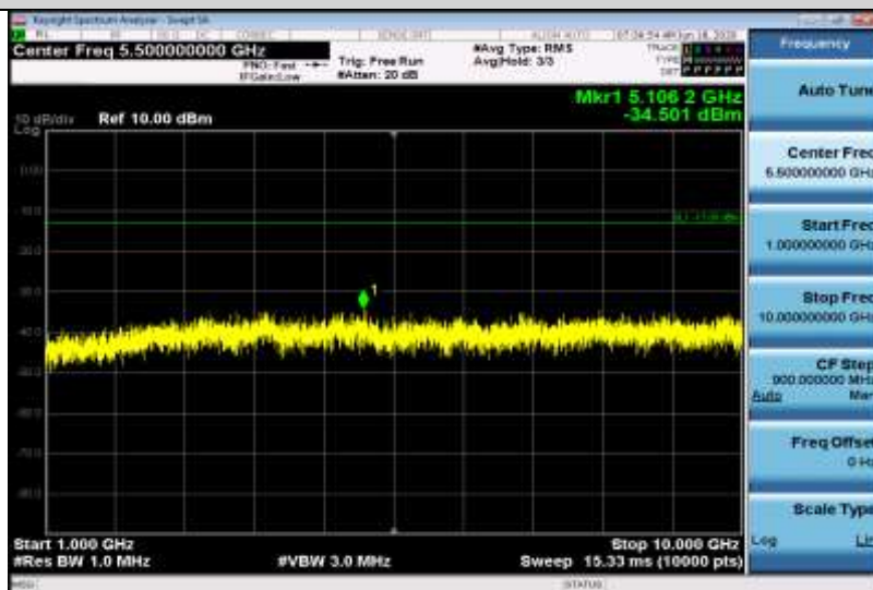
Band5-5MHz-QPSK-20625-1RB#0-Range2:1000~10000MHz
