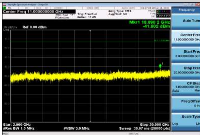
Band4-1.4MHz-QPSK-19957-1RB#0-Range3:2000~20000MHz
