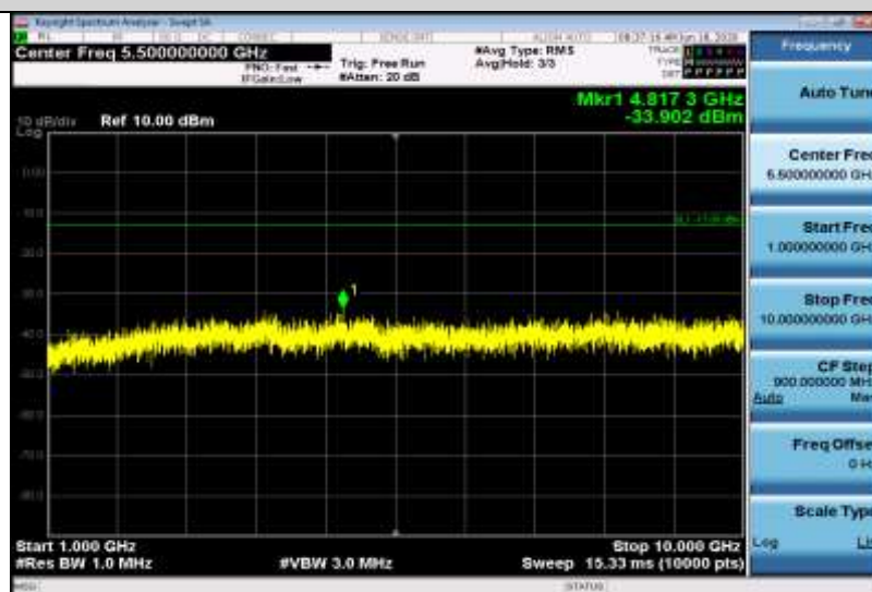
Band12-3MHz-16QAM-23165-1RB#0-Range2:1000~10000MHz
