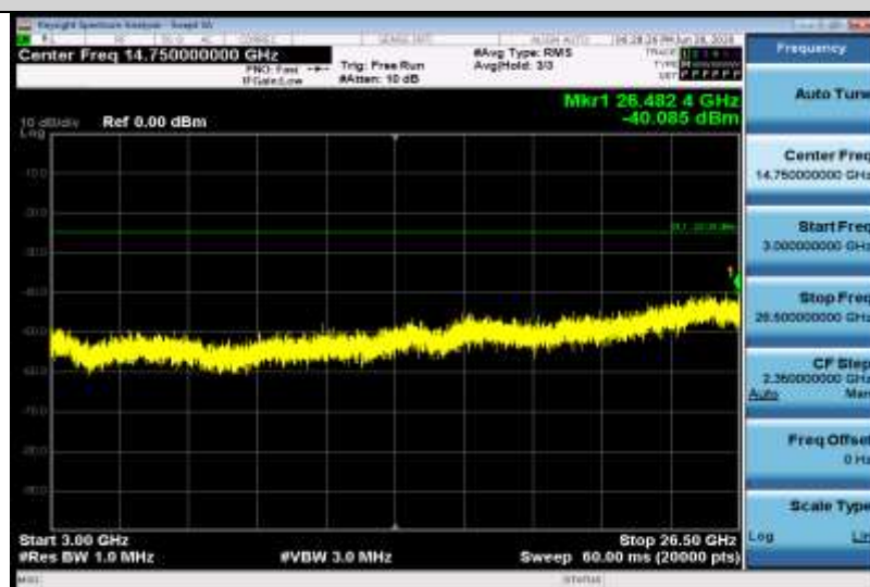
Band7-5MHz-16QAM-21100-1RB#0-Range3:3000~26500MHz
