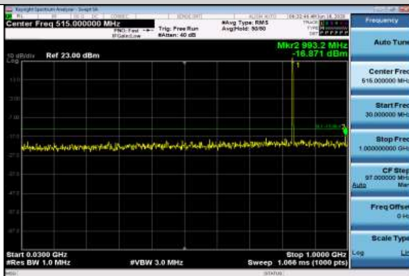
Band5-1.4MHz-16QAM-20525-1RB#0-Range1:30~1000MHz
