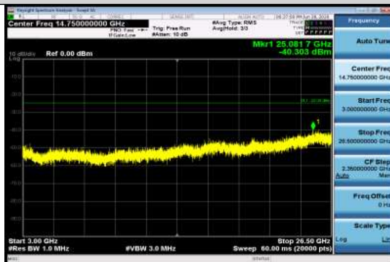
Band7-15MHz-16QAM-21100-1RB#0-Range3:3000~26500MHz
