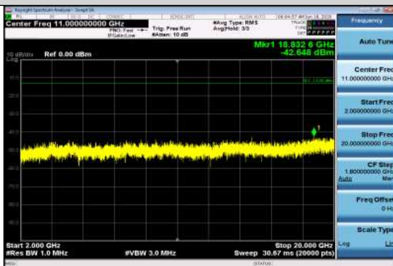
Band4-20MHz-16QAM-20300-1RB#0-Range3:2000~20000MHz
