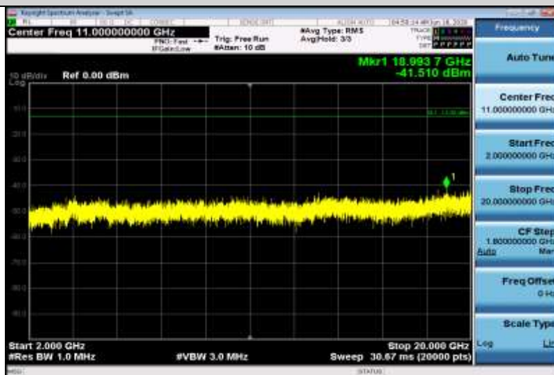
Band4-3MHz-16QAM-20385-1RB#0-Range3:2000~20000MHz
