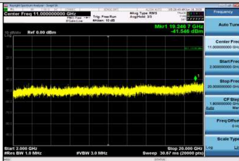
Band4-10MHz-16QAM-20350-1RB#0-Range3:2000~20000MHz
