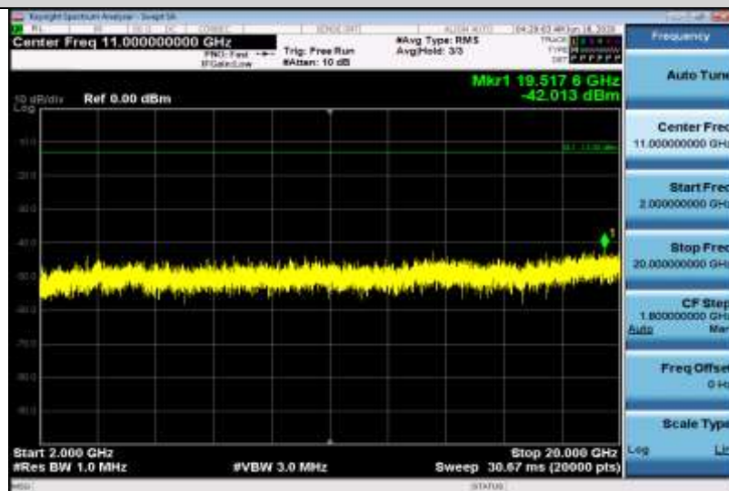
Band4-1.4MHz-16QAM-20175-1RB#0-Range3:2000~20000MHz
