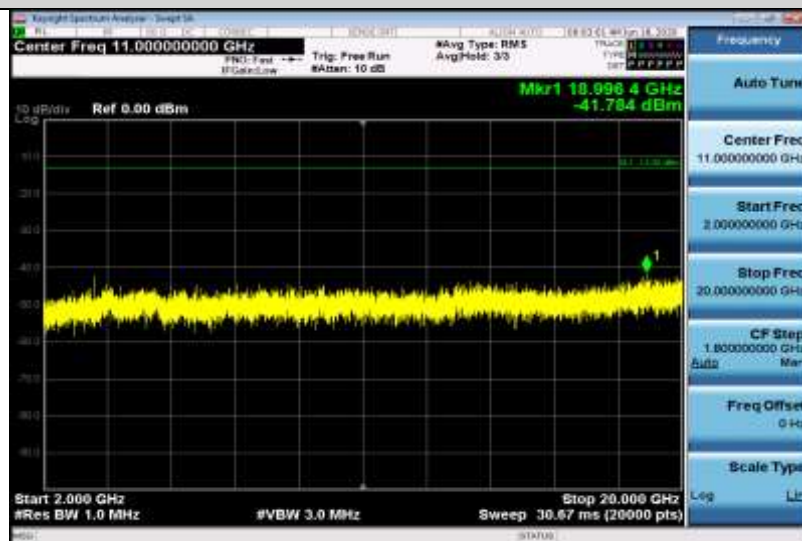
Band4-20MHz-16QAM-20050-1RB#0-Range3:2000~20000MHz
