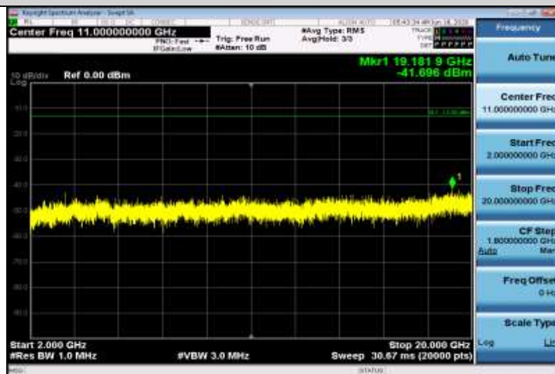
Band4-15MHz-16QAM-20025-1RB#0-Range3:2000~20000MHz
