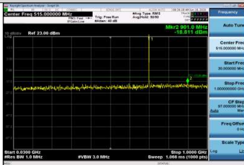
Band12-3MHz-16QAM-23095-1RB#0-Range1:30~1000MHz
