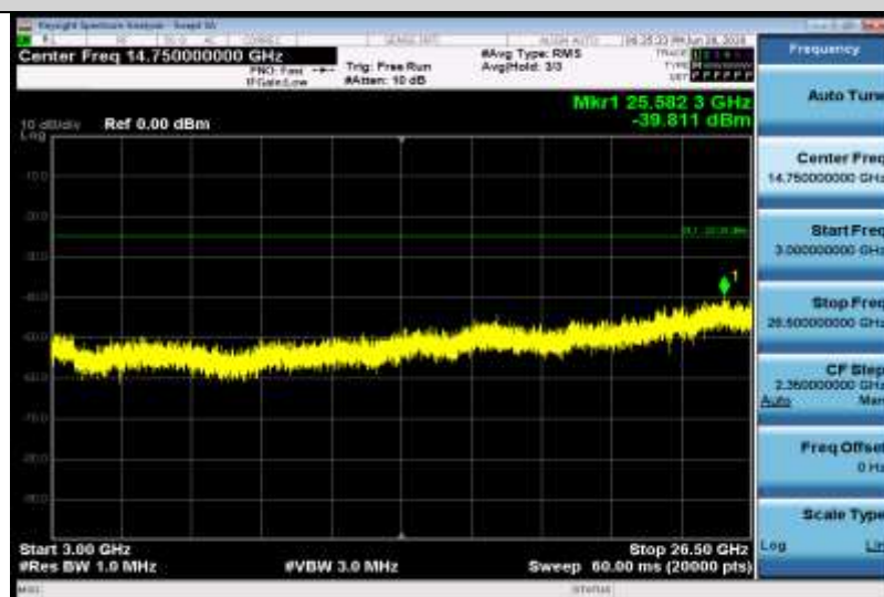
Band7-15MHz-QPSK-20825-1RB#0-Range3:3000~26500MHz
