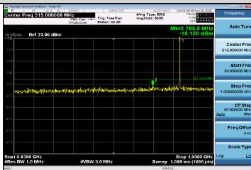
Band5-3MHz-QPSK-20525-1RB#0-Range1:30~1000MHz
