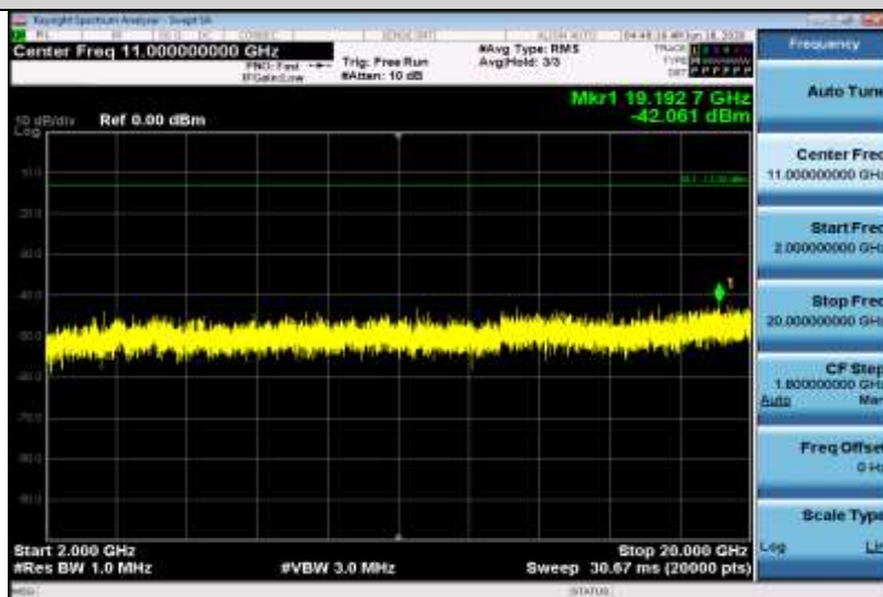
Band4-3MHz-16QAM-20175-1RB#0-Range3:2000~20000MHz
