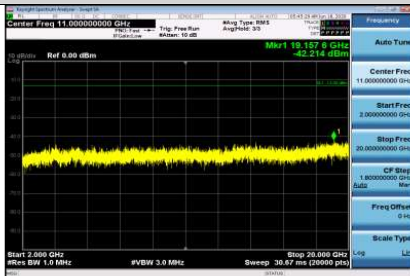
Band4-15MHz-16QAM-20325-1RB#0-Range3:2000~20000MHz
