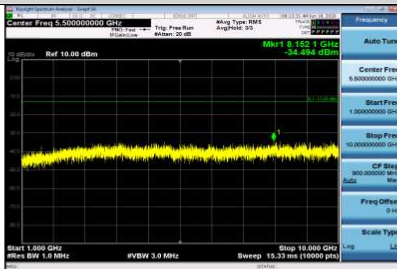
Band12-1.4MHz-QPSK-23173-1RB#0-Range2:1000~10000MHz
