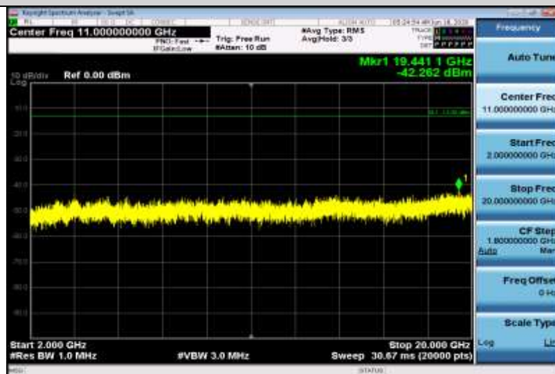
Band4-10MHz-16QAM-20000-1RB#0-Range3:2000~20000MHz
