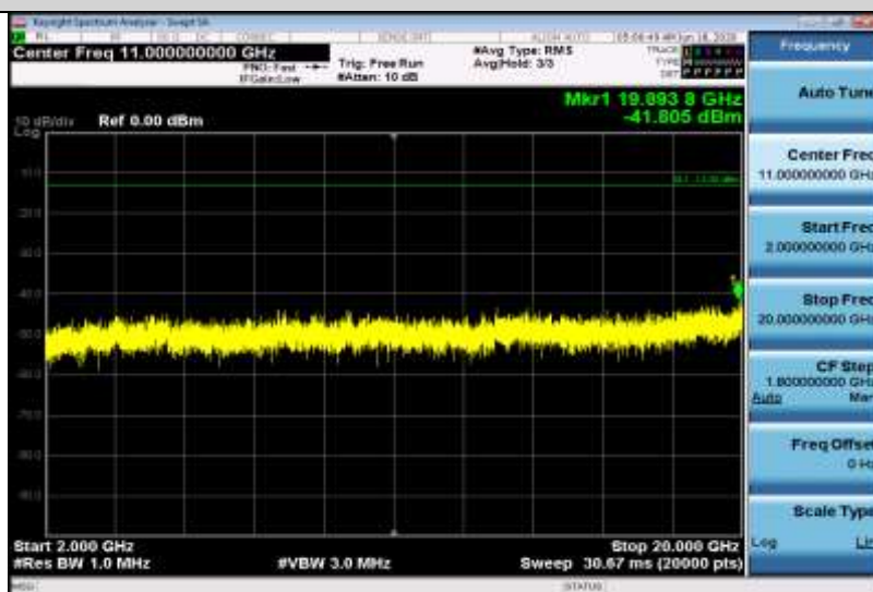
Band4-5MHz-16QAM-19975-1RB#0-Range3:2000~20000MHz
