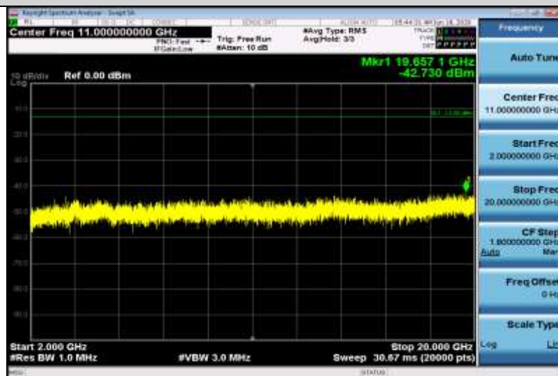
Band4-15MHz-16QAM-20175-1RB#0-Range3:2000~20000MHz
