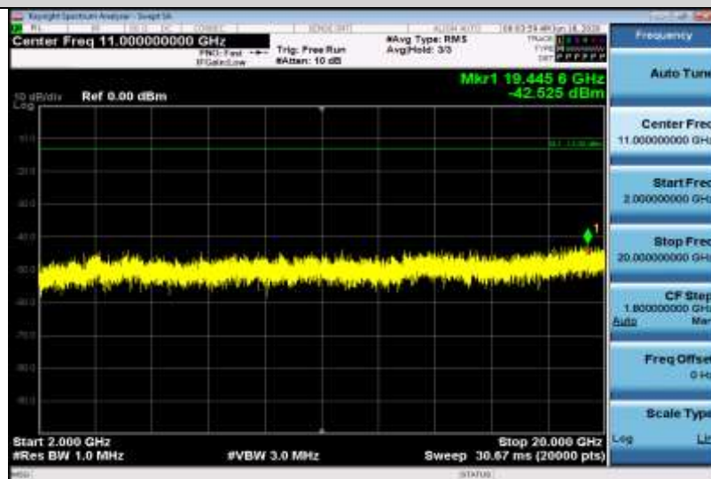
Band4-20MHz-16QAM-20175-1RB#0-Range3:2000~20000MHz
