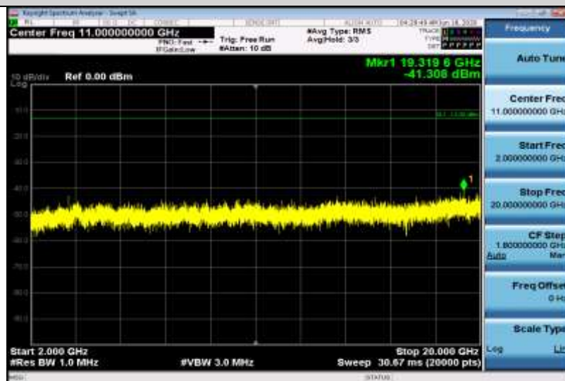
Band4-1.4MHz-QPSK-20393-1RB#0-Range3:2000~20000MHz
