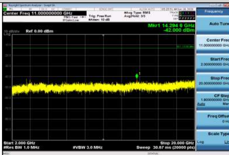
Band4-10MHz-16QAM-20175-1RB#0-Range3:2000~20000MHz
