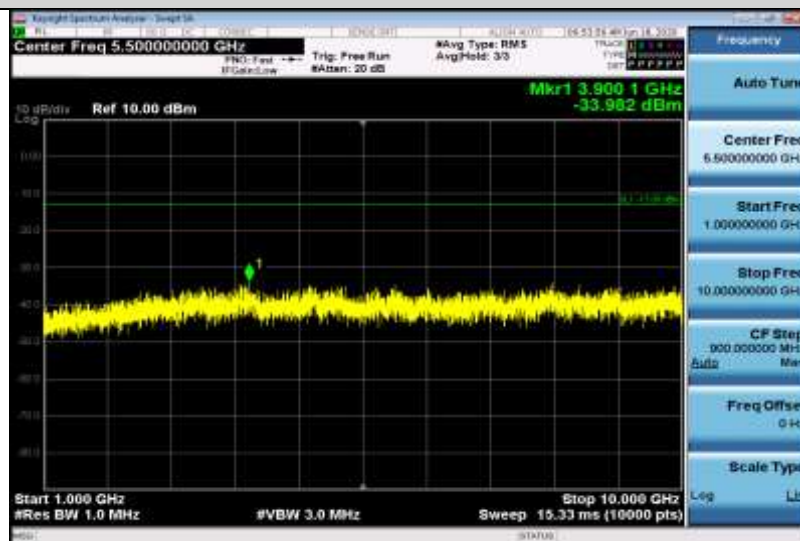
Band5-3MHz-16QAM-20635-1RB#0-Range2:1000~10000MHz
