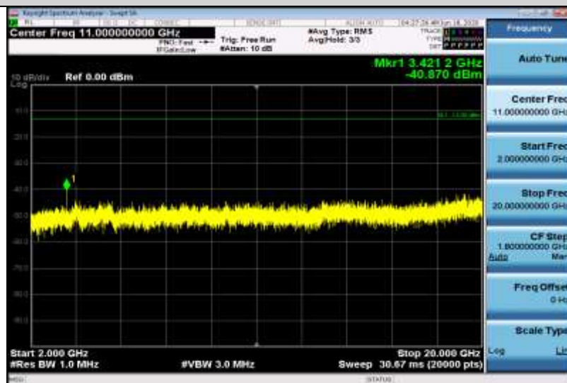
Band4-1.4MHz-16QAM-19957-1RB#0-Range3:2000~20000MHz
