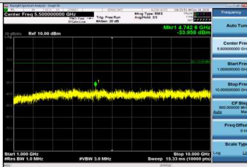
Band5-1.4MHz-16QAM-20643-1RB#0-Range2:1000~10000MHz
