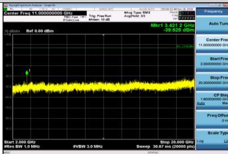
Band4-5MHz-QPSK-19975-1RB#0-Range3:2000~20000MHz
