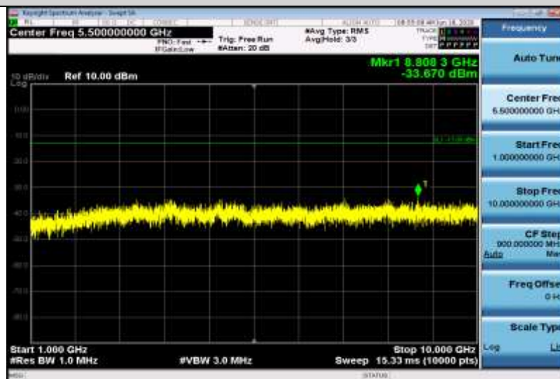
Band12-5MHz-16QAM-23155-1RB#0-Range2:1000~10000MHz
