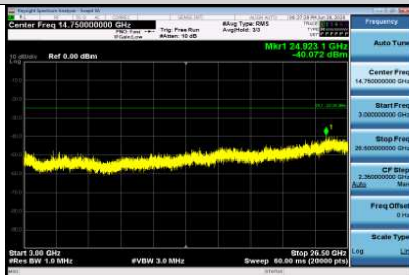
Band7-15MHz-QPSK-21375-1RB#0-Range3:3000~26500MHz
