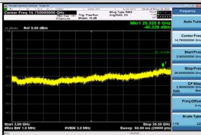
Band7-20MHz-16QAM-20850-1RB#0-Range3:3000~26500MHz
