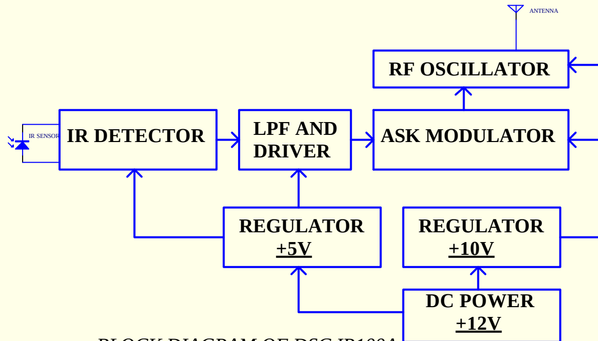
BLOCK DIAGRAM OF DSC IR100A
