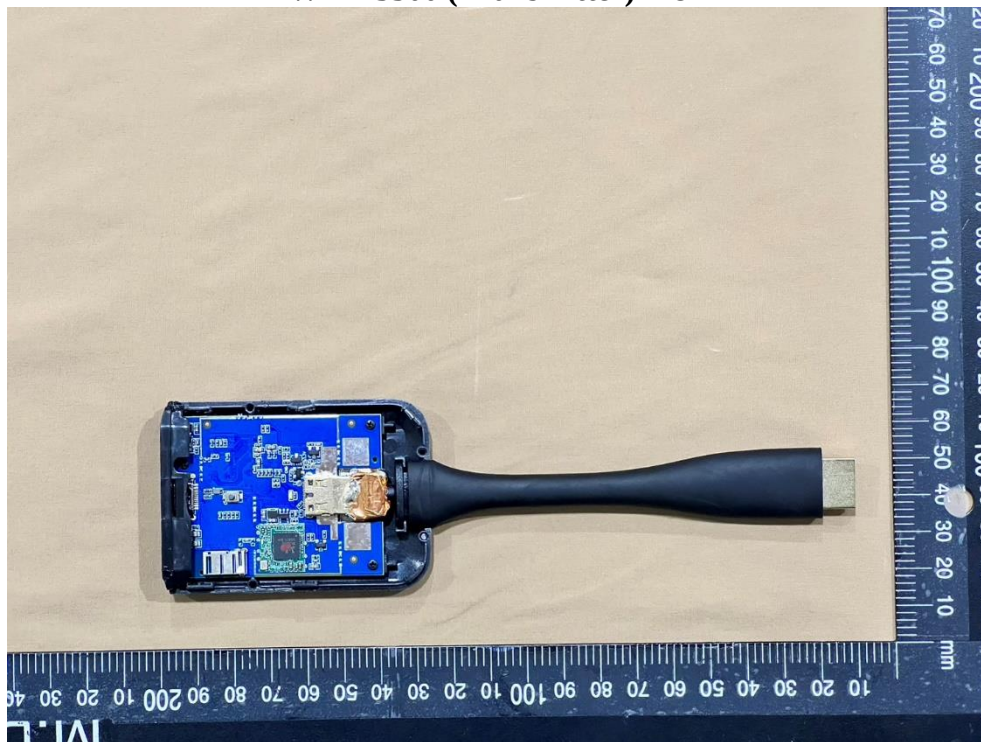
WTR-5500 (Transmitter) Pic 2
