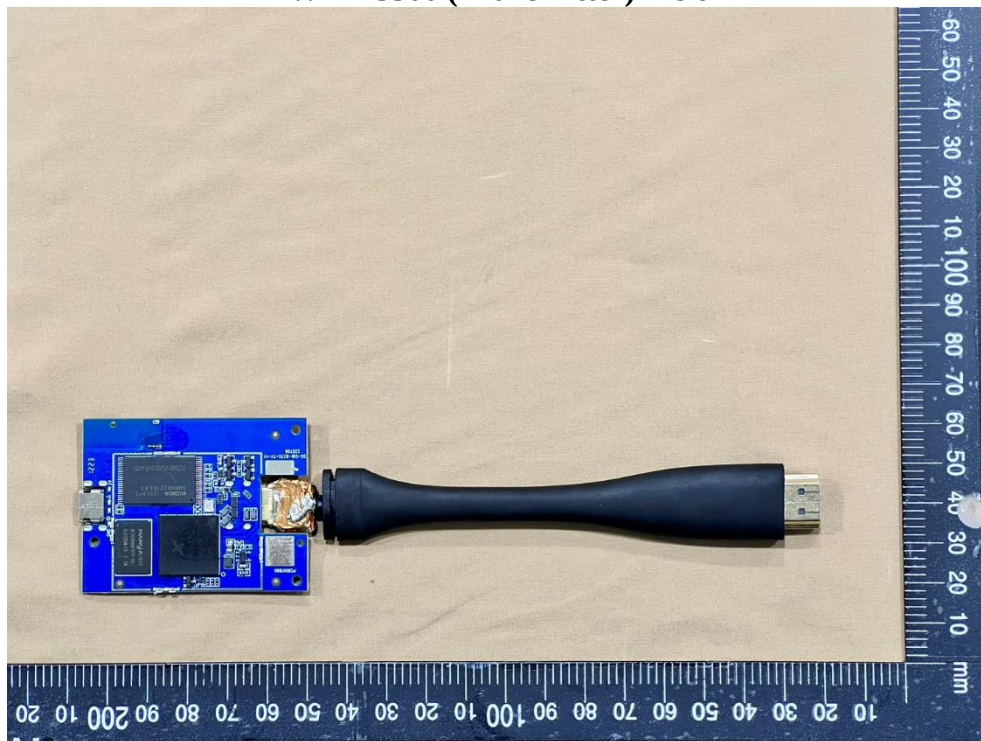
WTR-5500 (Transmitter) Pic 6
