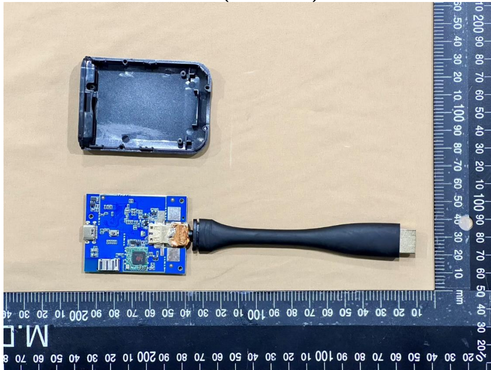
WTR-5500 (Transmitter) Pic 3
