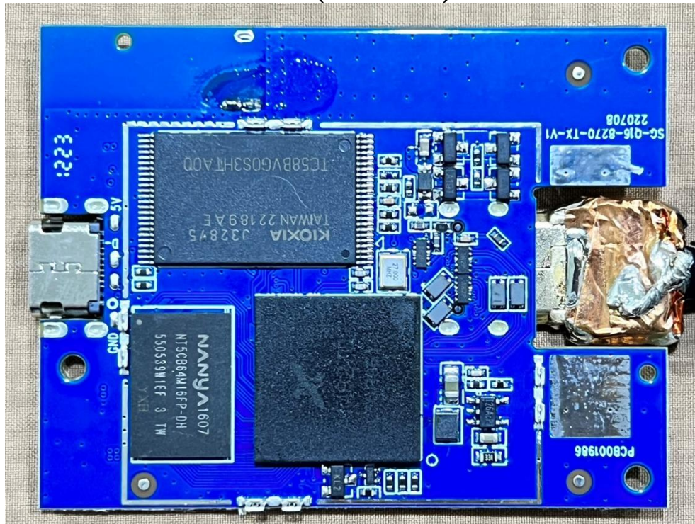
WTR-5500 (Transmitter) Pic 7
