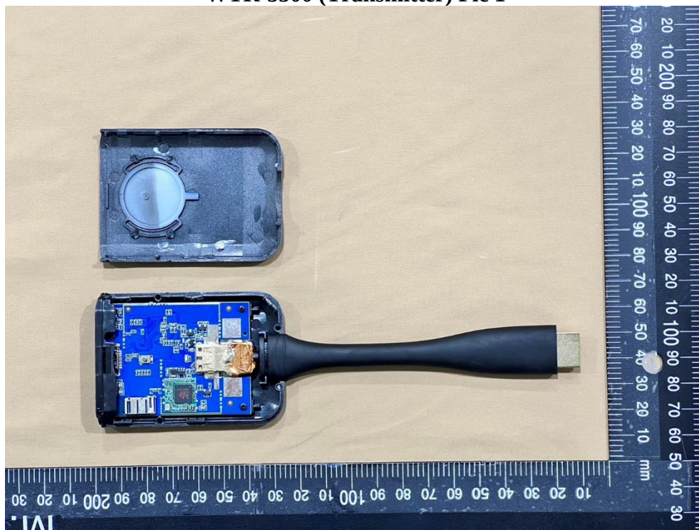
WTR-5500 (Transmitter) Pic 1
