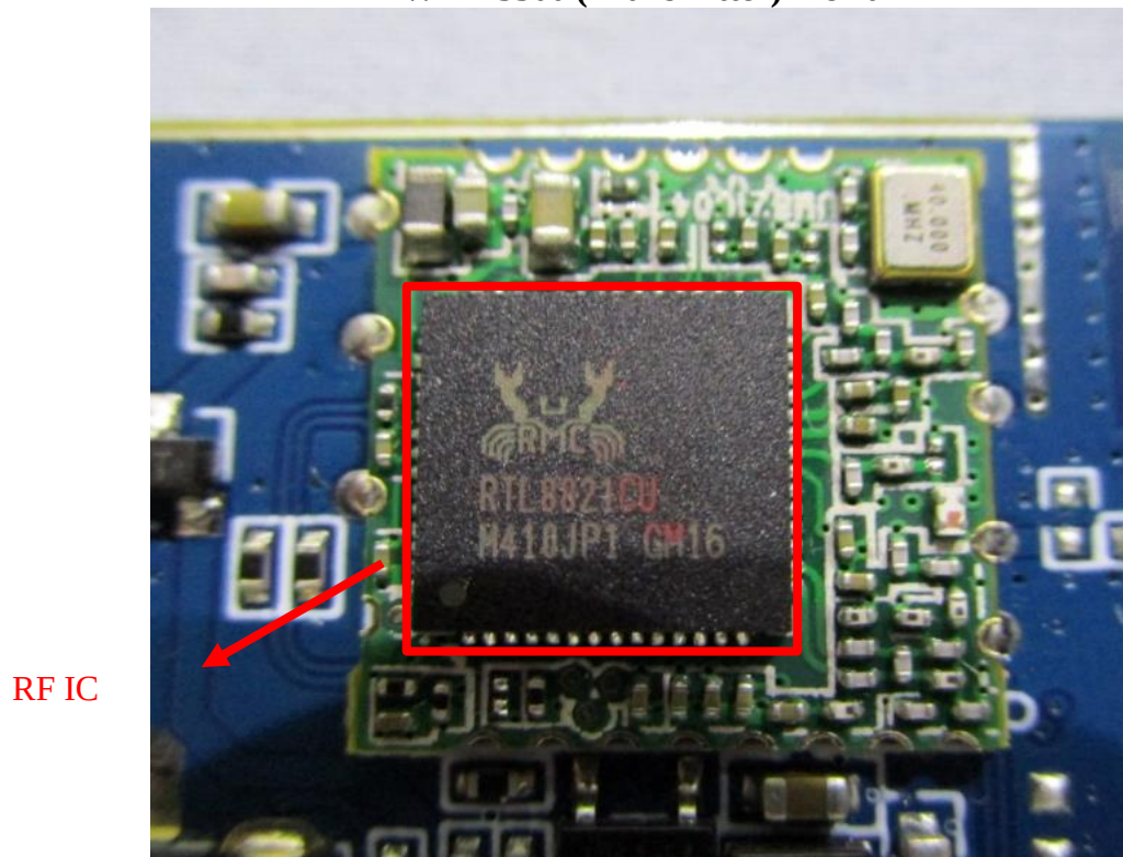
WTR-5500 (Transmitter) Pic 10
