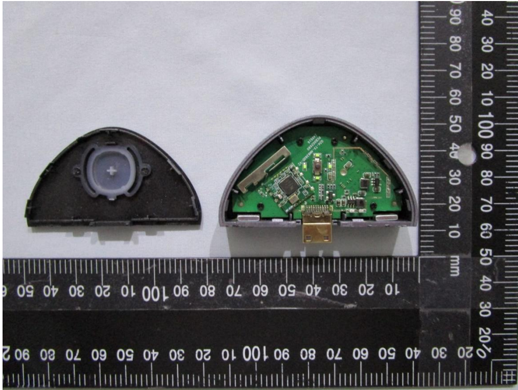
Internal Photos WTR-5600C Pic 1
