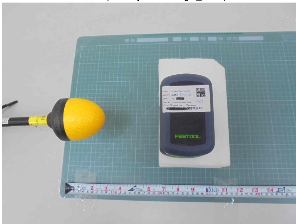
E-Field (Standby Mode - Right_20cm)
