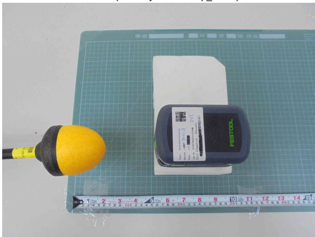
E-Field (Standby Mode - Bottom_15cm)
