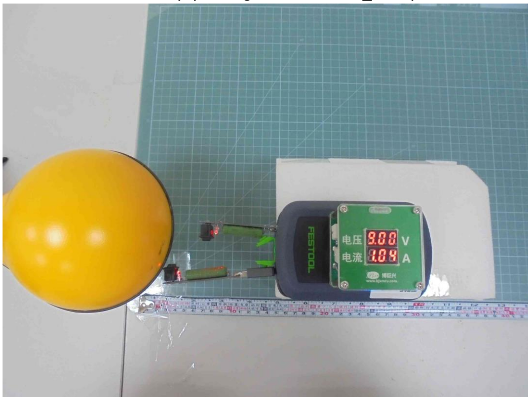
H-Field (Operating Mode - Bottom_15cm)
