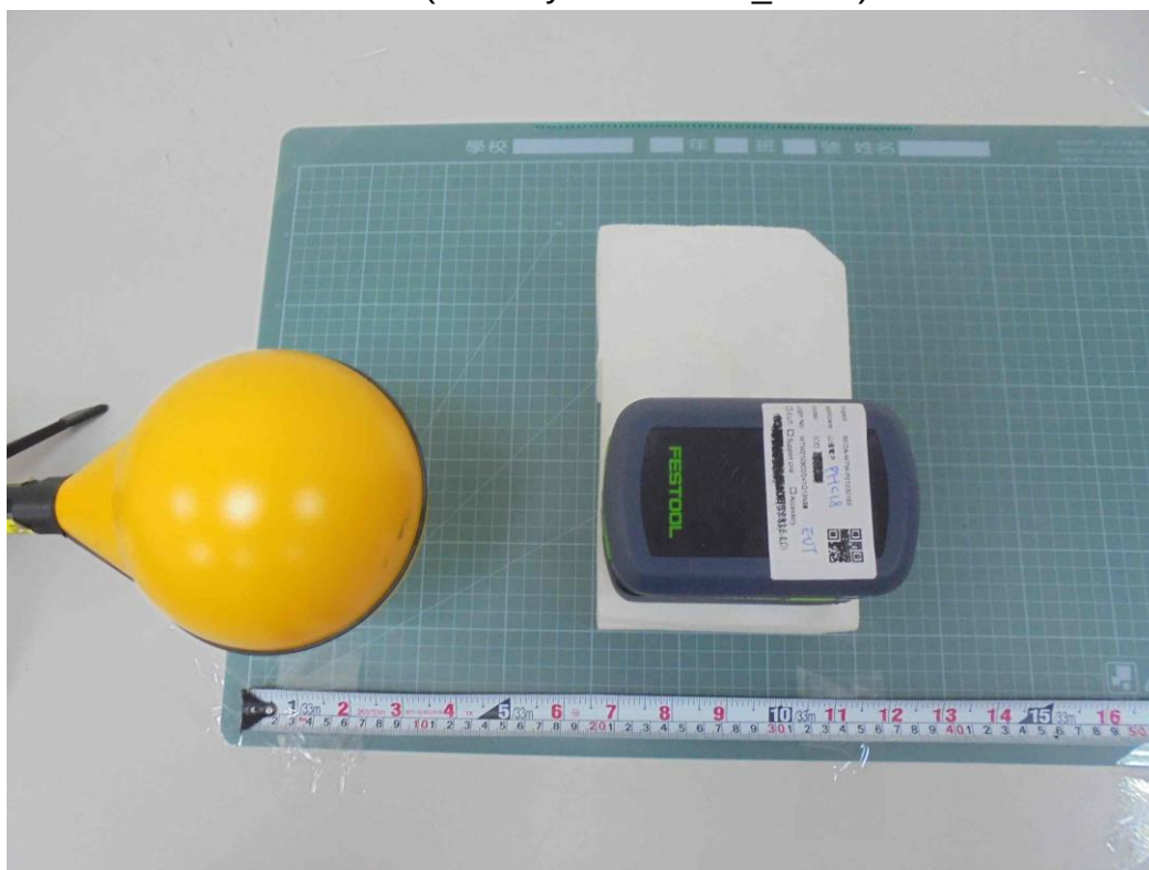
H-Field (Standby Mode - Right_20cm)
