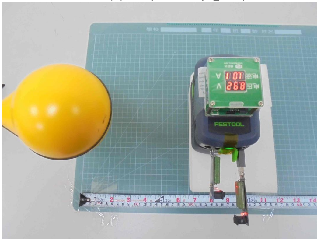
H-Field (Operating Mode - Right_20cm)
