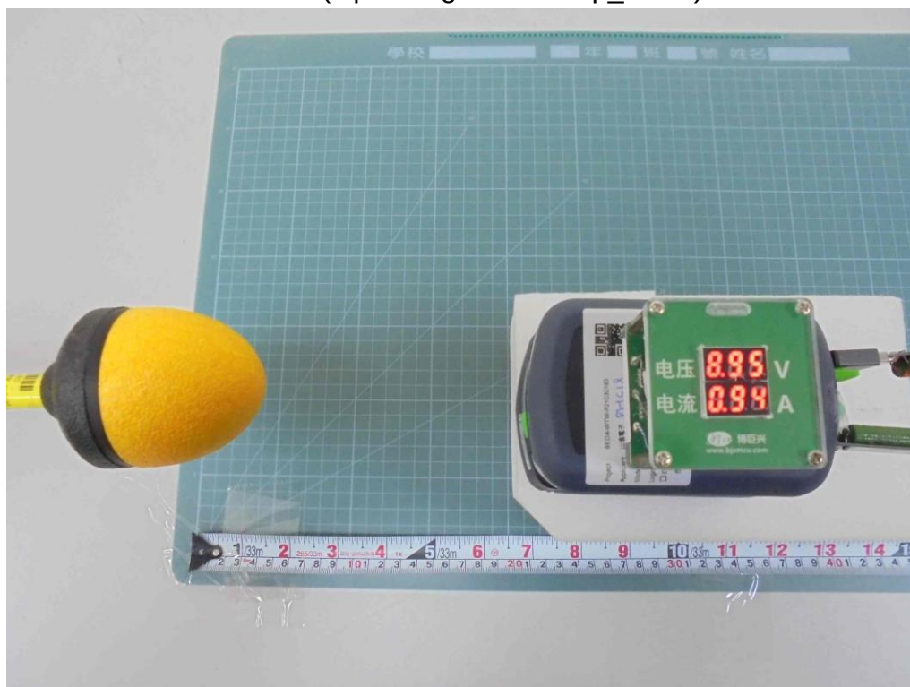
E-Field (Operating Mode - Bottom_20cm)
