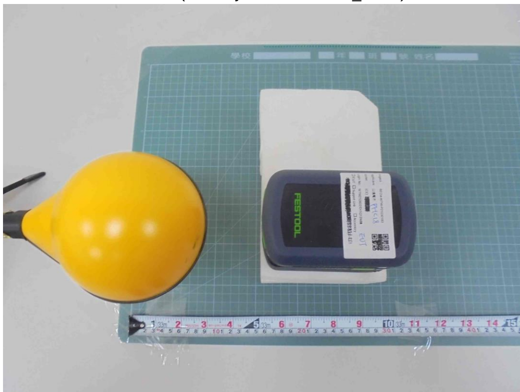
H-Field (Standby Mode - Bottom_15cm)
