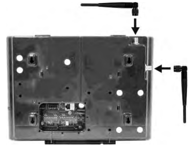
Figure 12. Antenna mounting
