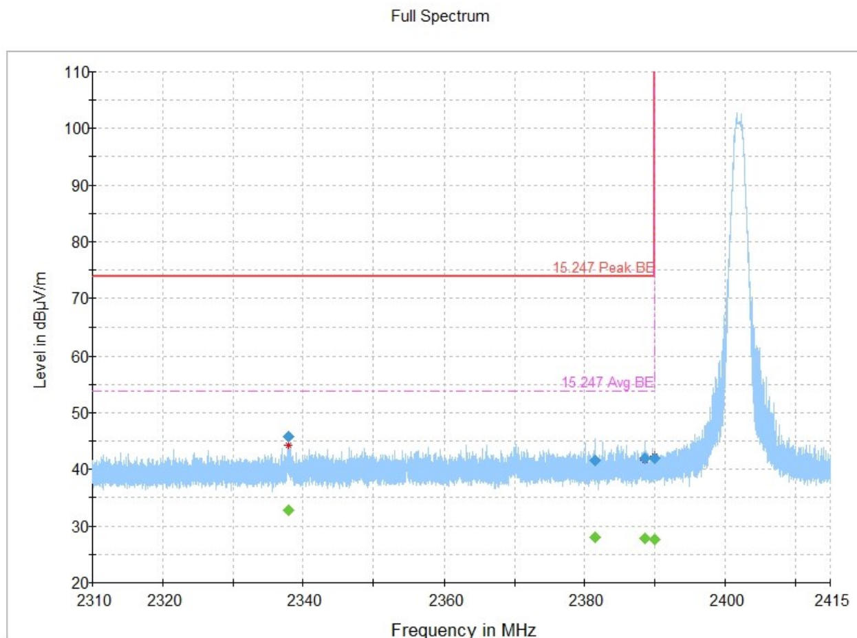
Figure 8.6-1: Radiated emissions, restricted band edge, low
