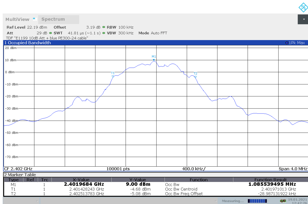
Figure 8.8-1: 99% bandwidth, 2402 MHz
