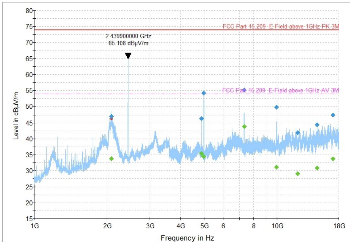
Full Spectrum
