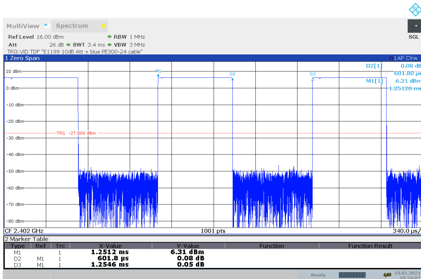
Figure 8.3-1: Duty cycle
