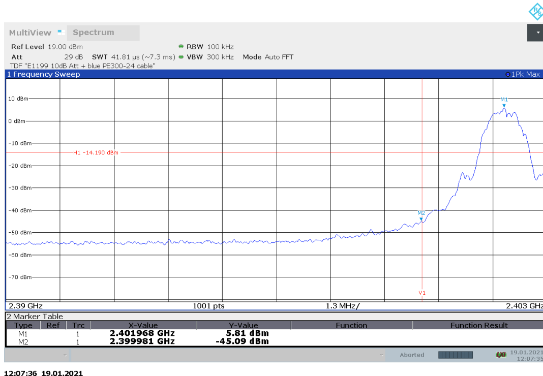
Figure 8.4-1: Band edge measurement, 2402 MHz
