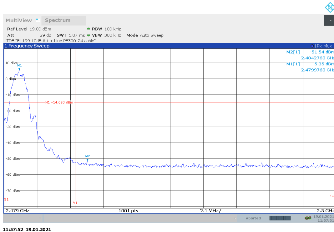
Figure 8.4-2: Band edge measurement, 2480 MHz
