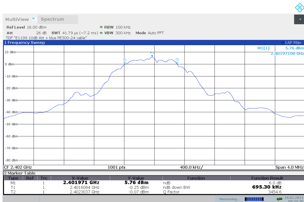
Figure 8.2-1: 6 dB occupied bandwidth, 2402 MHz
