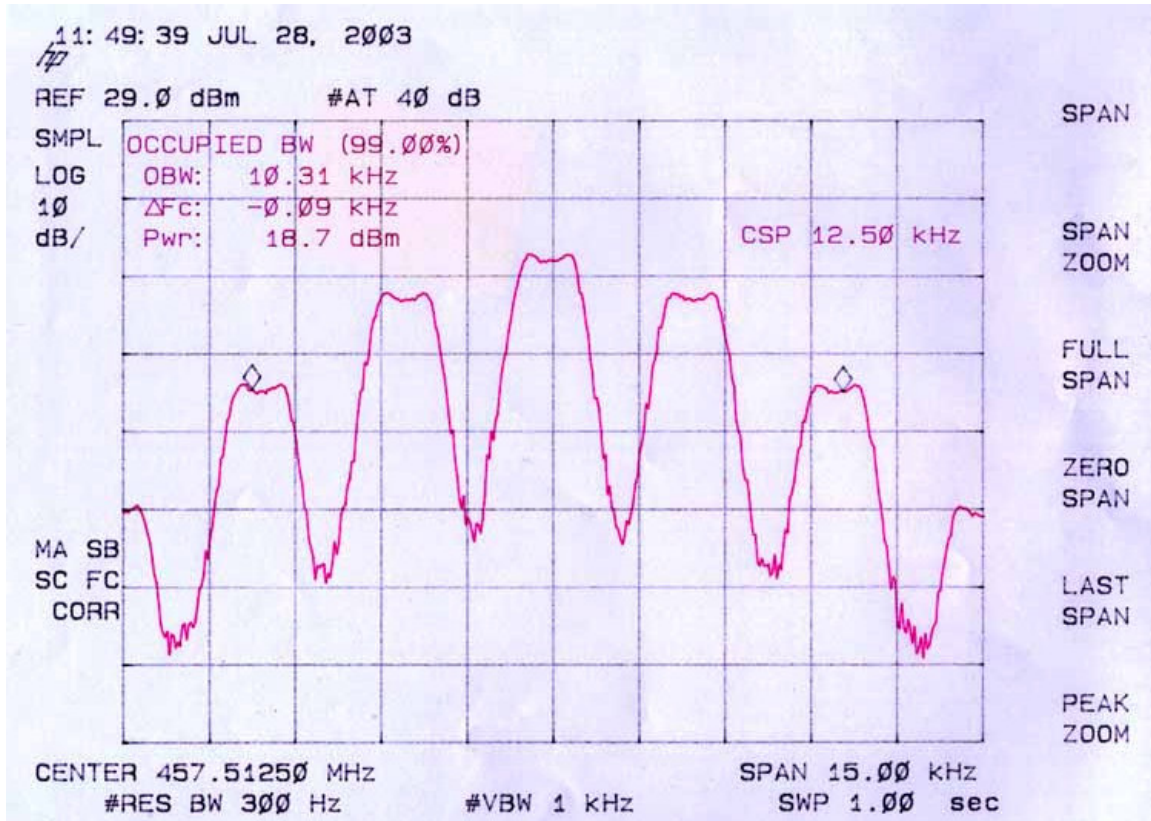
Figure 1 BASE 400 Modulated with 2500Hz + 16dB
