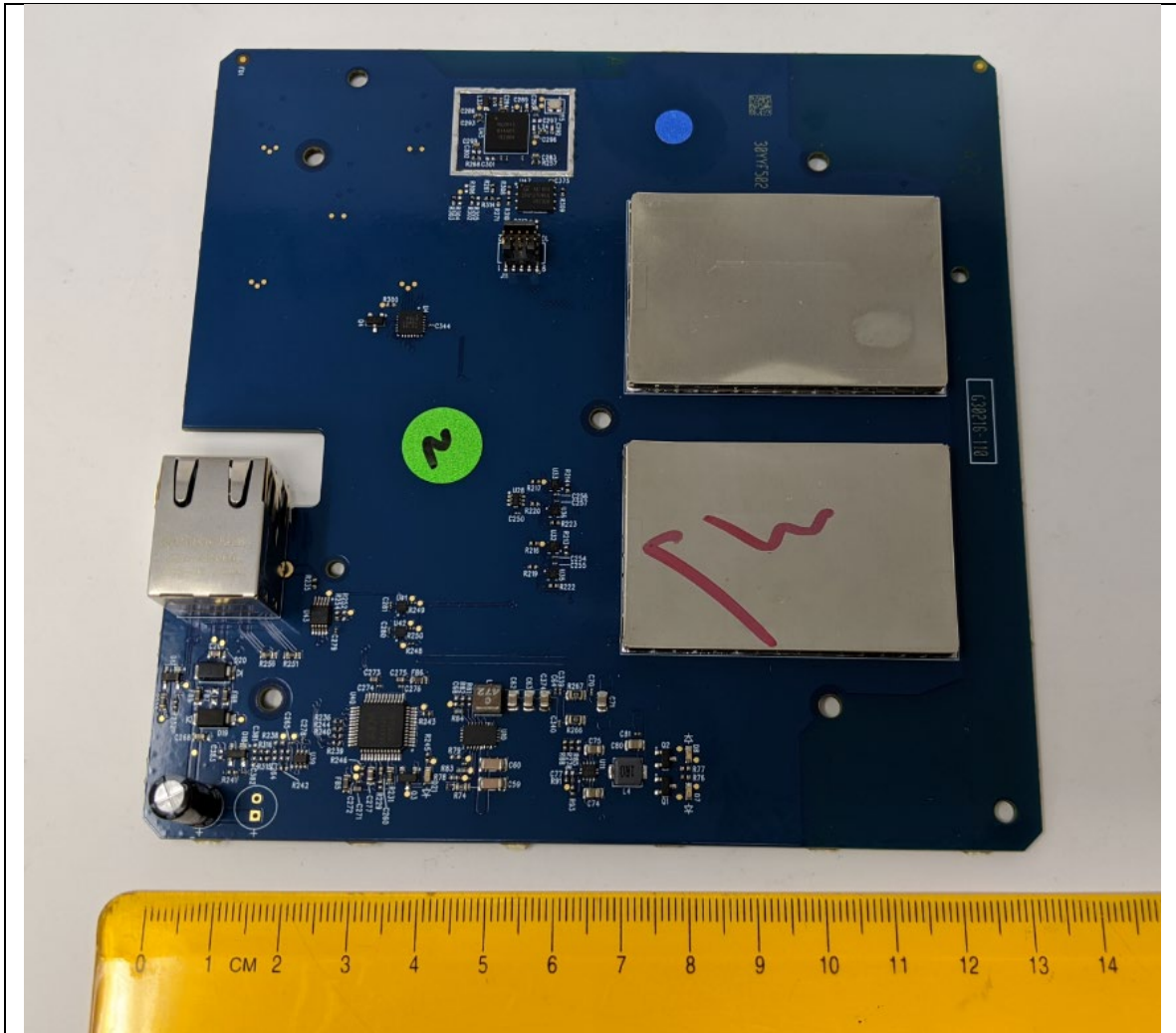
MAIN BOARD TOP VIEW WITH RF SHIELDS
