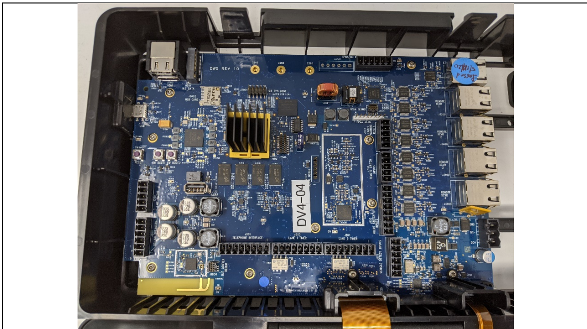
OPEN ENCLOSURE VIEW 2
