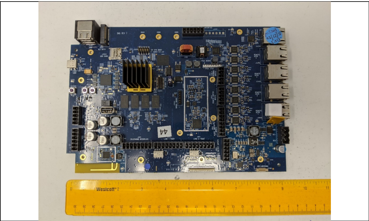
PCB TOP VIEW
