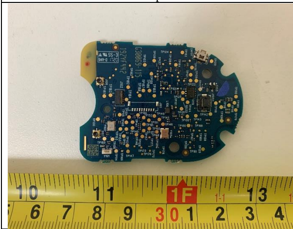
Internal - Main PCBA Bottom
