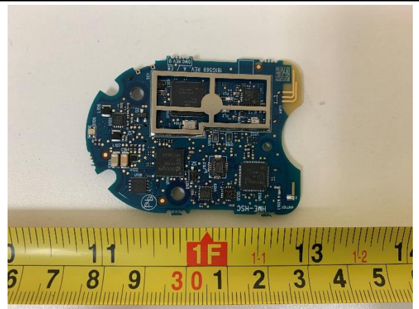
Internal - Main PCBA Top
