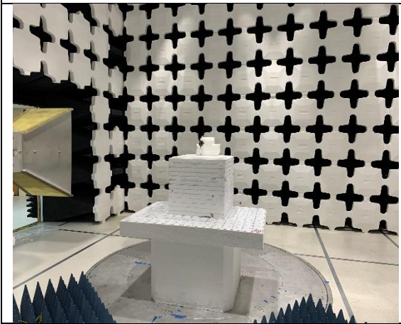
Radiated Emission-Above 1GHz-Front
