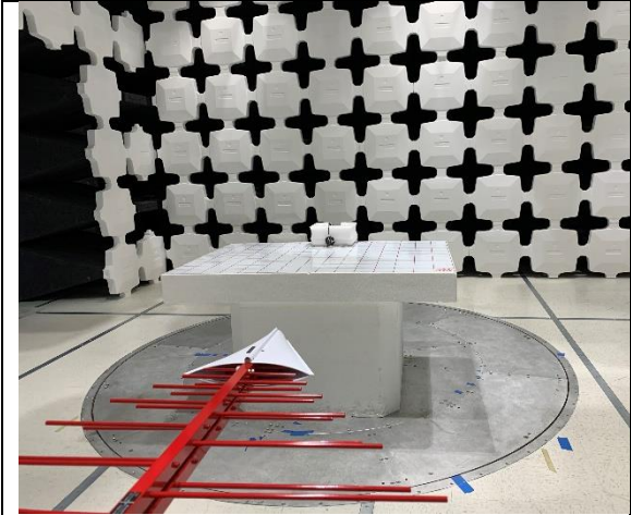
Radiated Emission-Below 1GHz-Front
