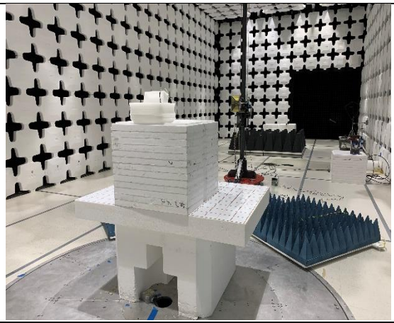
Radiated Emission-Above 1GHz-Back
