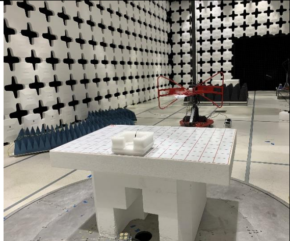
Radiated Emission-Below 1GHz-Back
