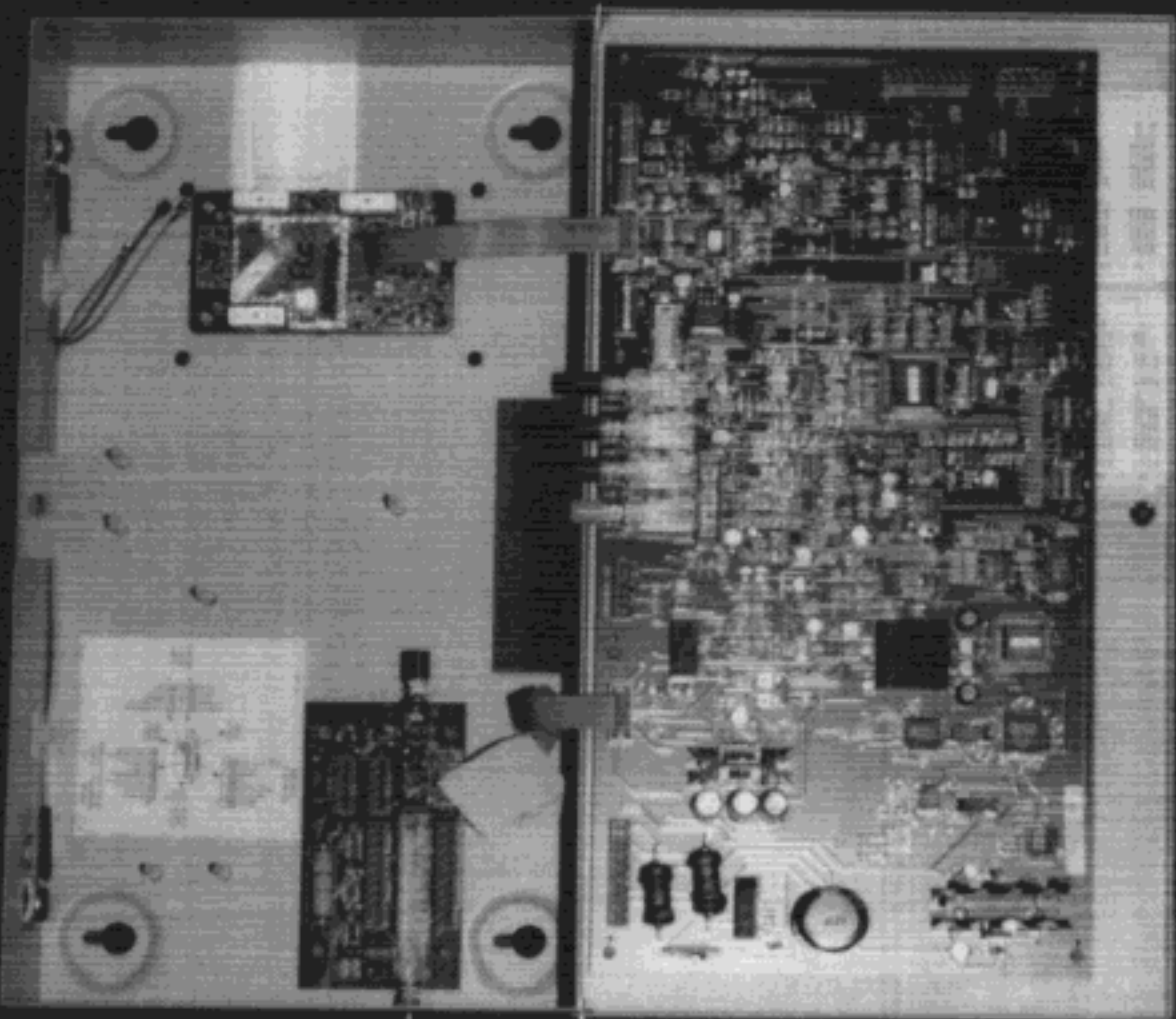
Figure A5 SYS1000A Base Interior with boards in place (BYMB1K)
