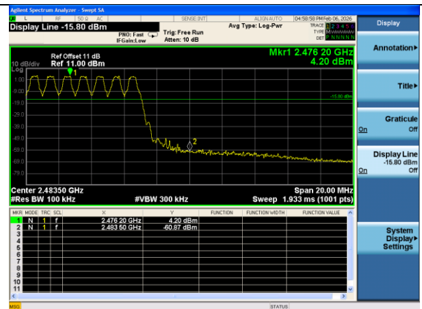
BT-GFSK-Band Edge-High-Hopping
