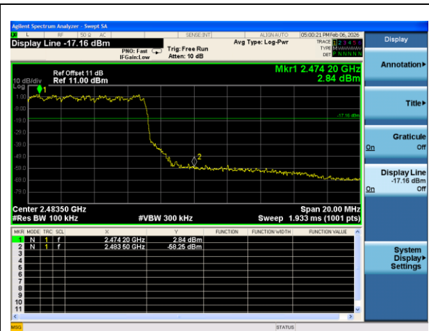
BT-8DPSK-Band Edge-High-Hopping
