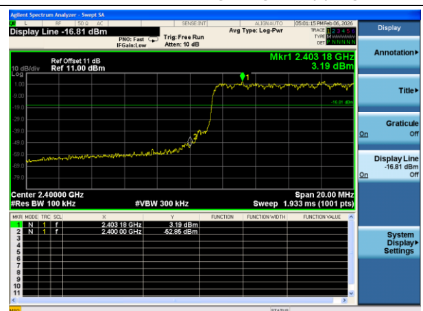
BT-8DPSK-Band Edge-Low-Hopping
