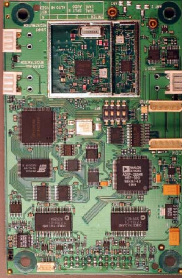
BS200 XCVR Board Top View wo/Shield
