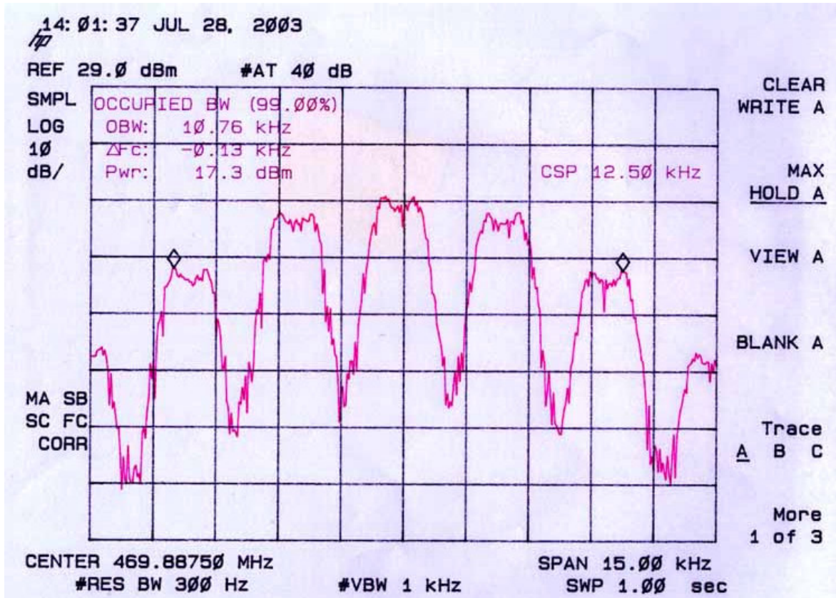
Figure 1 COM400 Modulated with 2500Hz + 16 dB
