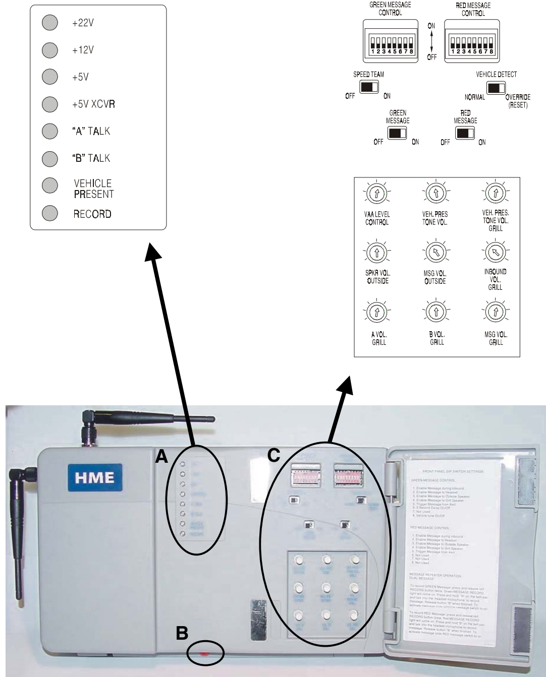
Figure 2. Wireless 6000 Base Station with cabinet door open
