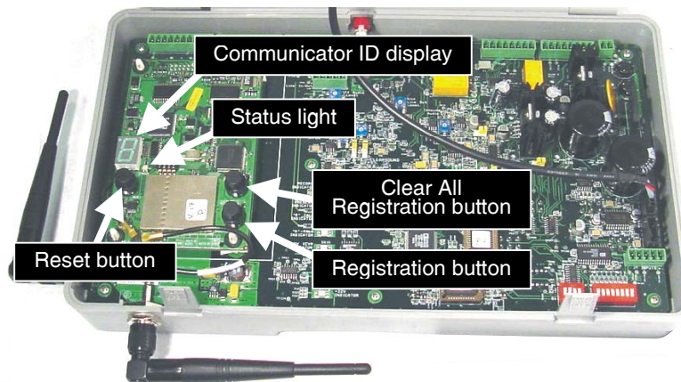
Figure 5. Registration buttons and indicators
