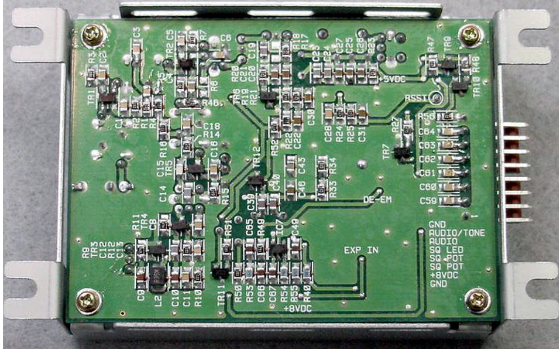
RX MODULE BOTTOM WITHOUT SHIELD FILE: RX MODULE BOTTOM WITHOUT SHIELD.JPG
