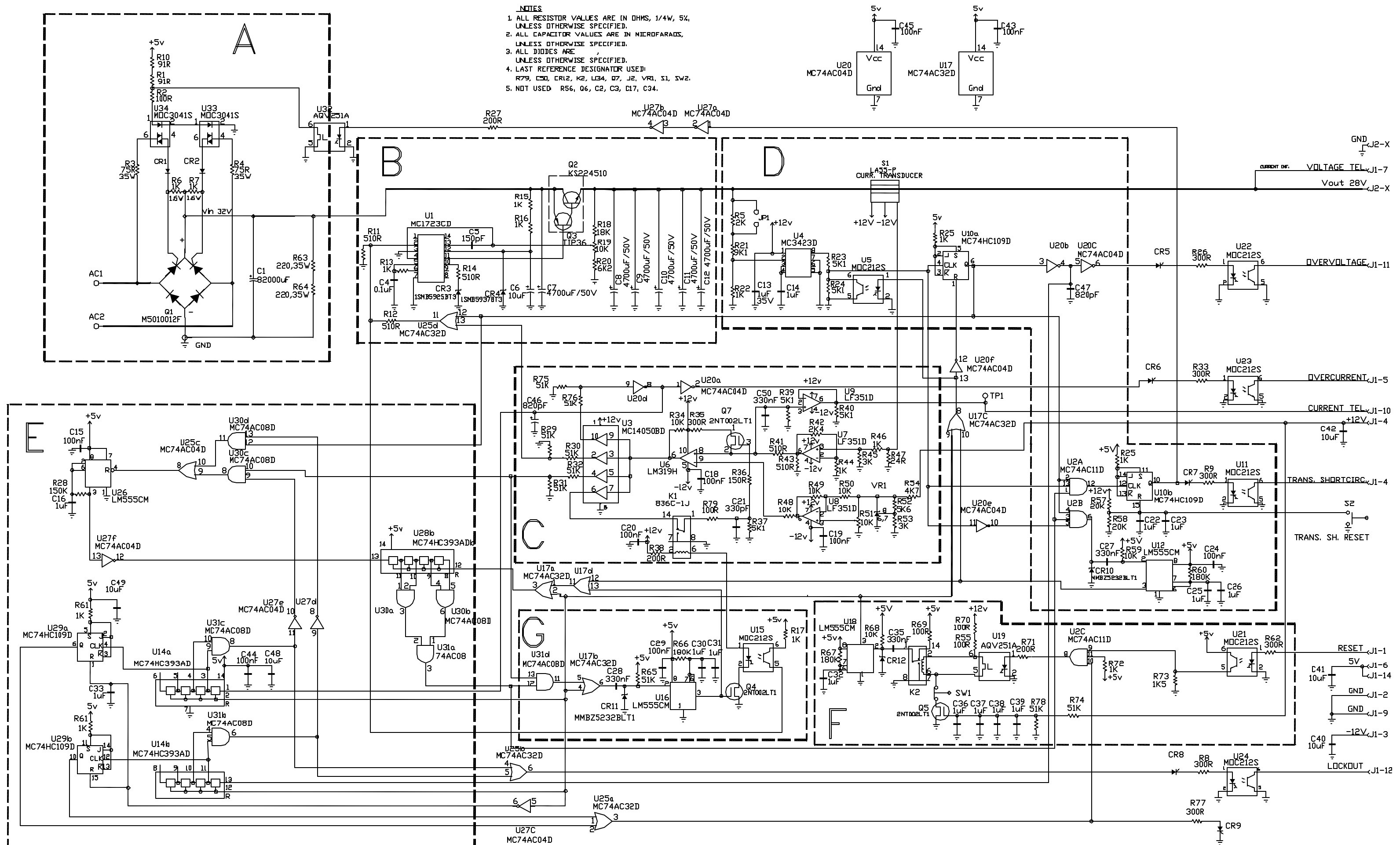
41D1680S Figure 4 SCH. - LIN. REGULATOR
