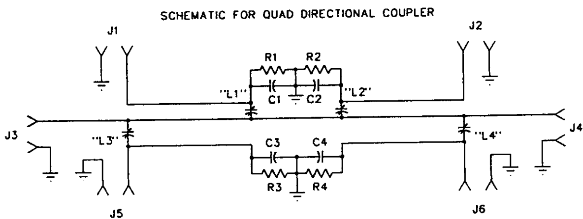
Figure 3: Quad Directional Coupler equivalent Schematic.
