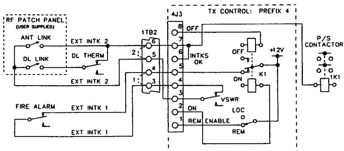
Figure 1: TTS10B and TTS50B Transmitter Interlock Connections.
