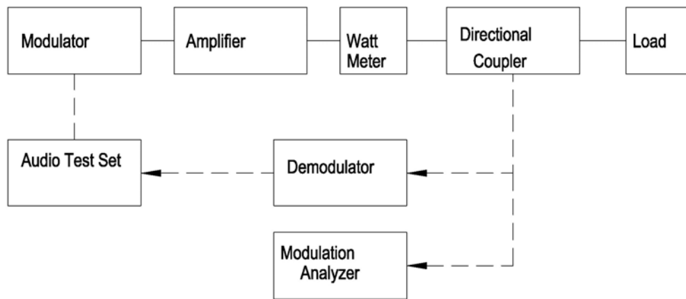
Video Test Setup
