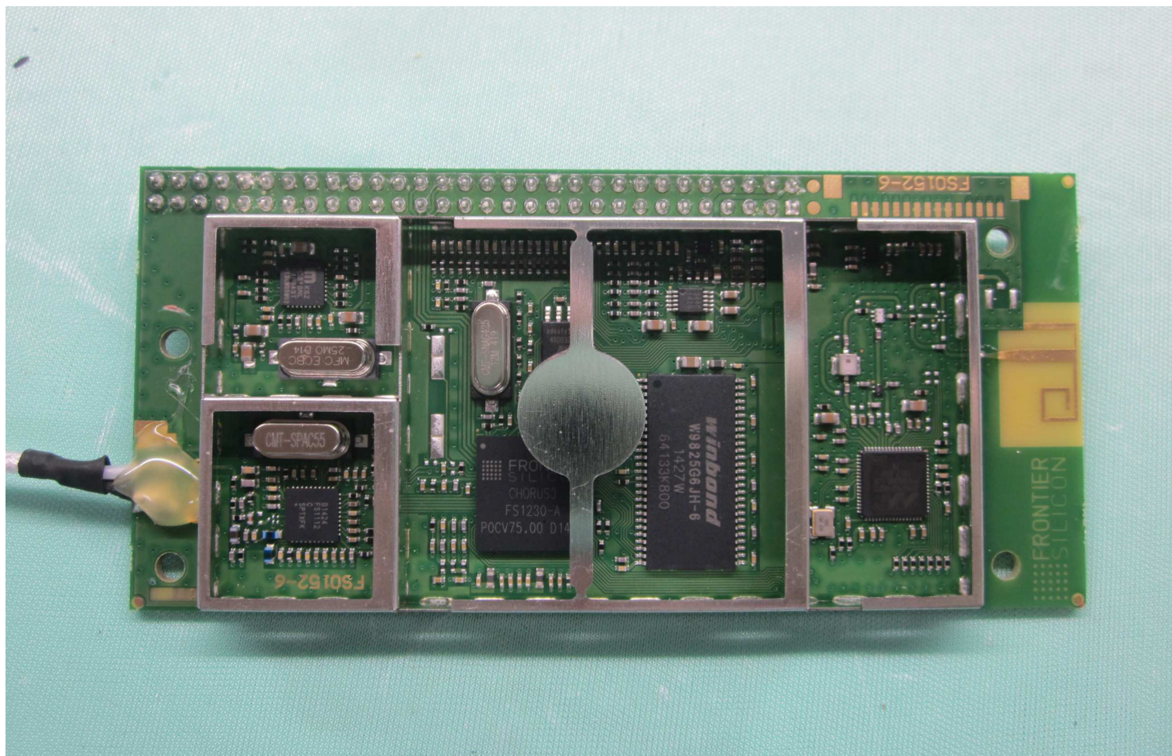
FCC ID: BZAWDFB0920H3 PHOTOGRAPH OF THE PRODUCT
