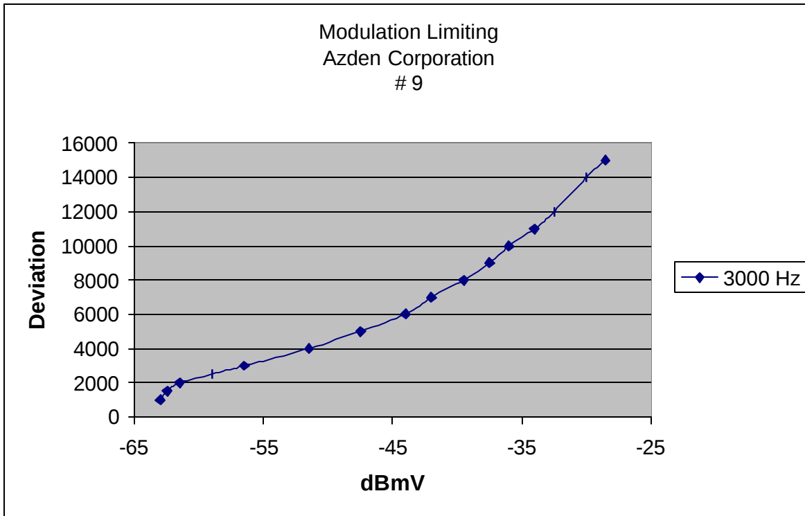
Modulation Limiting Plot 3000 Hz
