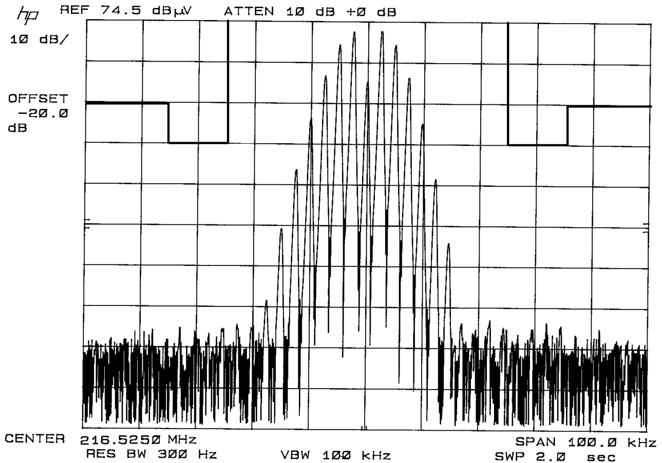
Occupied Bandwidth Plot 50 kHz channel
