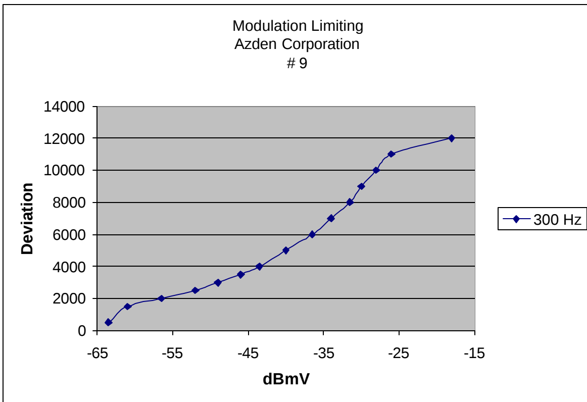
Modulation limiting 300 Hz
