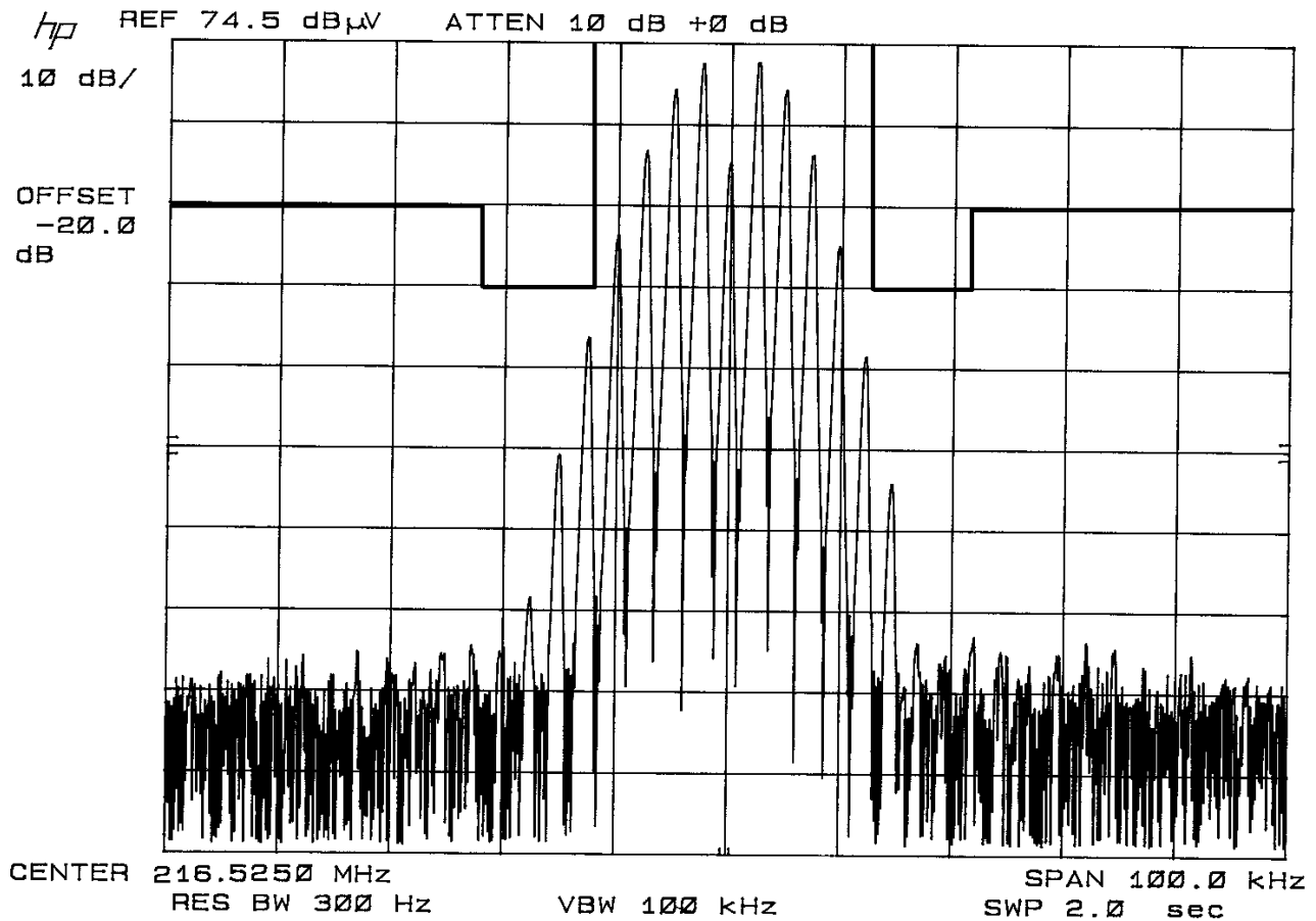
Occupied Bandwidth Plot 25 kHz channel
