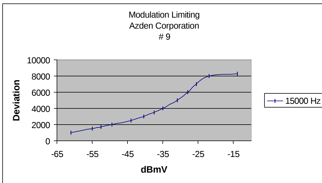
Modulation Limiting Plot 15000 Hz
