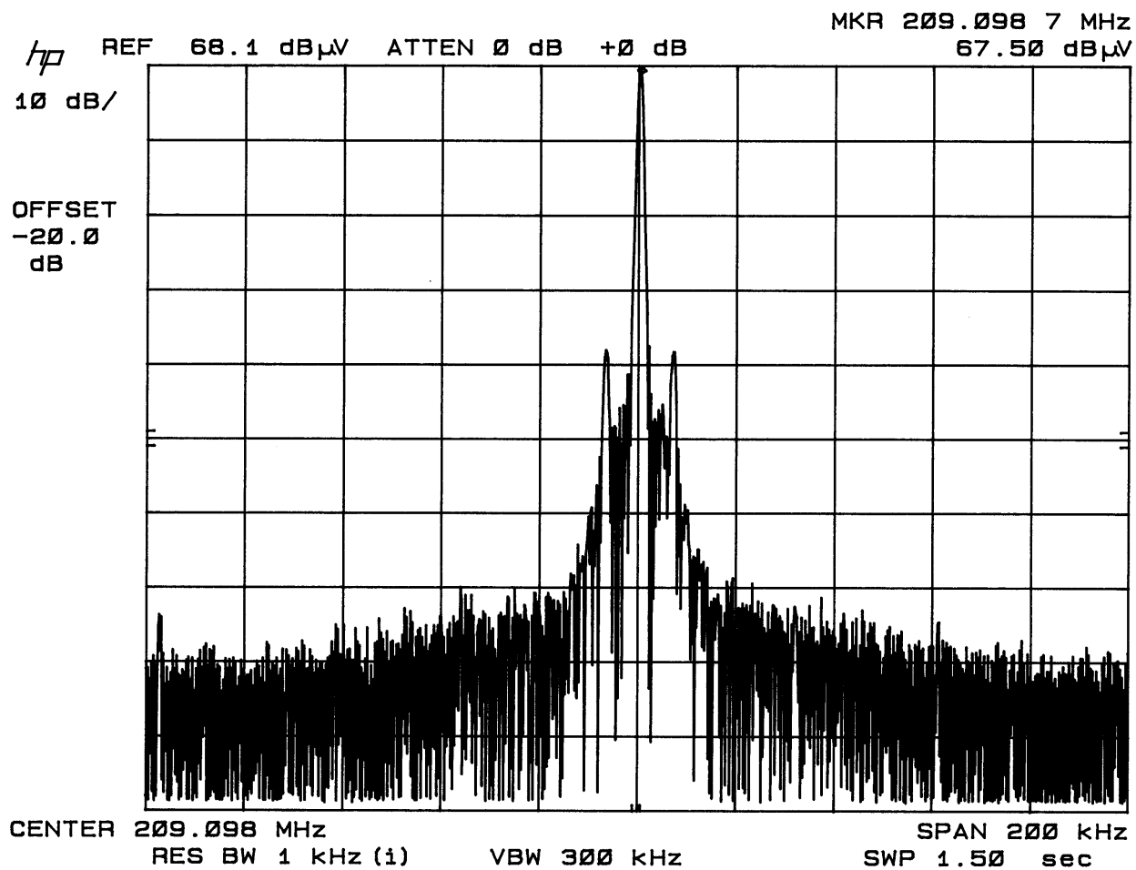
Occupied BW CW Plot
