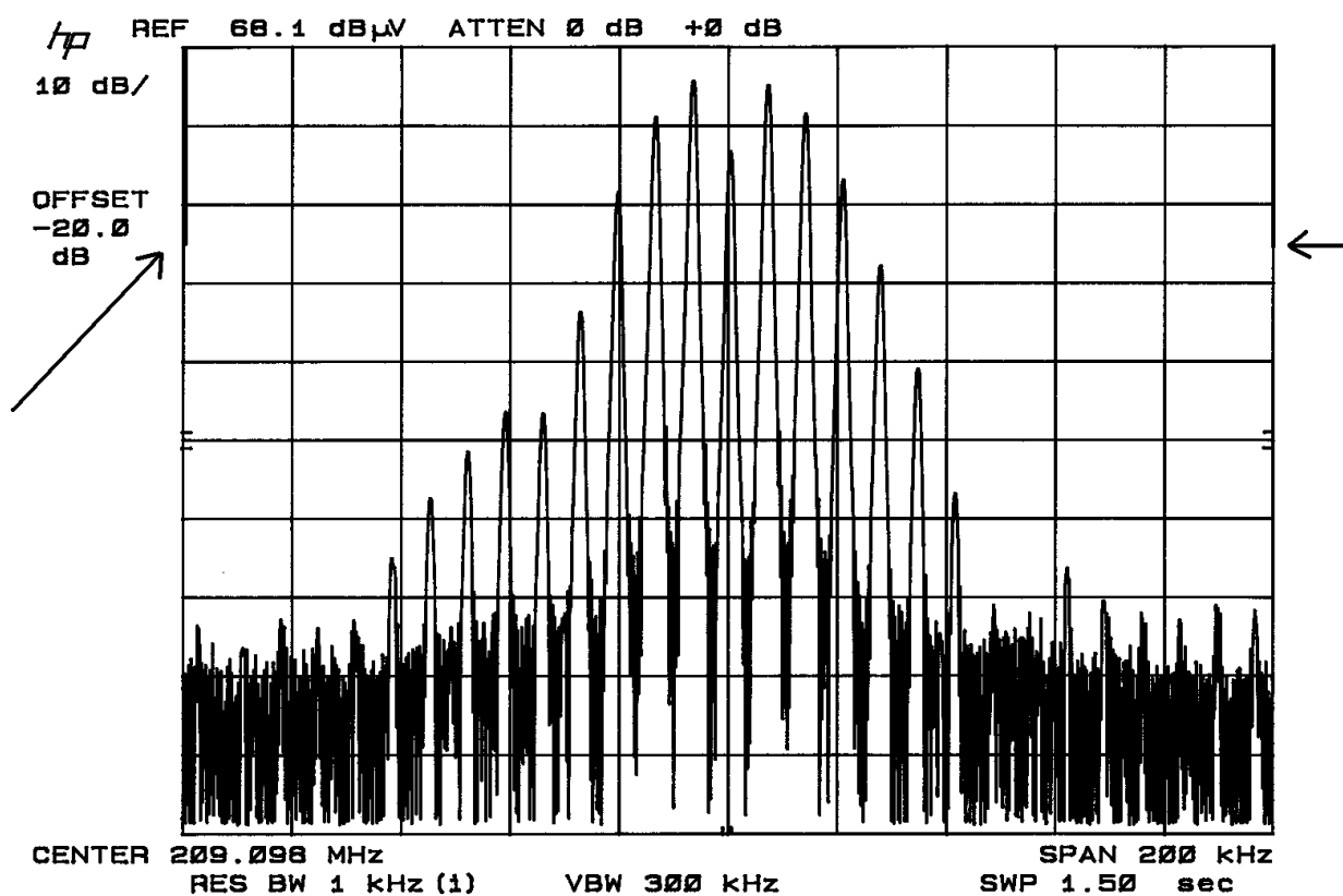
Occupied BW Plot
