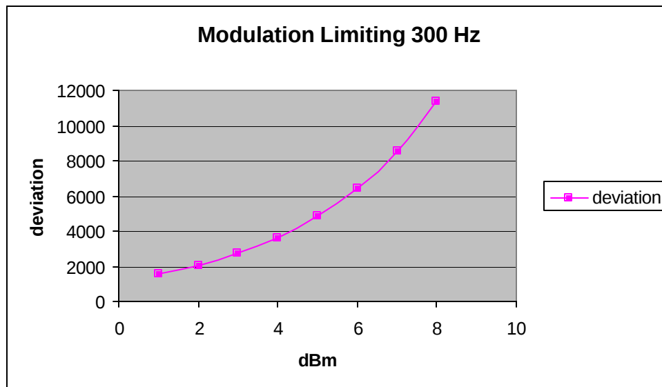
MODULATION LIMITING GRAPH - 300 Hz
