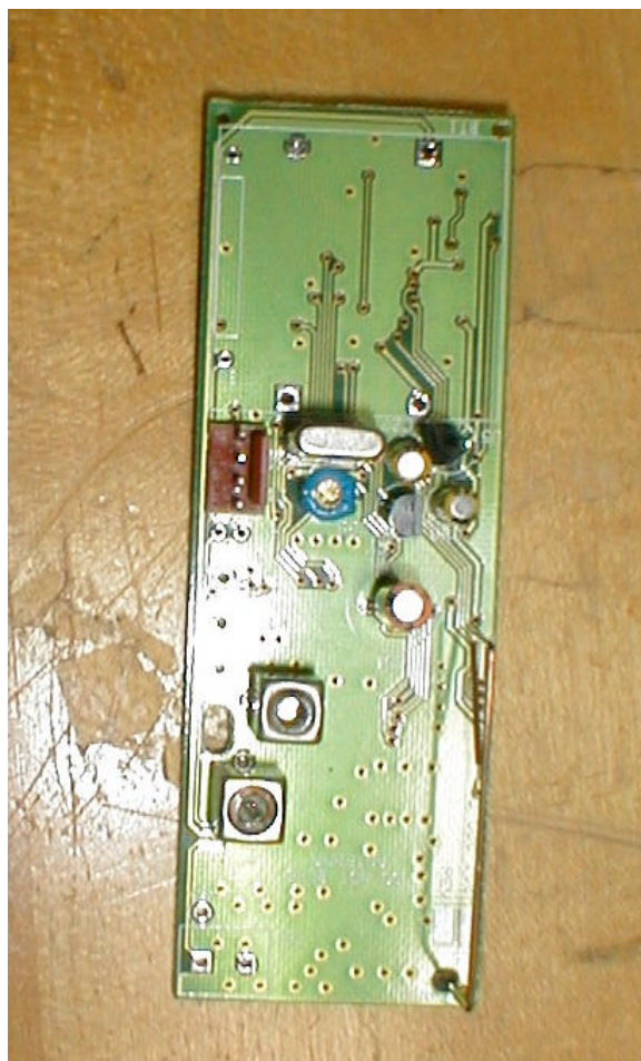
PCB Top View
