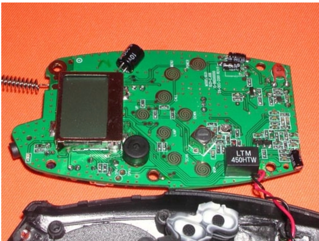
Internal Photo - 4
