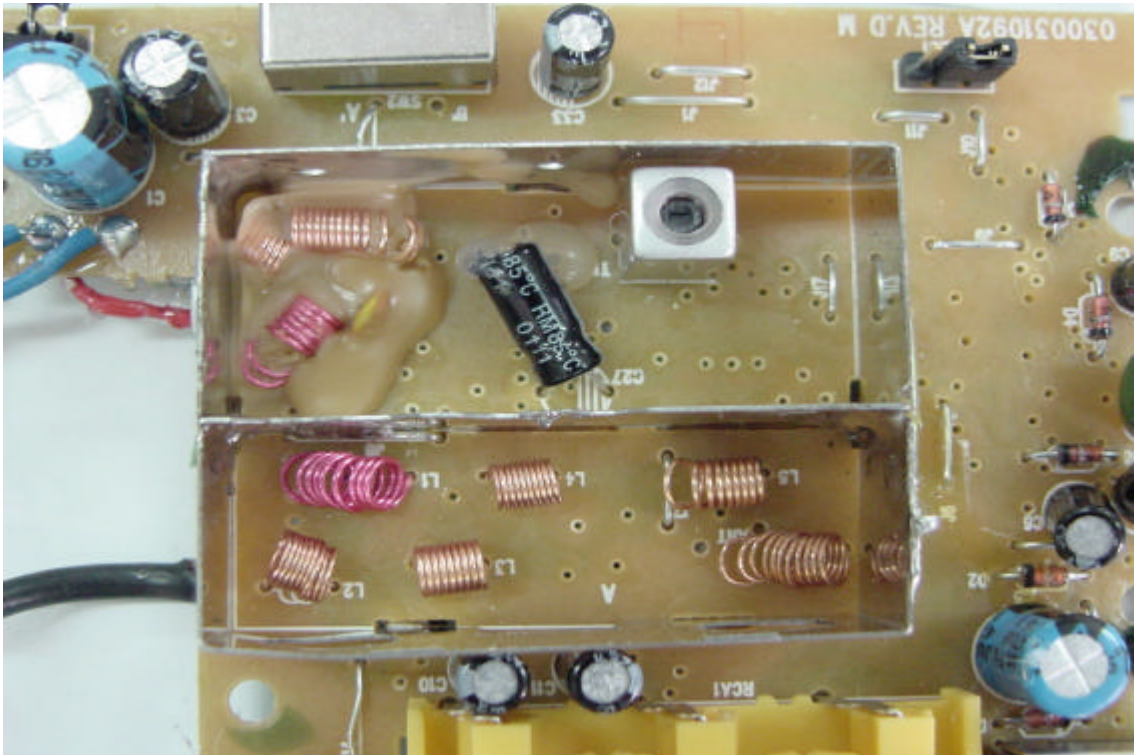
Component View of Tuner PCB
