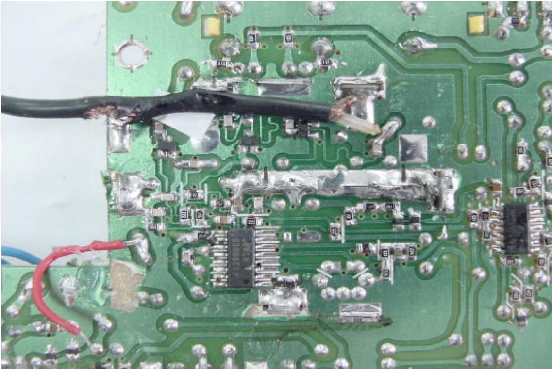
Solder View of Tuner PCB
