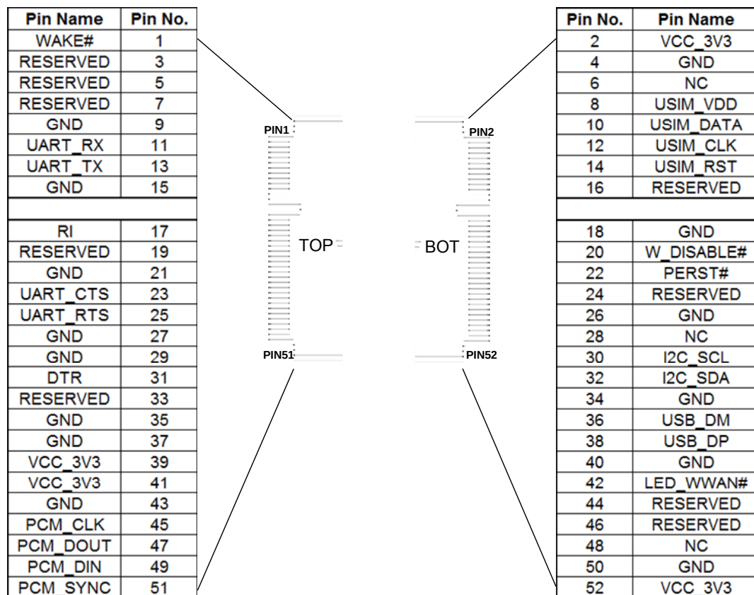
Figure 2: Pin Assignment
