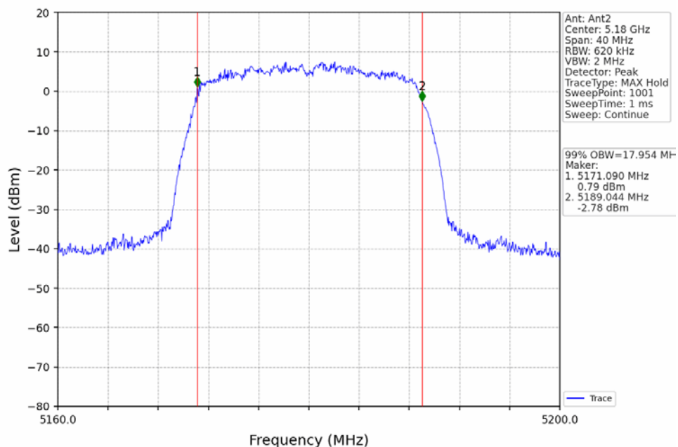
802.11ac(VHT20)_LCH_5180MHz_Ant2_NTNV
