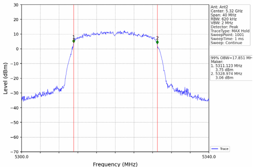
802.11ac(VHT20)_HCH_5320MHz_Ant2_NTNV
