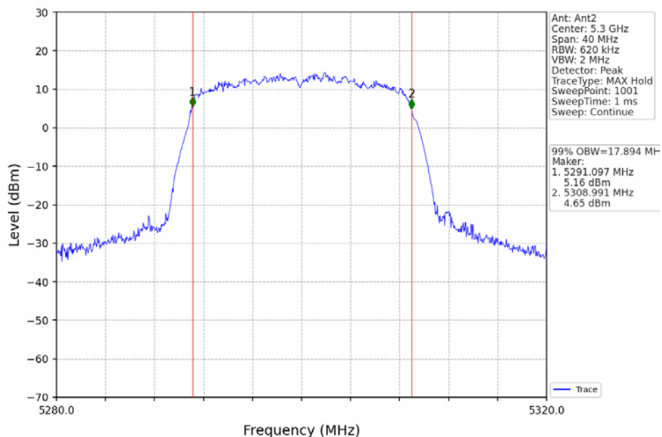
802.11ac(VHT20)_MCH_5300MHz_Ant2_NTNV
