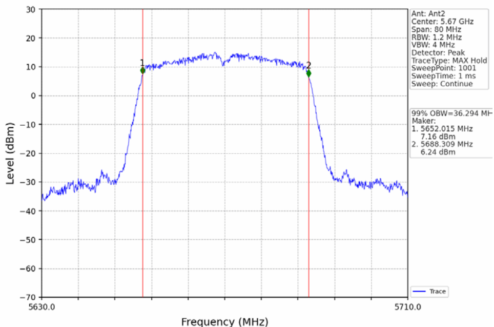
802.11n(HT40)_HCH_5670MHz_Ant2_NTNV
