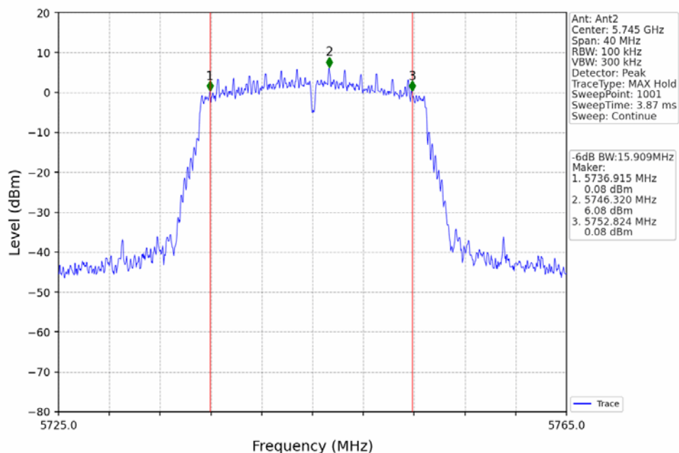
802.11ac(VHT20)_LCH_5745MHz_Ant2_NTNV
