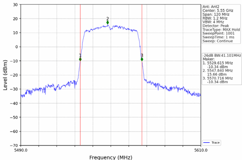
802.11n(HT40)_MCH_5550MHz_Ant2_NTNV
