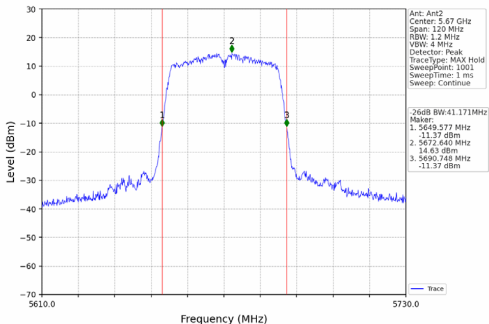
802.11n(HT40)_HCH_5670MHz_Ant2_NTNV
