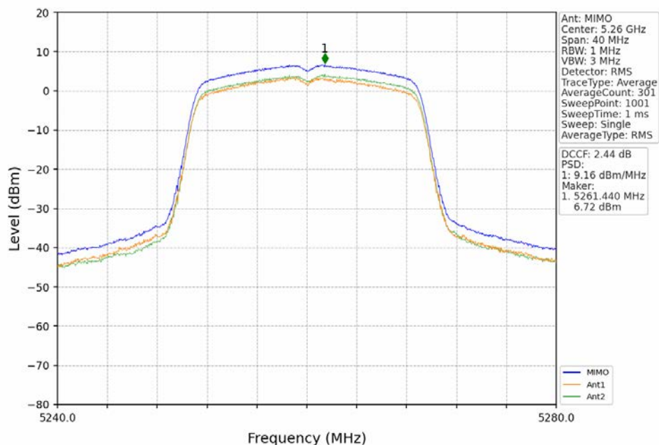
802.11ac(VHT20)_LCH_5260MHz_MIMO_NTNV
