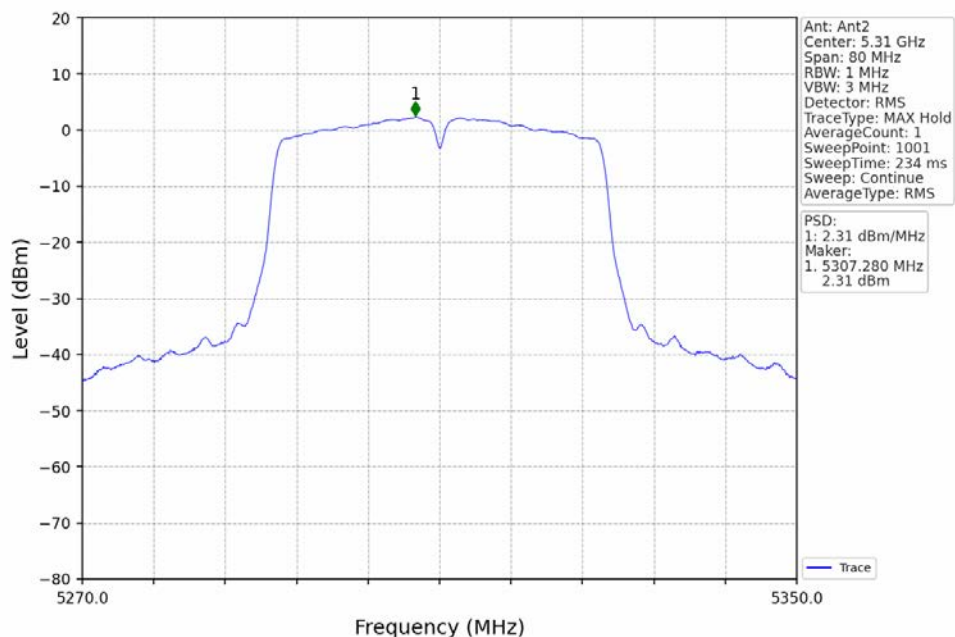
802.11n(HT40)_HCH_5310MHz_Ant2_NTNV
