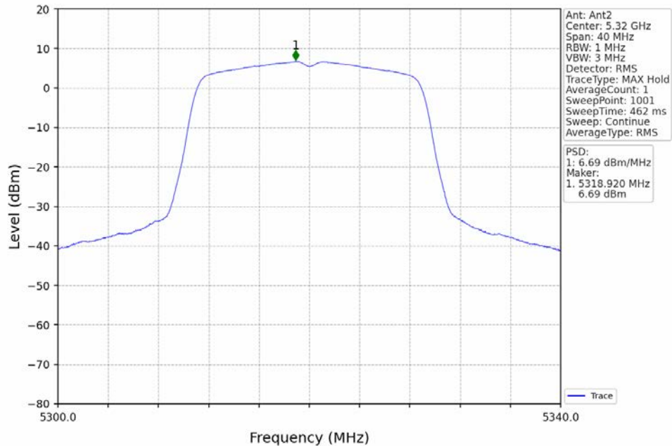
802.11ac(VHT20)_HCH_5320MHz_MIMO_NTNV
