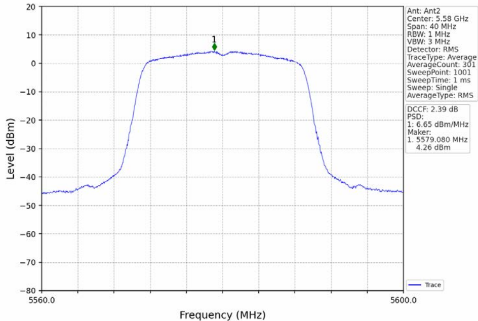
802.11ac(VHT20)_MCH_5580MHz_MIMO_NTNV
