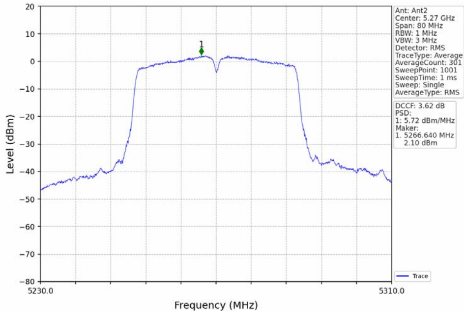
802.11ac(VHT40)_LCH_5270MHz_MIMO_NTNV
