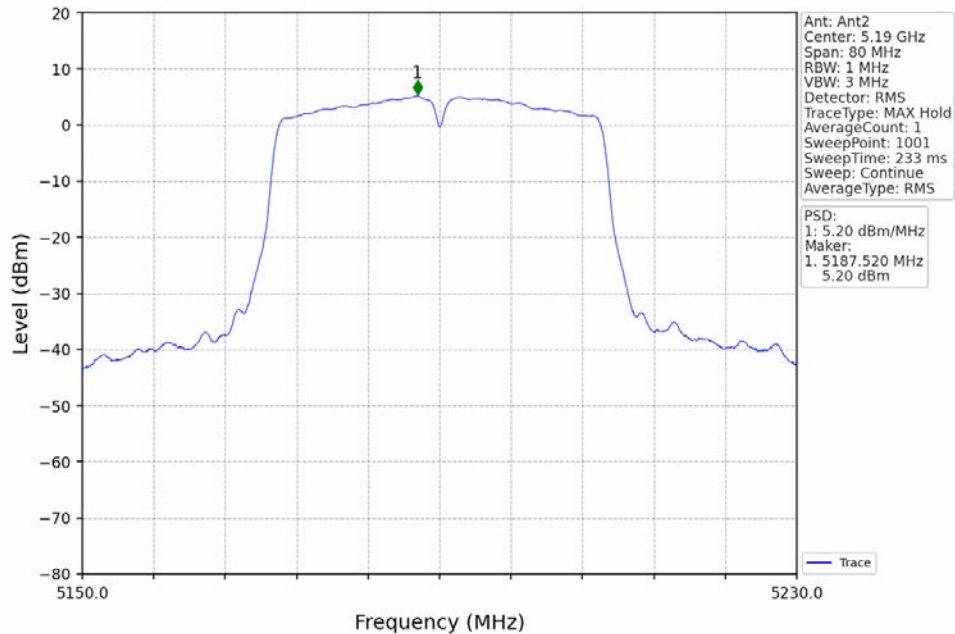
802.11n(HT40)_LCH_5190MHz_MIMO_NTNV
