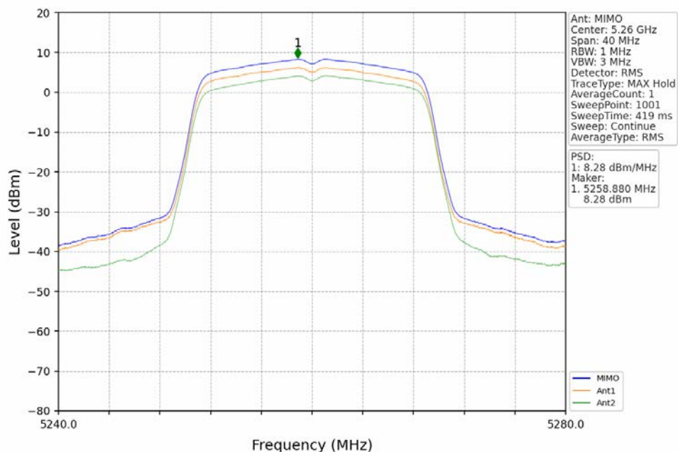
802.11n(HT20)_LCH_5260MHz_MIMO_NTNV
