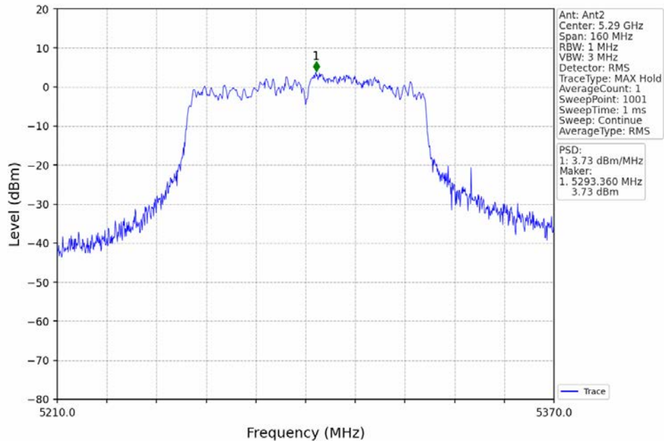
802.11ac(VHT80)_MCH_5290MHz_MIMO_NTNV
