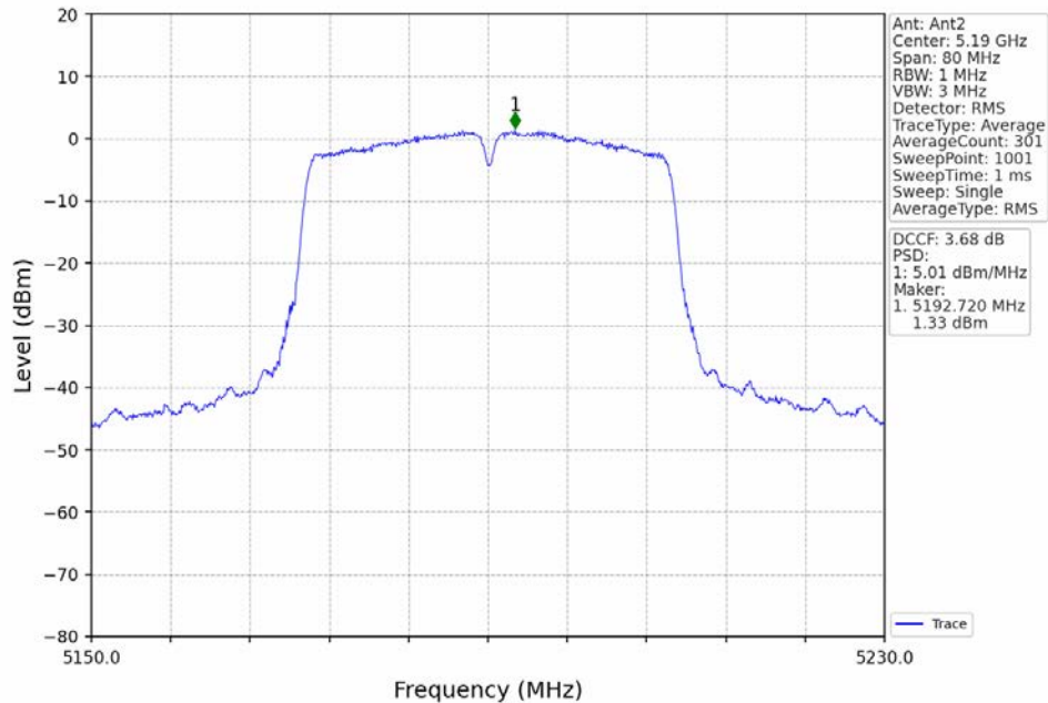
802.11ac(VHT40)_LCH_5190MHz_MIMO_NTNV
