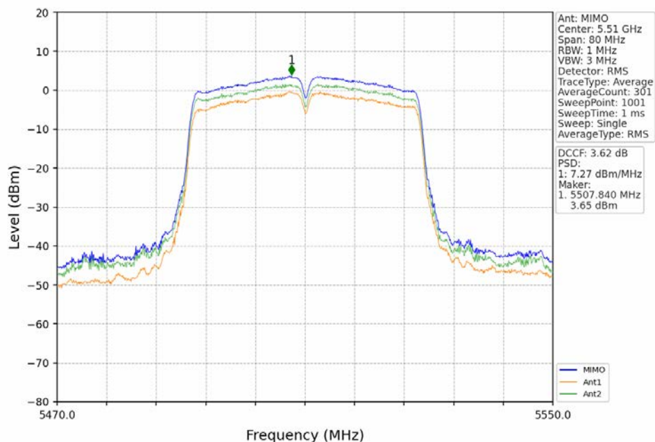
802.11ac(VHT40)_LCH_5510MHz_MIMO_NTNV
