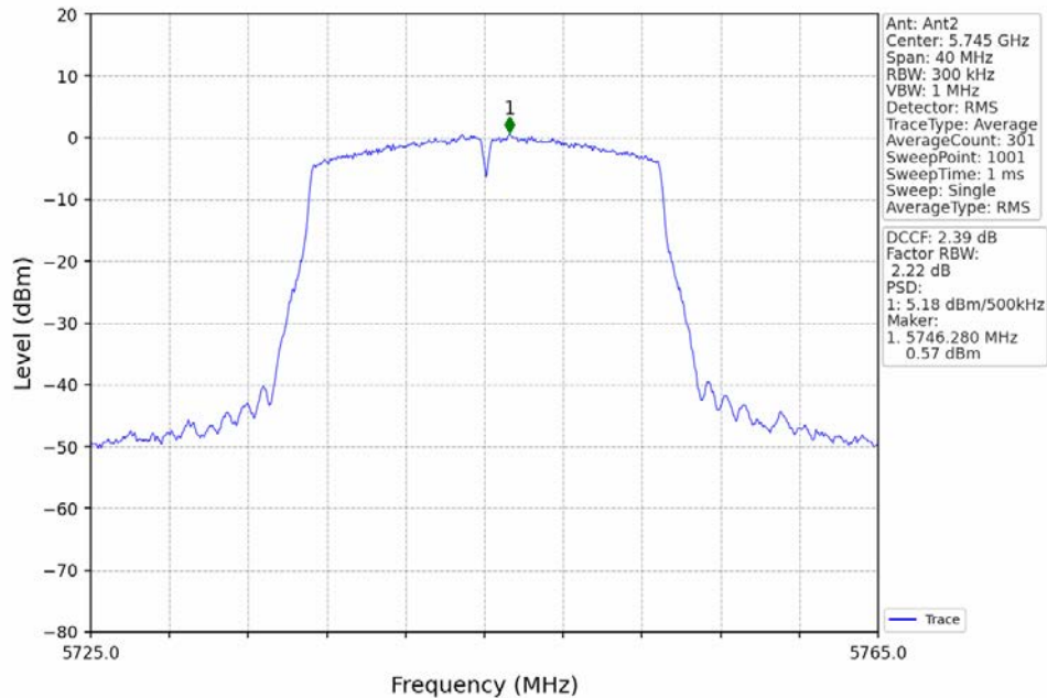
802.11ac(VHT20)_LCH_5745MHz_MIMO_NTNV
