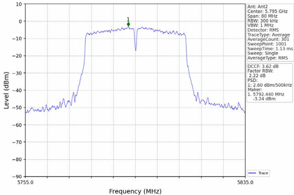
802.11ac(VHT40)_HCH_5795MHz_MIMO_NTNV
