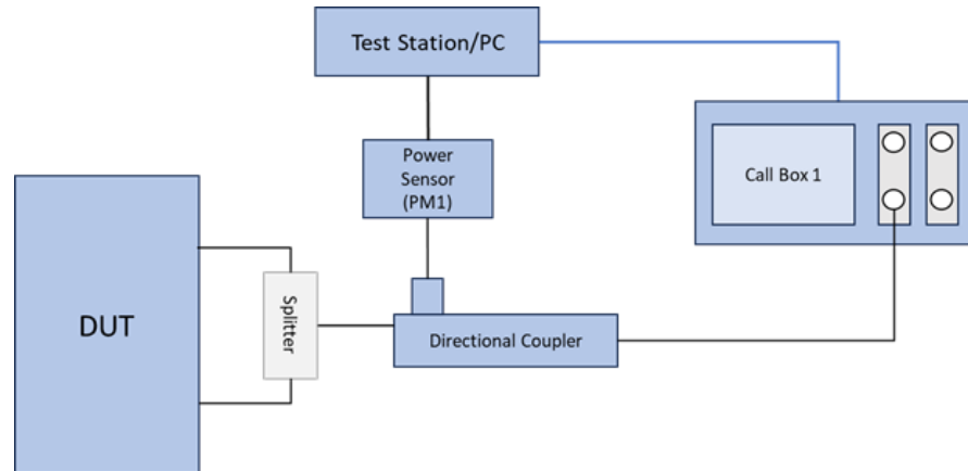
(b) Appendix D – Test Setup Photo 1, 2
