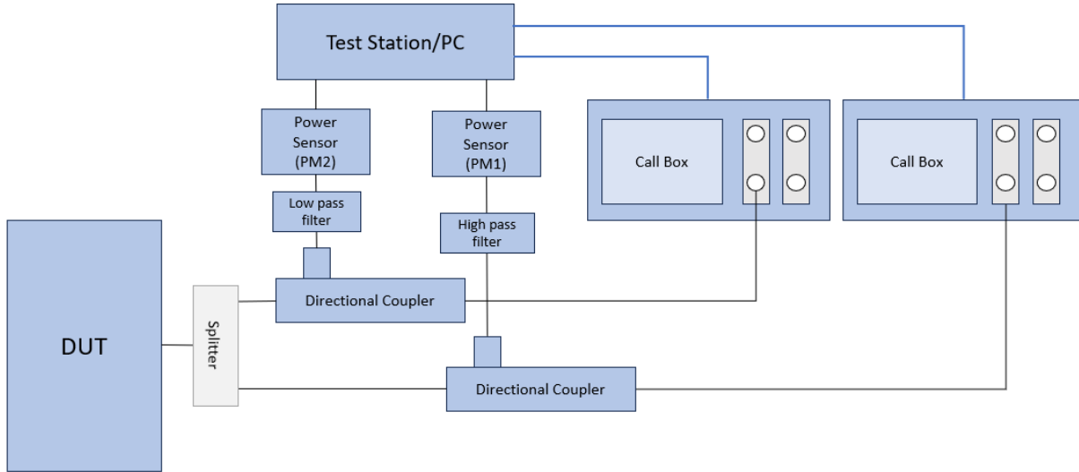
(c) Appendix D – Test Setup Photo 4
