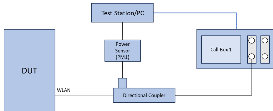
(a) Appendix D – Test Setup Photo 1, 2
