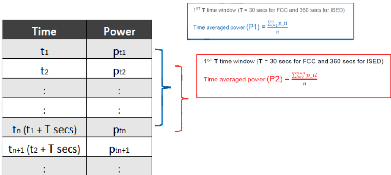
Figure 4-3 Time running/moving average illustration
