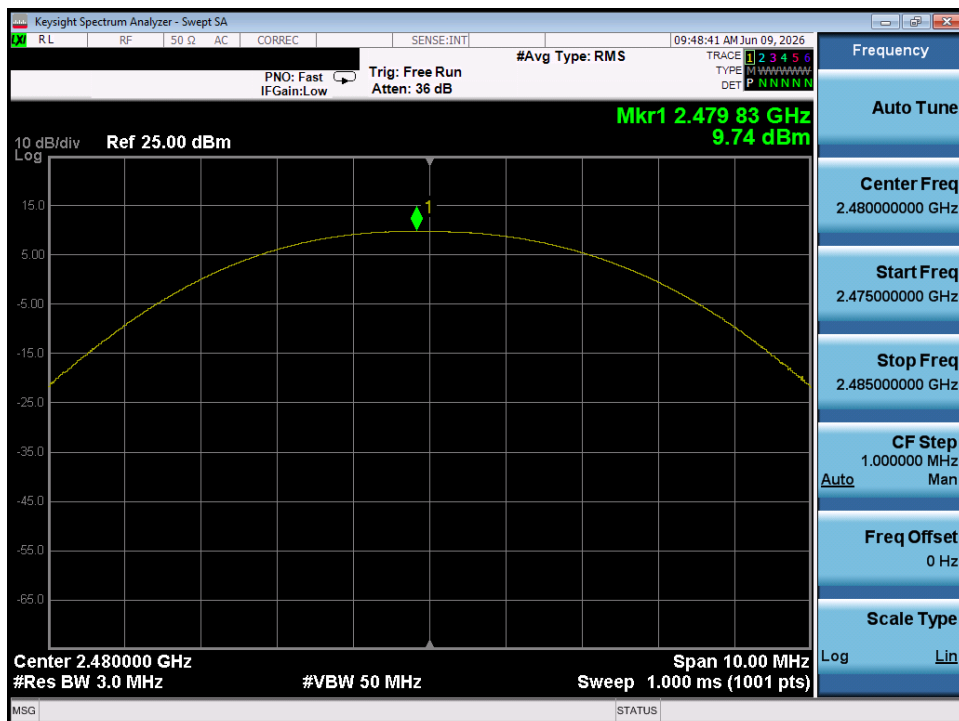
Plot 7-27. Peak Power Plot (Bluetooth (LE), 125kbps – Ch. 39) – Dual Chain 0
