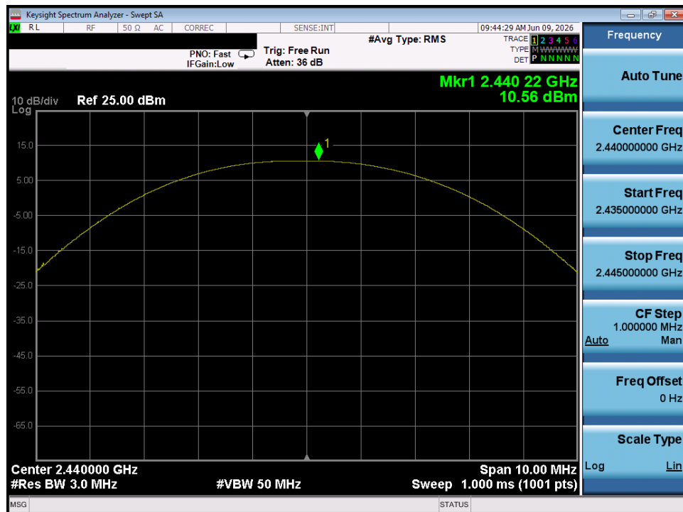
Plot 7-38. Peak Power Plot (Bluetooth (LE), 125kbps – Ch. 17) – Dual Chain 1
