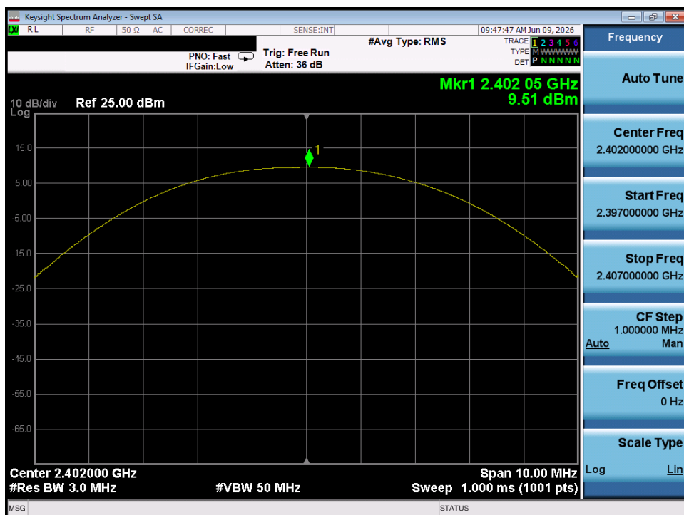
Plot 7-25. Peak Power Plot (Bluetooth (LE), 125kbps – Ch. 37) – Dual Chain 0
