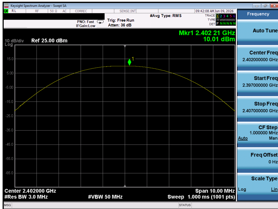
Plot 7-37. Peak Power Plot (Bluetooth (LE), 125kbps – Ch. 37) – Dual Chain 1
