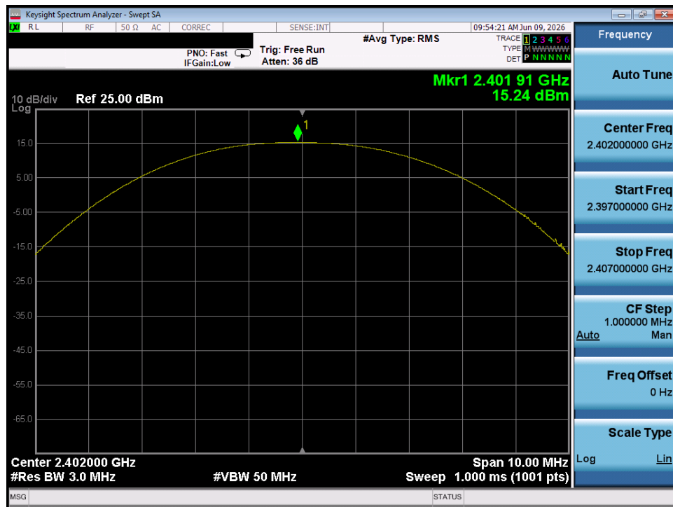
Plot 7-16. Peak Power Plot (Bluetooth (LE), 500kbps – Ch. 37) – Chain 1
