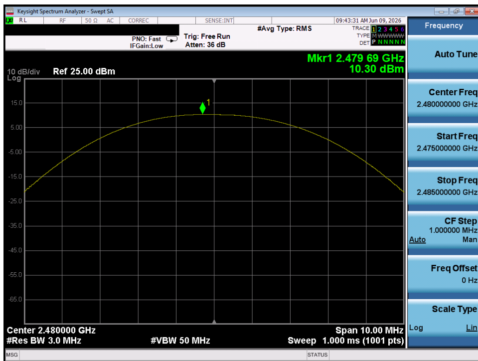
Plot 7-42. Peak Power Plot (Bluetooth (LE), 500kbps – Ch. 39) – Dual Chain 1
