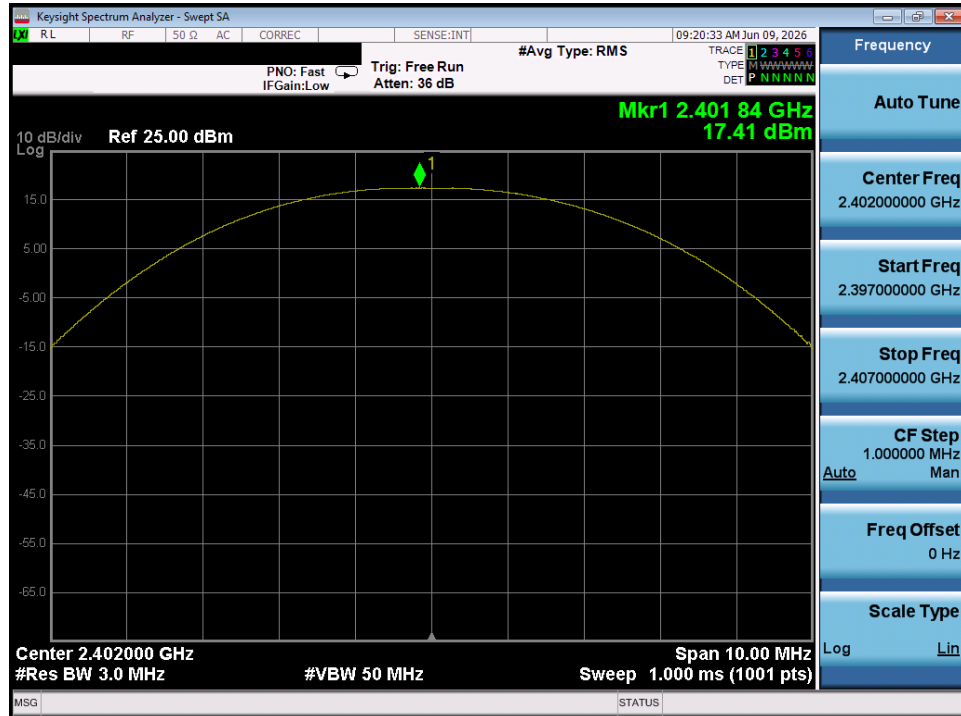
Plot 7-7. Peak Power Plot (Bluetooth (LE), 1Mbps – Ch. 37) – Chain 0
