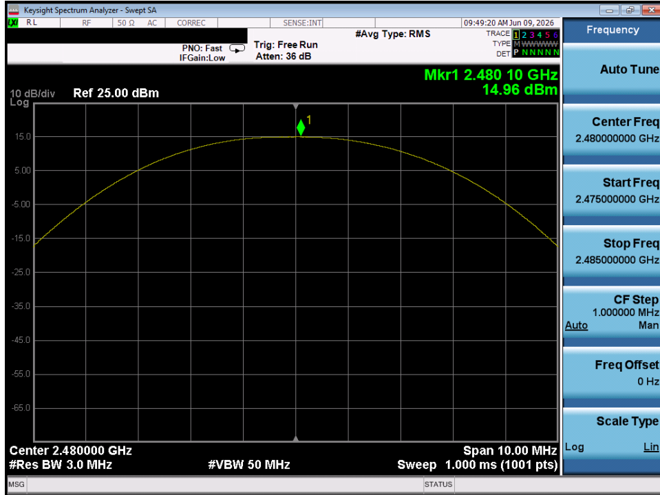
Plot 7-3. Peak Power Plot (Bluetooth (LE), 125kbps – Ch. 39) – Chain 0
