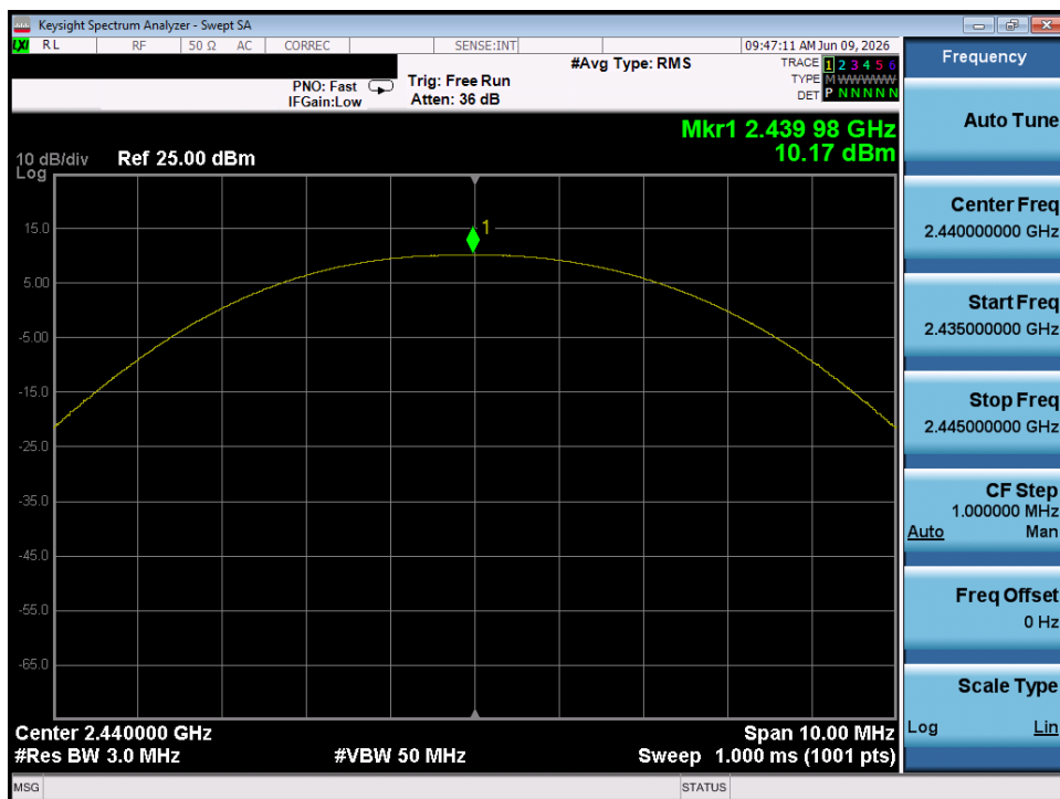
Plot 7-26. Peak Power Plot (Bluetooth (LE), 125kbps – Ch. 17) – Dual Chain 0
