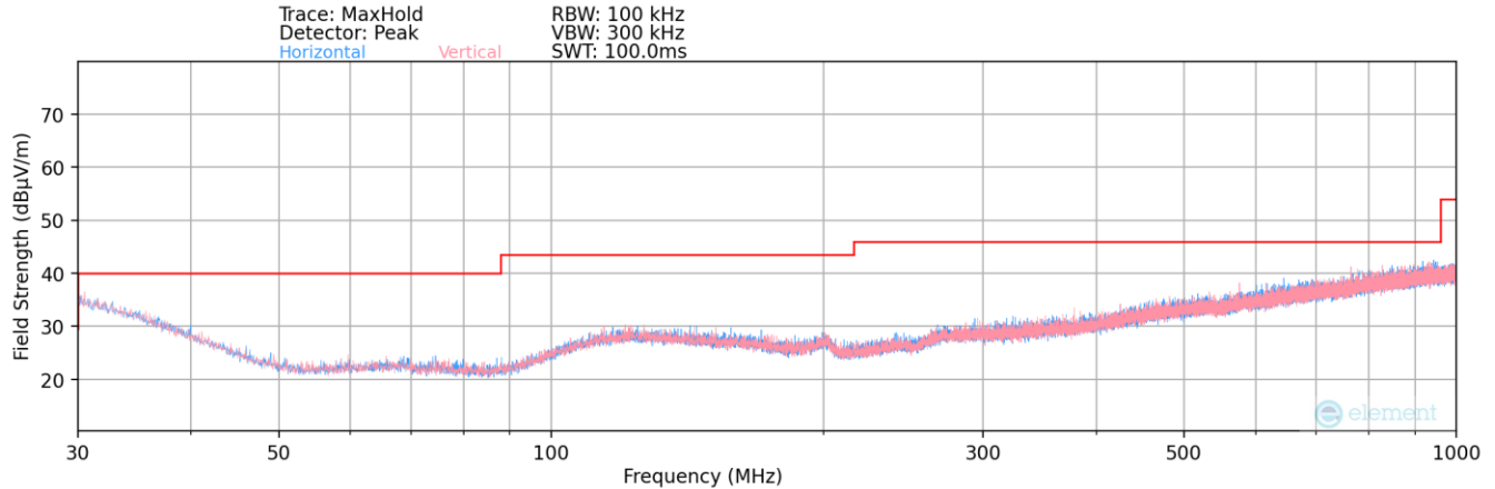
Plot 7-49. Radiated Spurious Plot below 1GHz (Bluetooth (LE))
