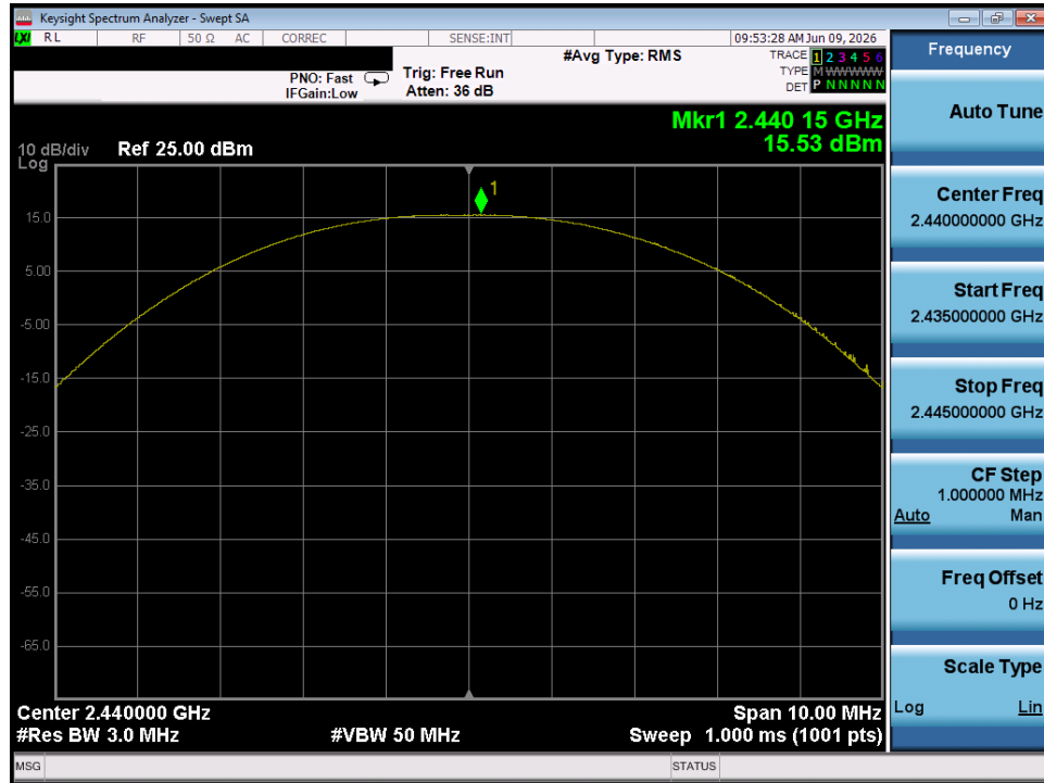
Plot 7-17. Peak Power Plot (Bluetooth (LE), 500kbps – Ch. 17) – Chain 1
