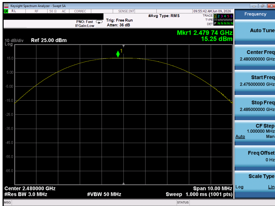
Plot 7-18. Peak Power Plot (Bluetooth (LE), 500kbps – Ch. 39) – Chain 1
