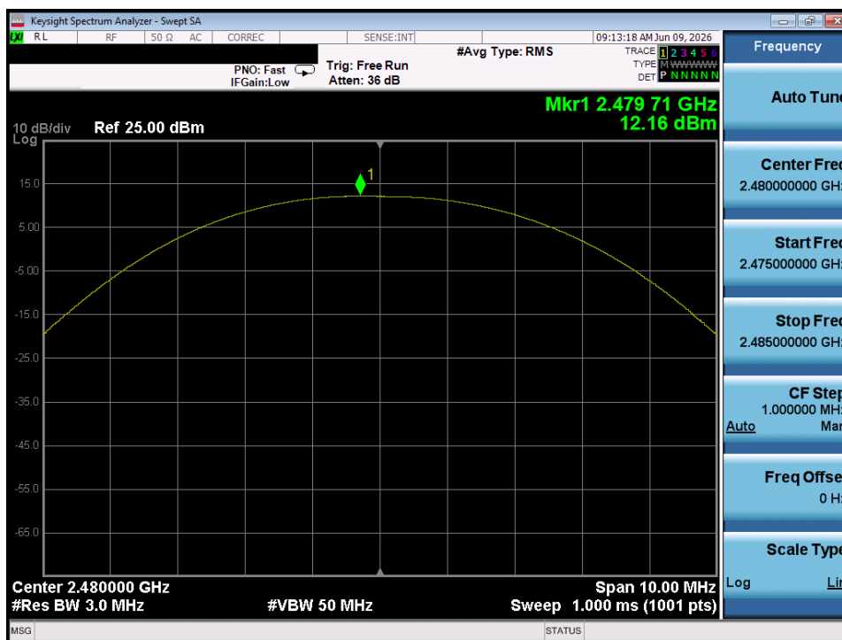
Plot 7-45. Peak Power Plot (Bluetooth (LE), 1Mbps – Ch. 39) – Dual Chain 1
