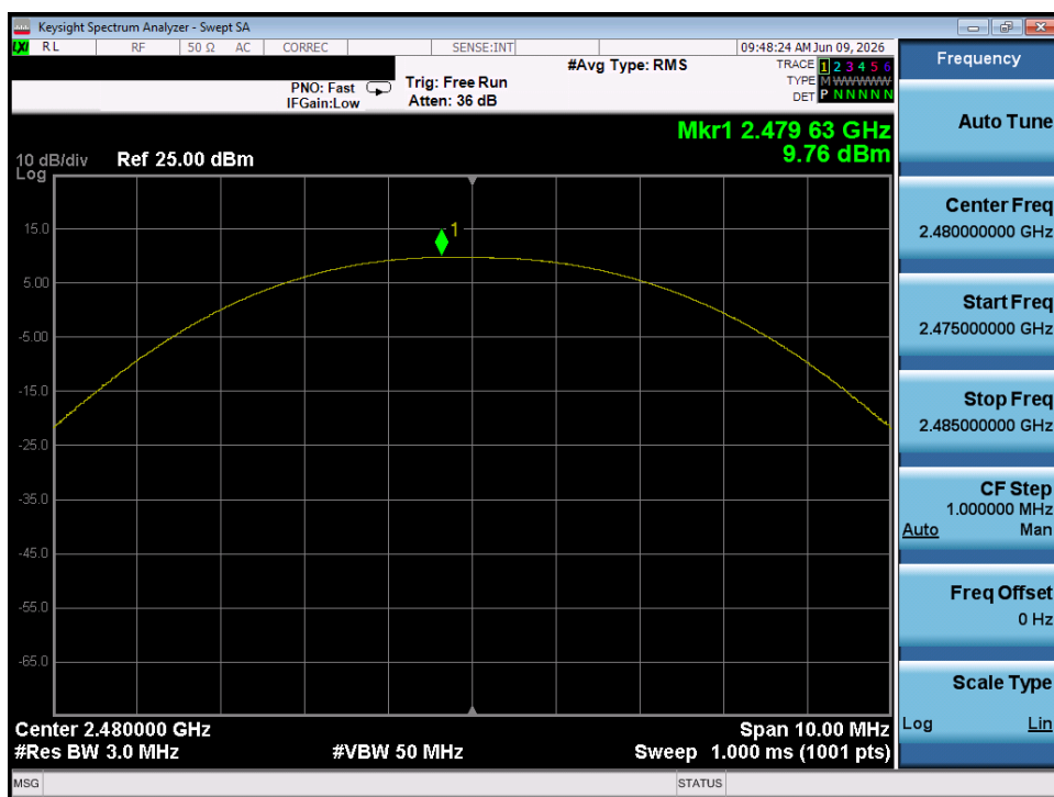
Plot 7-30. Peak Power Plot (Bluetooth (LE), 500kbps – Ch. 39) – Dual Chain 0
