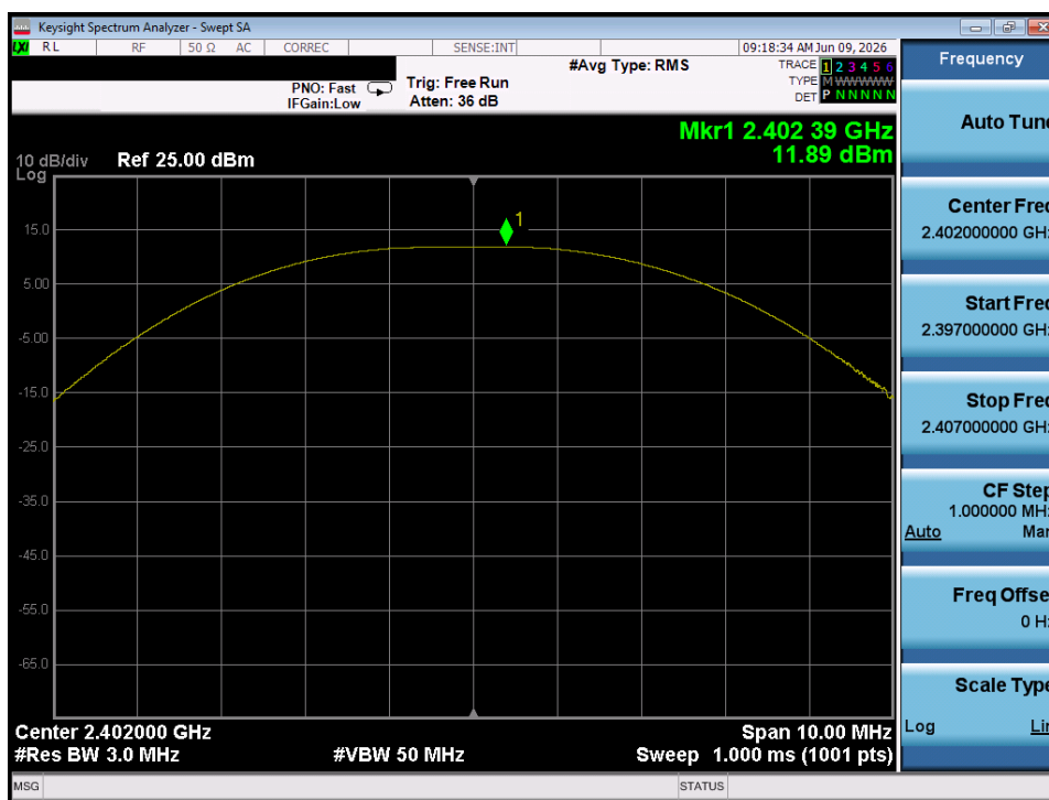
Plot 7-34. Peak Power Plot (Bluetooth (LE), 2Mbps - Ch. 0) - Dual Chain 0
