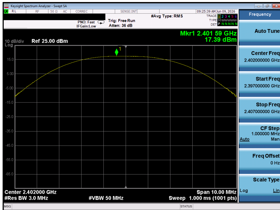
Plot 7-22. Peak Power Plot (Bluetooth (LE), 2Mbps – Ch. 0) – Chain 1
