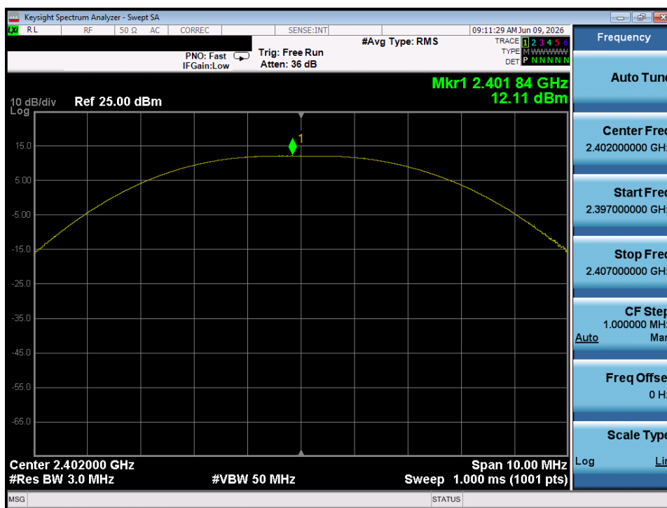
Plot 7-46. Peak Power Plot (Bluetooth (LE), 2Mbps – Ch. 0) – Dual Chain 1
