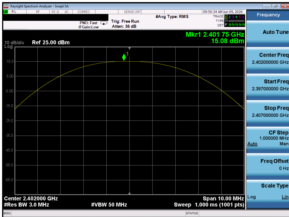
Plot 7-4. Peak Power Plot (Bluetooth (LE), 500kbps – Ch. 37) – Chain 0
