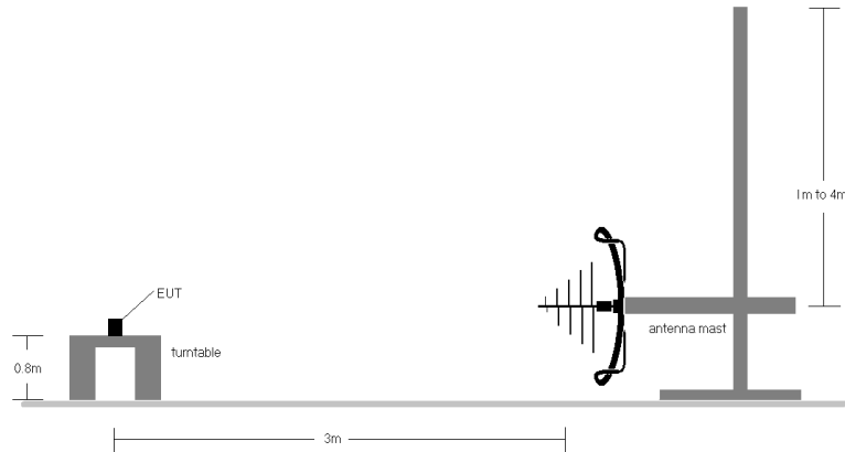
Figure 7-3. Radiated Test Setup < 1GHz
