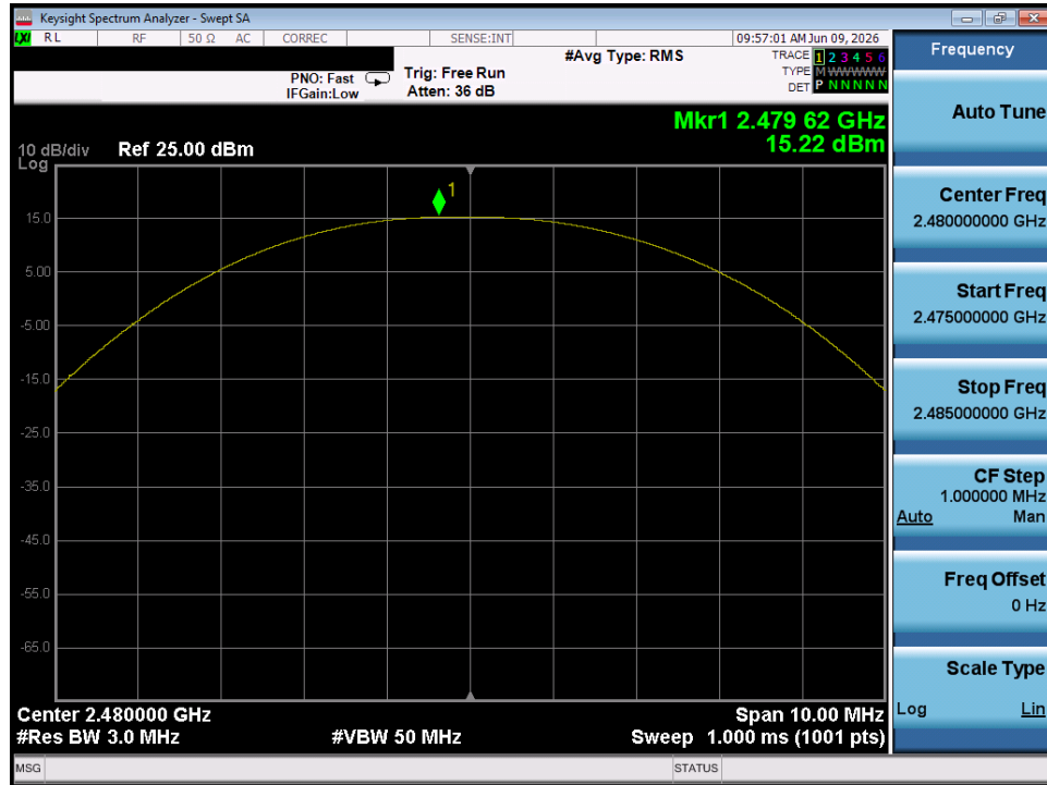
Plot 7-15. Peak Power Plot (Bluetooth (LE), 125kbps – Ch. 39) – Chain 1
