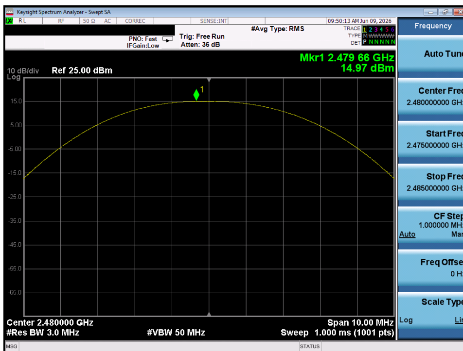
Plot 7-6. Peak Power Plot (Bluetooth (LE), 500kbps – Ch. 39) – Chain 0
