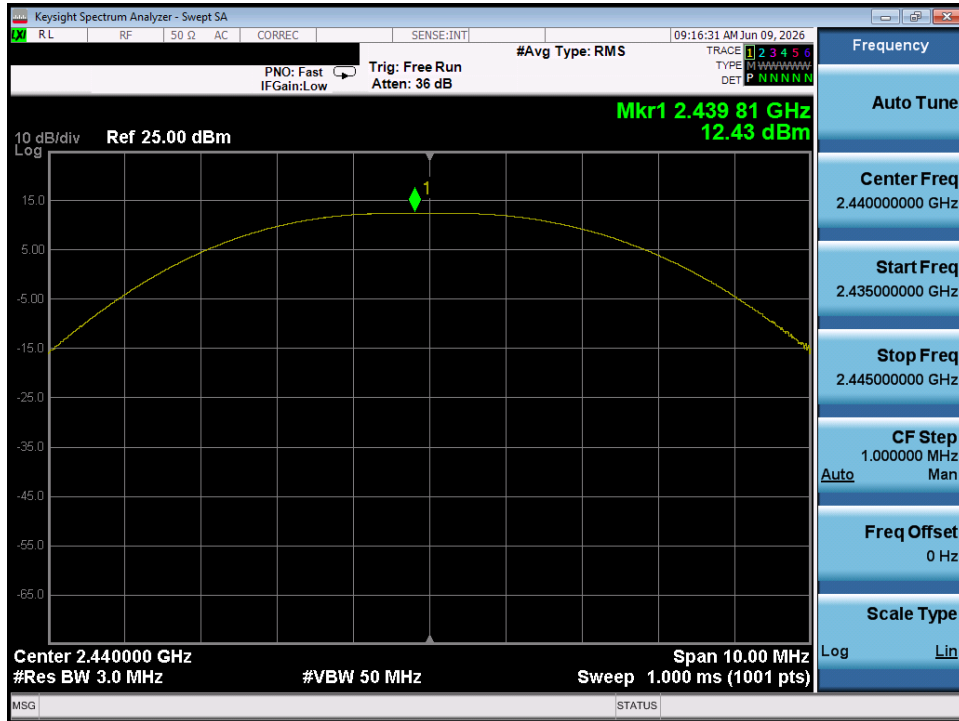
Plot 7-35. Peak Power Plot (Bluetooth (LE), 2Mbps - Ch. 17) - Dual Chain 0
