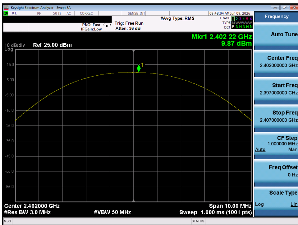
Plot 7-28. Peak Power Plot (Bluetooth (LE), 500kbps – Ch. 37) – Dual Chain 0
