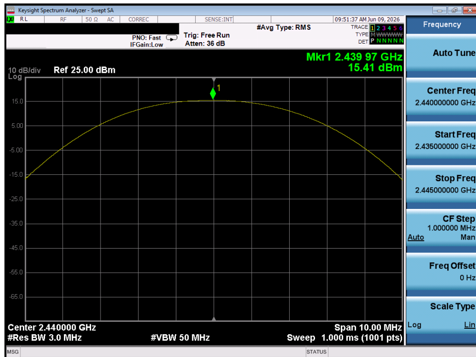
Plot 7-2. Peak Power Plot (Bluetooth (LE), 125kbps – Ch. 17) – Chain 0
