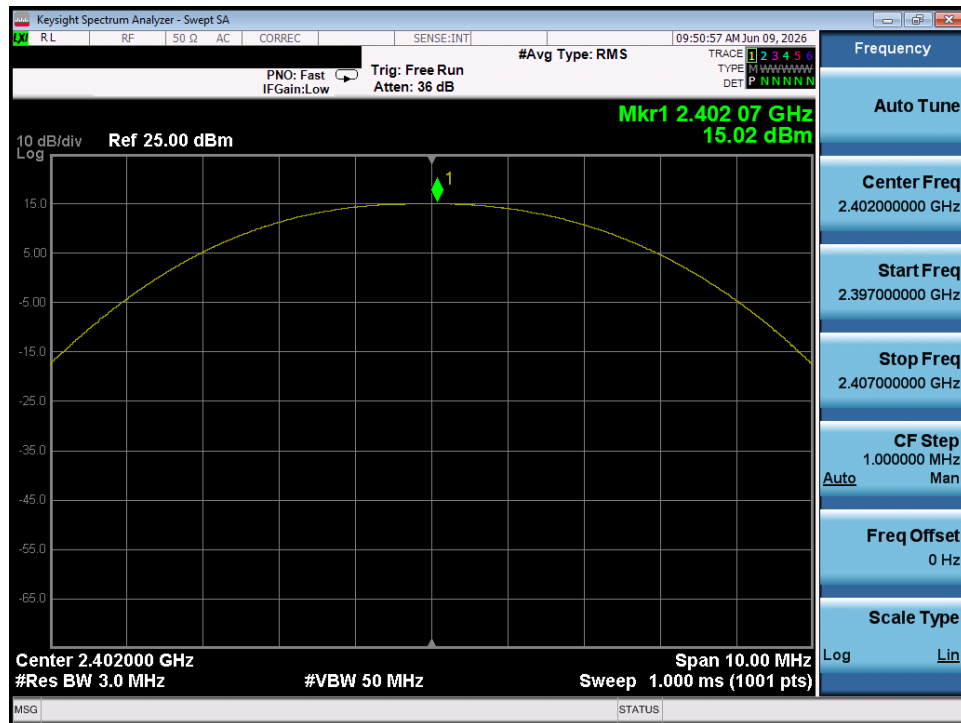
Plot 7-1. Peak Power Plot (Bluetooth (LE), 125kbps – Ch. 37) – Chain 0
