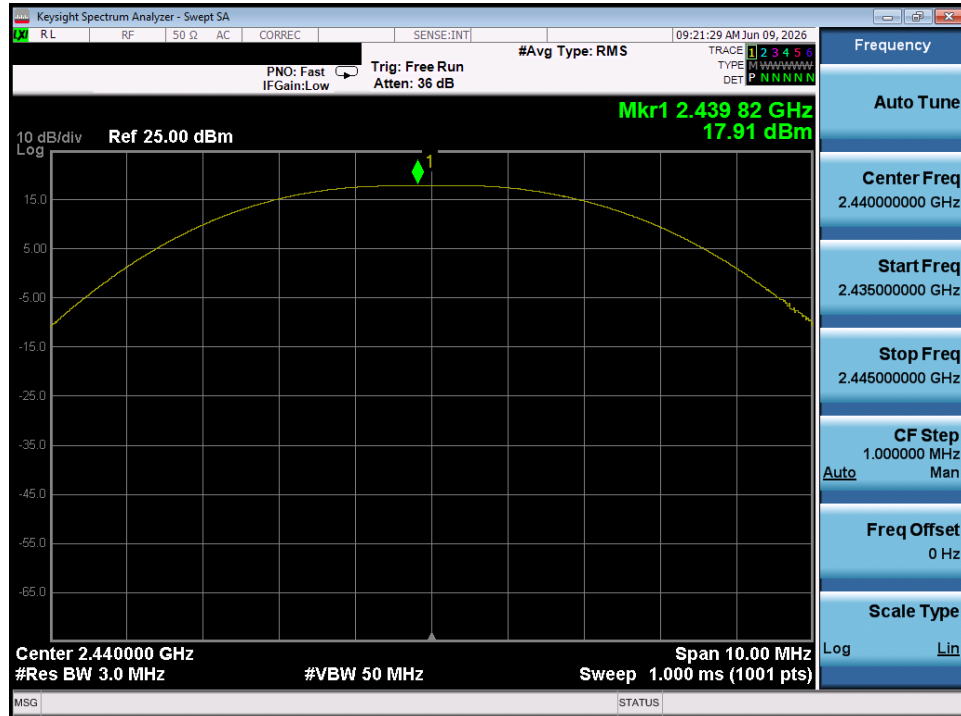
Plot 7-11. Peak Power Plot (Bluetooth (LE), 2Mbps - Ch. 17) - Chain 0
