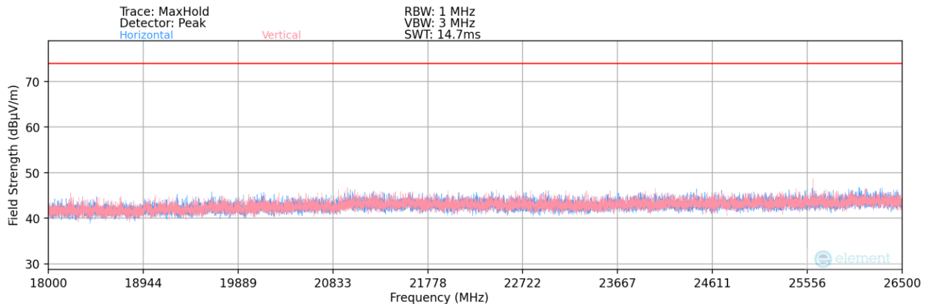
Plot 7-51. Radiated Spurious Plot above 18GHz (Bluetooth (LE))
