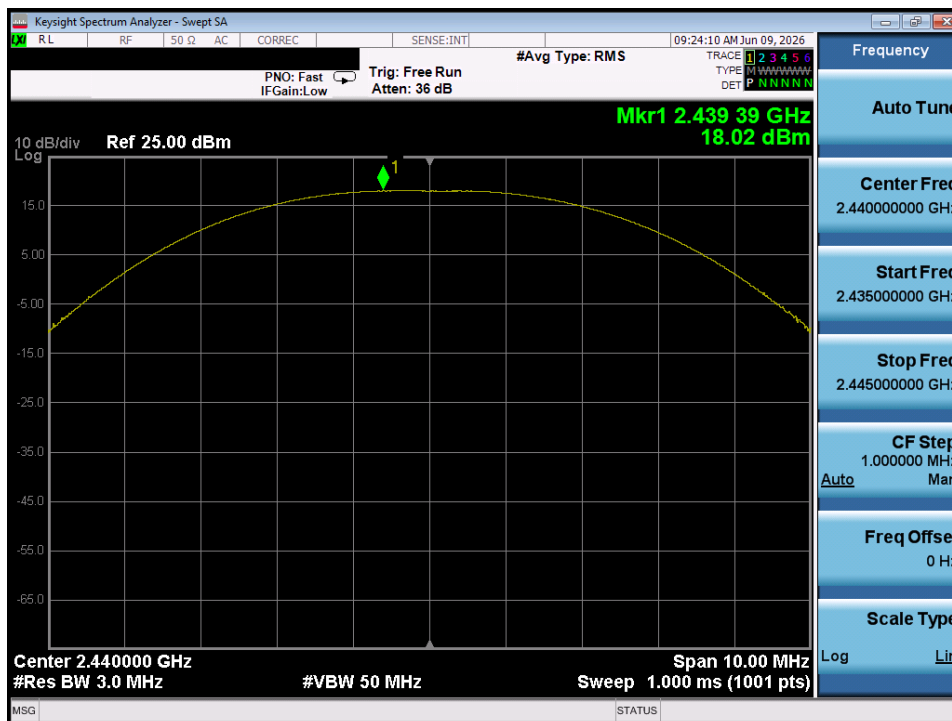
Plot 7-23. Peak Power Plot (Bluetooth (LE), 2Mbps – Ch. 17) – Chain 1
