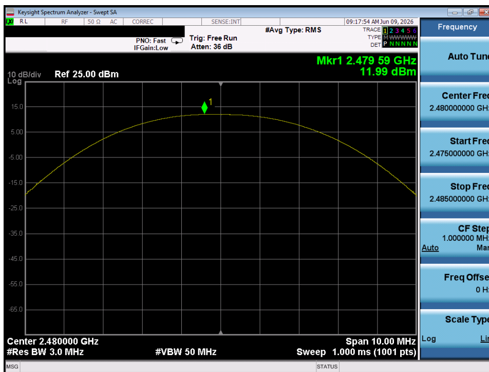
Plot 7-33. Peak Power Plot (Bluetooth (LE), 1Mbps - Ch. 39) - Dual Chain 0
