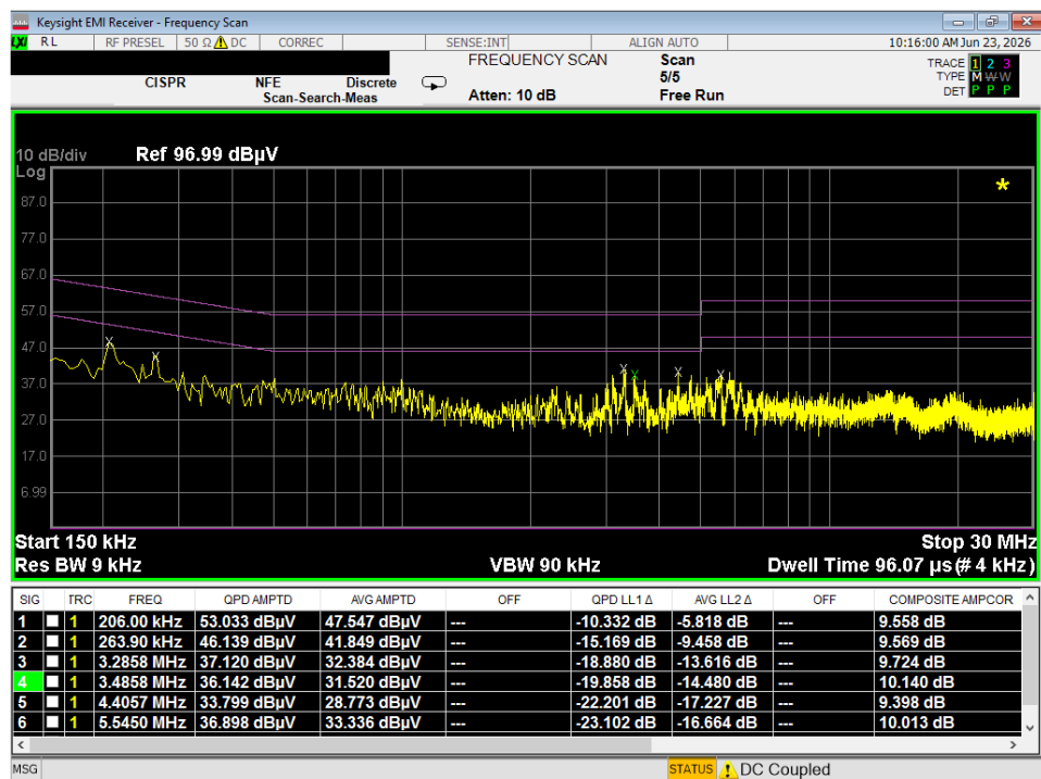
Plot 7-60. Line-Conducted Test Plot (L1)
