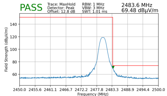
Plot 7-55. Radiated Restricted Upper Band Edge Measurement (Peak)
