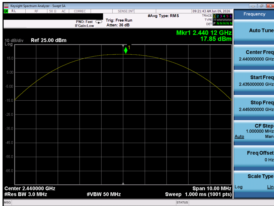
Plot 7-8. Peak Power Plot (Bluetooth (LE), 1Mbps – Ch. 17) – Chain 0
