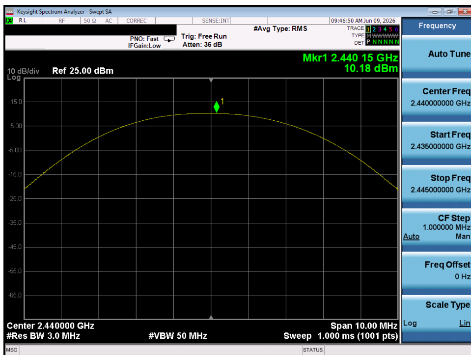
Plot 7-29. Peak Power Plot (Bluetooth (LE), 500kbps – Ch. 17) – Dual Chain 0
