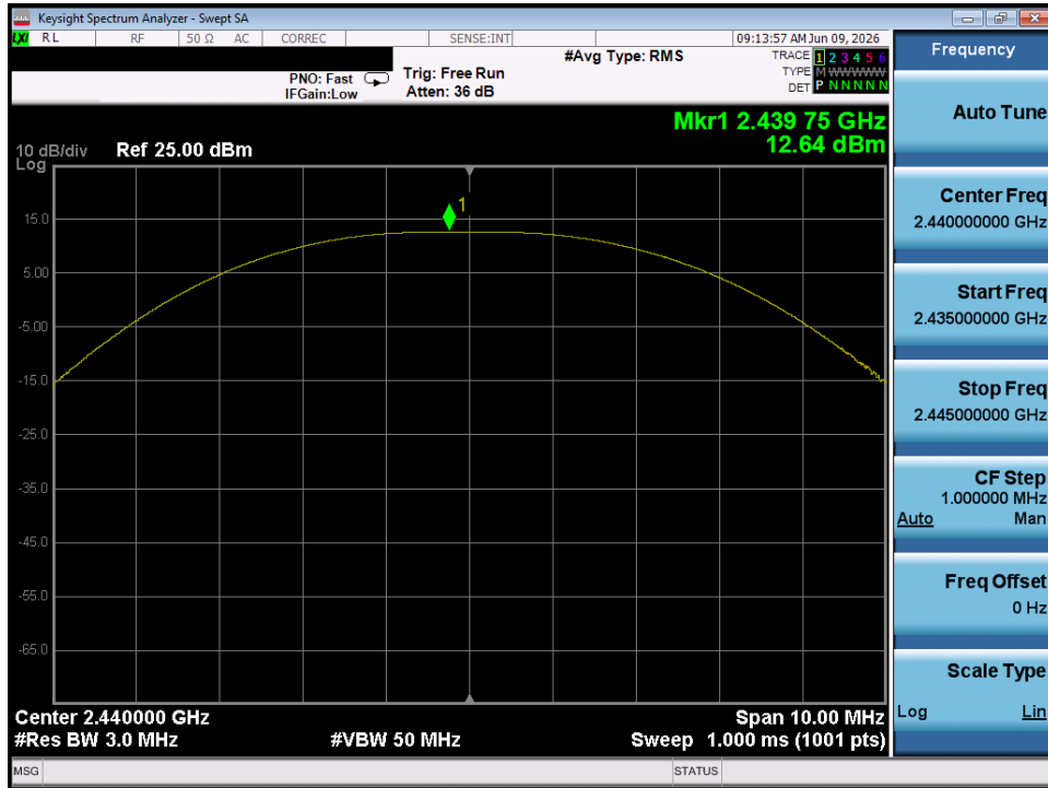
Plot 7-47. Peak Power Plot (Bluetooth (LE), 2Mbps – Ch. 17) – Dual Chain 1
