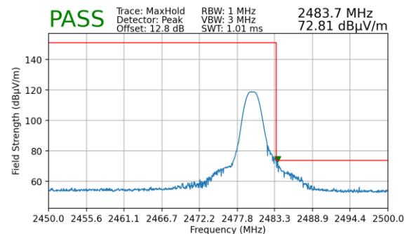
Plot 7-59. Radiated Restricted Upper Band Edge Measurement (Peak)
