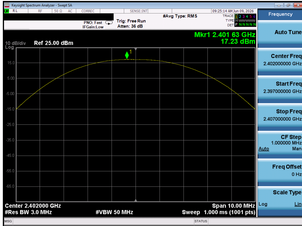
Plot 7-19. Peak Power Plot (Bluetooth (LE), 1Mbps - Ch. 37) - Chain 1
