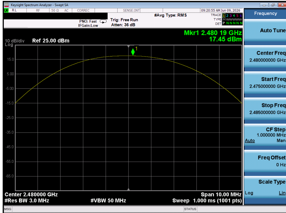
Plot 7-9. Peak Power Plot (Bluetooth (LE), 1Mbps – Ch. 39) – Chain 0
