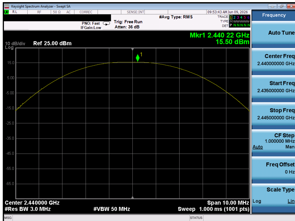
Plot 7-14. Peak Power Plot (Bluetooth (LE), 125kbps - Ch. 17) - Chain 1
