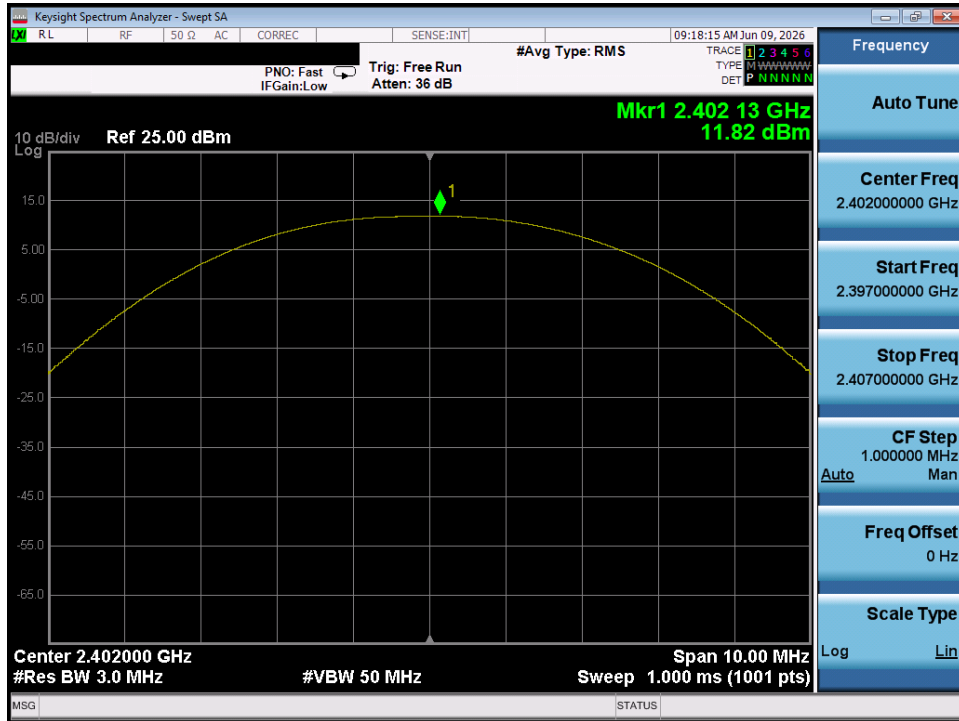
Plot 7-31. Peak Power Plot (Bluetooth (LE), 1Mbps - Ch. 37) - Dual Chain 0
