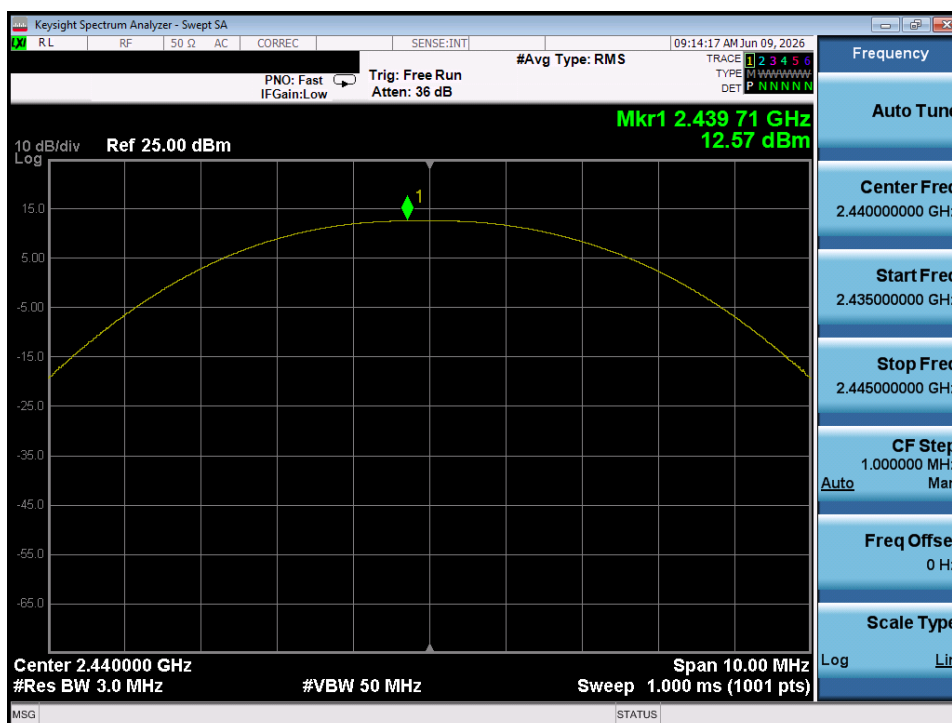
Plot 7-44. Peak Power Plot (Bluetooth (LE), 1Mbps – Ch. 17) – Dual Chain 1
