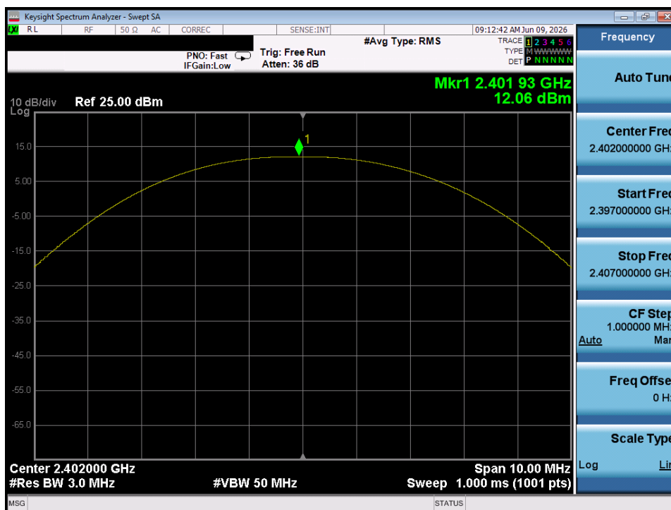
Plot 7-43. Peak Power Plot (Bluetooth (LE), 1Mbps – Ch. 37) – Dual Chain 1
