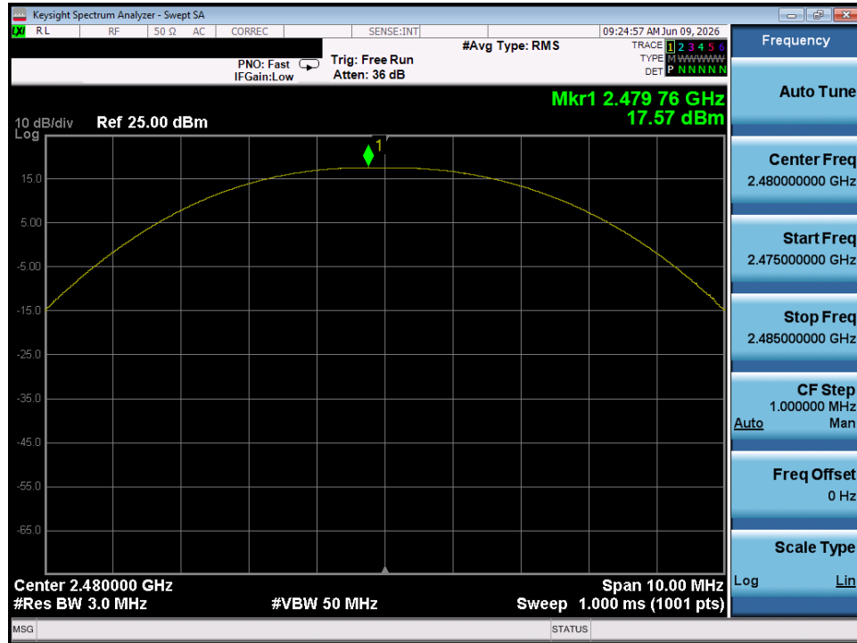
Plot 7-21. Peak Power Plot (Bluetooth (LE), 1Mbps – Ch. 39) – Chain 1
