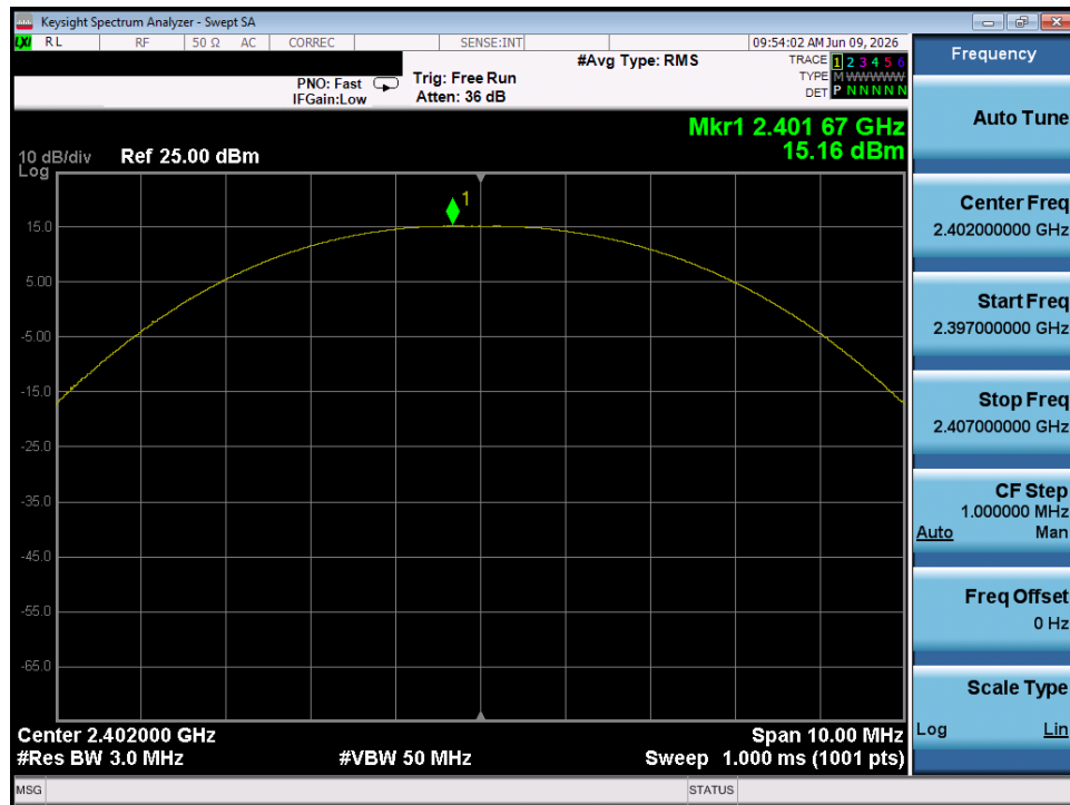
Plot 7-13. Peak Power Plot (Bluetooth (LE), 125kbps - Ch. 37) - Chain 1
