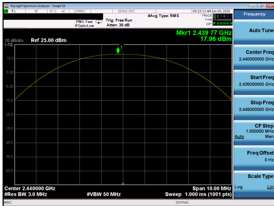
Plot 7-20. Peak Power Plot (Bluetooth (LE), 1Mbps - Ch. 17) - Chain 1
