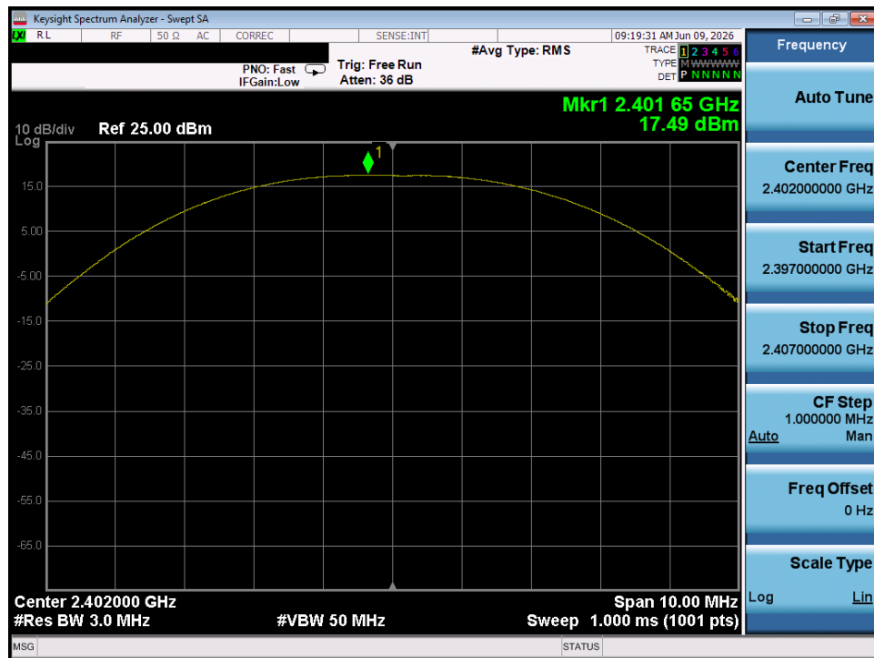
Plot 7-10. Peak Power Plot (Bluetooth (LE), 2Mbps – Ch. 0) – Chain 0
