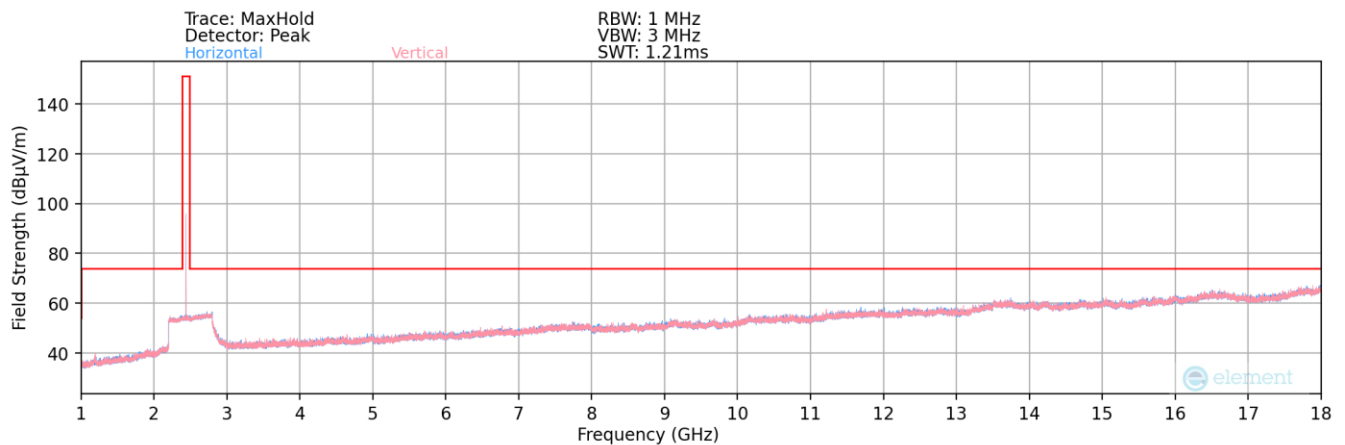
Plot 7-50. Radiated Spurious Plot above 1GHz (Bluetooth (LE))
