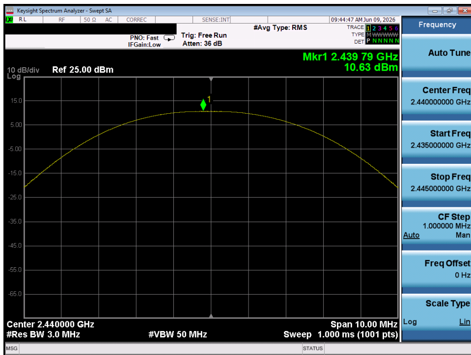
Plot 7-41. Peak Power Plot (Bluetooth (LE), 500kbps – Ch. 17) – Dual Chain 1
