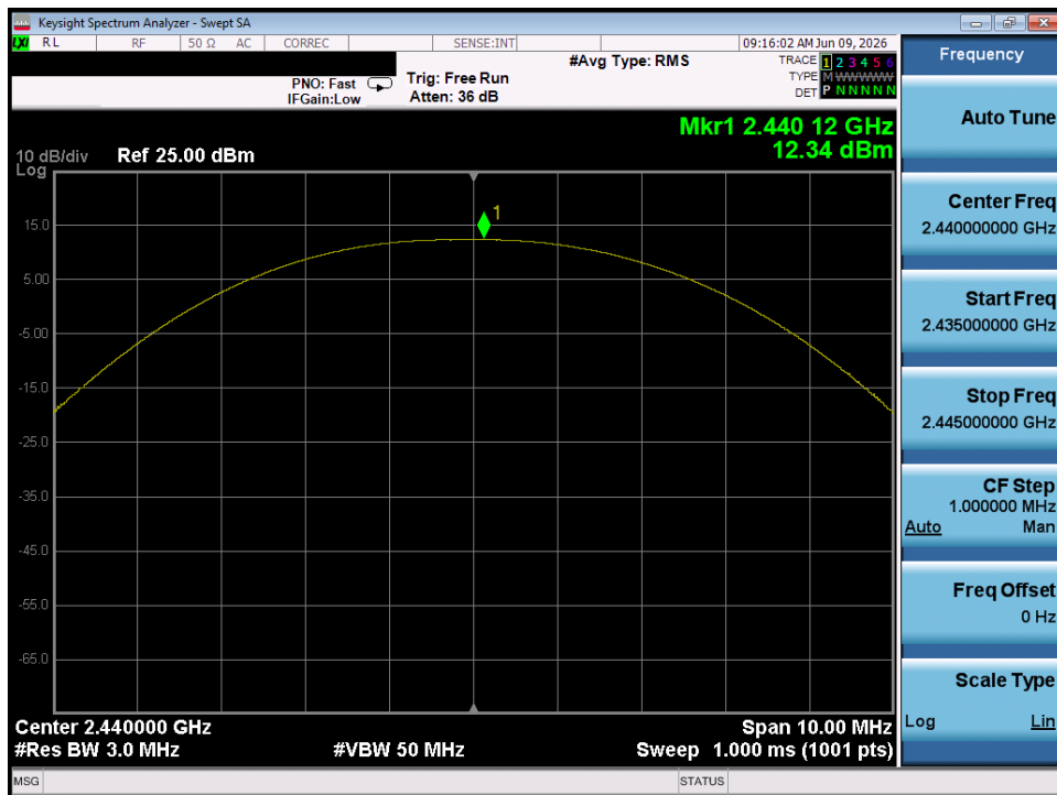
Plot 7-32. Peak Power Plot (Bluetooth (LE), 1Mbps - Ch. 17) - Dual Chain 0
