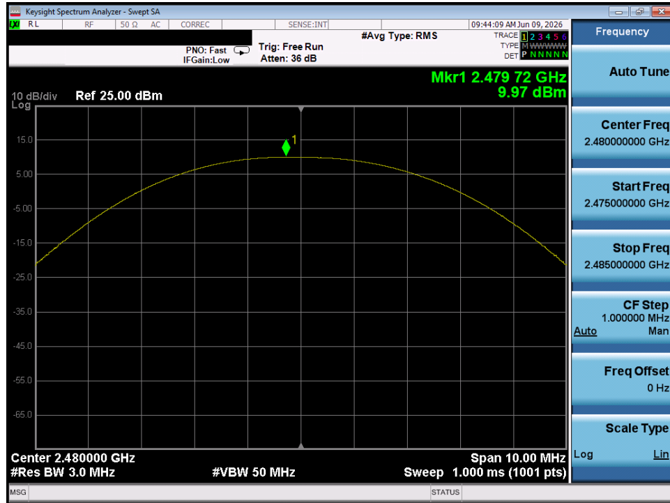
Plot 7-39. Peak Power Plot (Bluetooth (LE), 125kbps – Ch. 39) – Dual Chain 1
