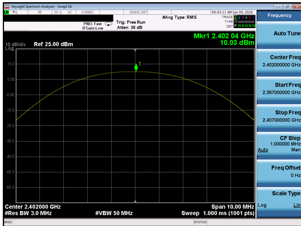
Plot 7-40. Peak Power Plot (Bluetooth (LE), 500kbps – Ch. 37) – Dual Chain 1
