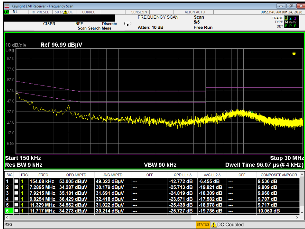
Plot 7-28. Line-Conducted Test Plot (L1)
