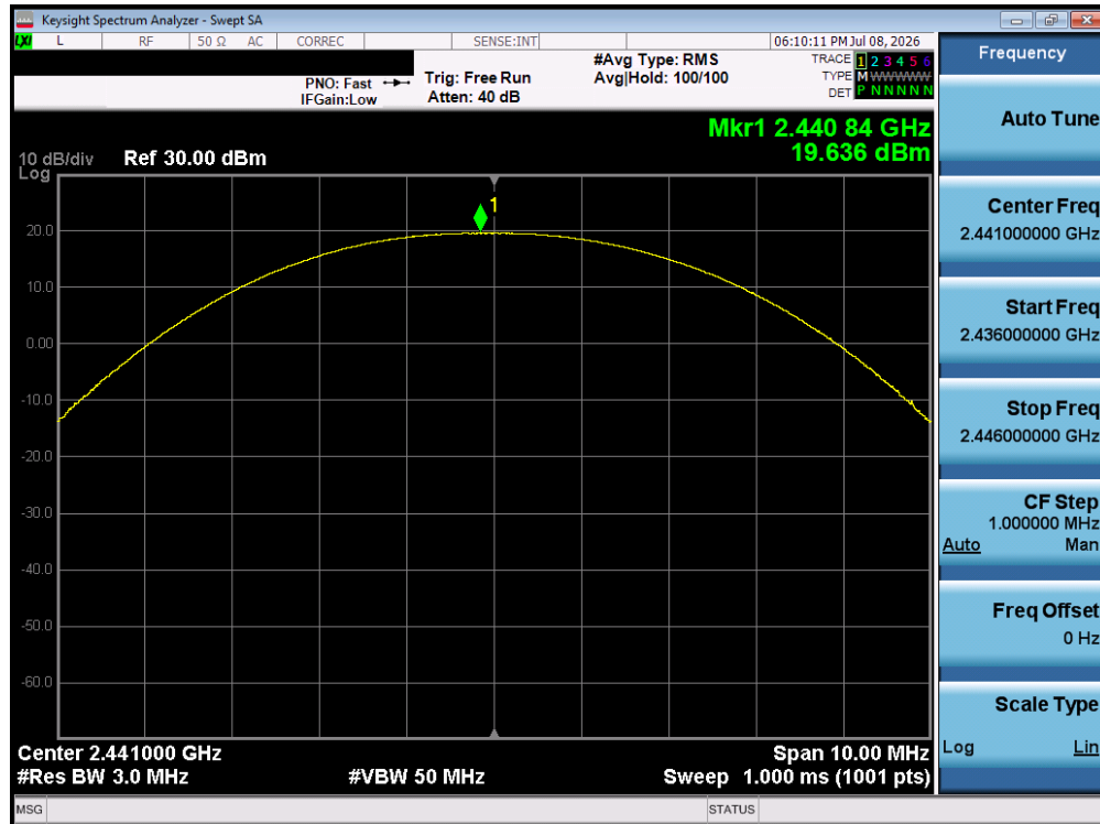
Plot 7-1. Peak Conducted Power (1Mbps – Ch. 39) – Ant0
