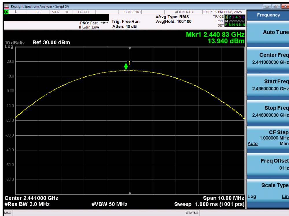
Plot 7-2. Peak Conducted Power (2Mbps – Ch. 39) – Ant0
