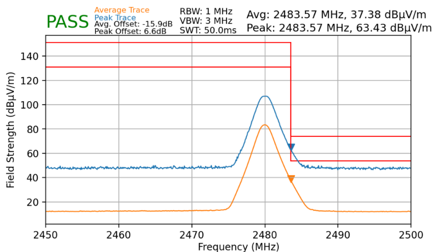
Plot 7-26. Radiated Restricted Upper Band Edge Measurement – MIMO
