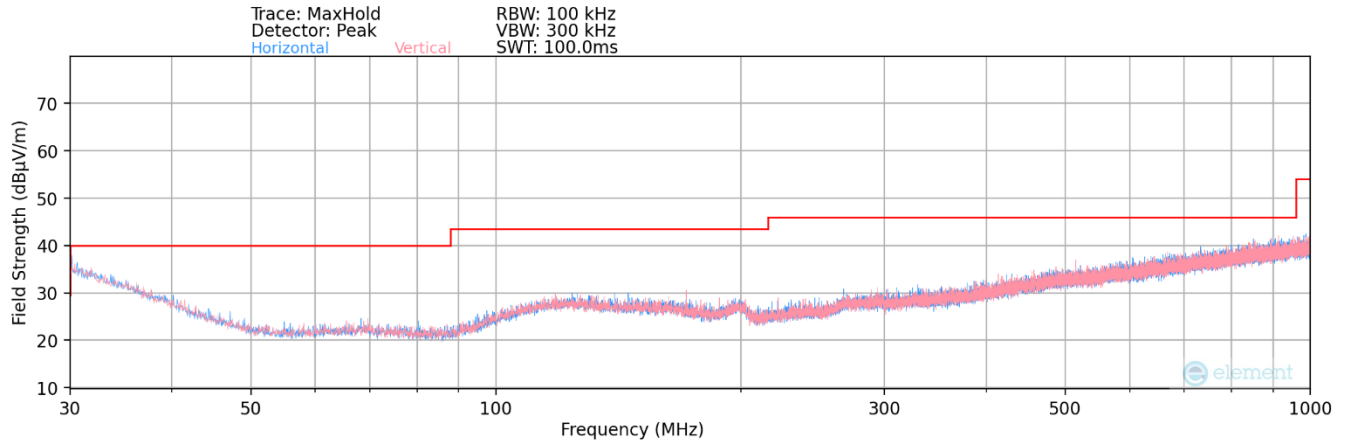
Plot 7-27. Radiated Spurious Plot below 1GHz – DUAL ANTENNA
