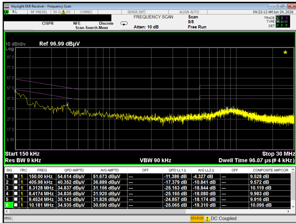
Plot 7-29. Line-Conducted Test Plot (N)
