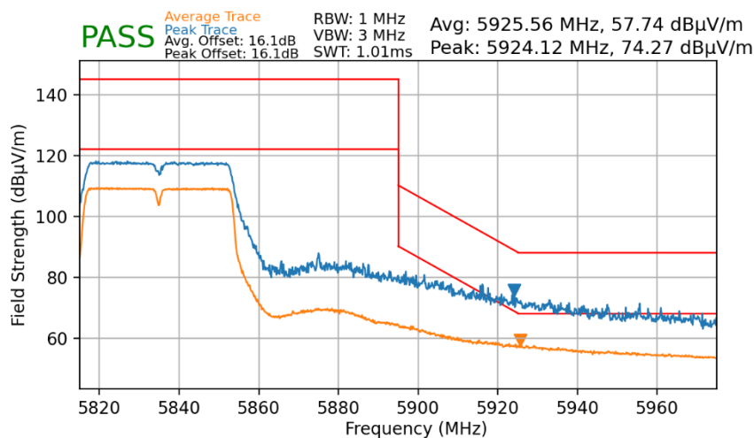
Plot 7-24. Upper Band Edge Plot MIMO (UNII Band 4)
