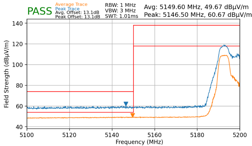
Plot 7-14. Lower Band Edge Plot MIMO (UNII Band 1) - OFDMA
