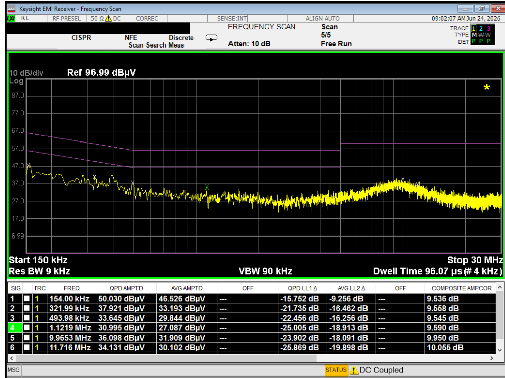
Plot 7-35. Line Conducted Plot with 802.11a UNII Band 4 – Ch.173 (L1)
