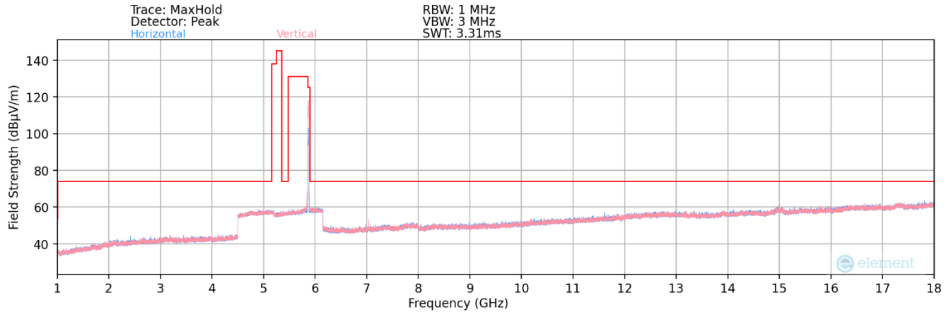
Plot 7-10. Radiated Spurious Plot above 1GHz MIMO (802.11be – UNII Band 4 Ch. 173 – 106T)
