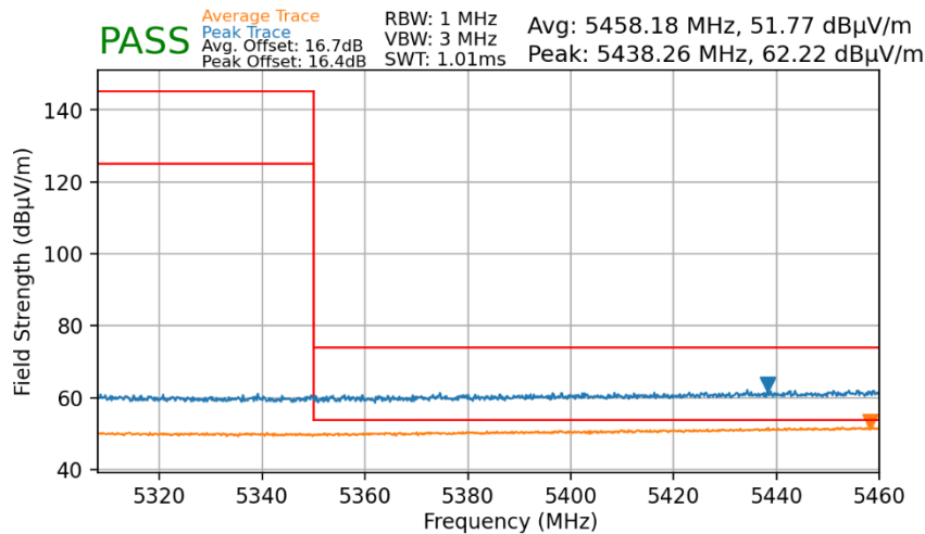
Plot 7-16. Upper Band Edge Plot MIMO (UNII Band 2A) - OFDMA
