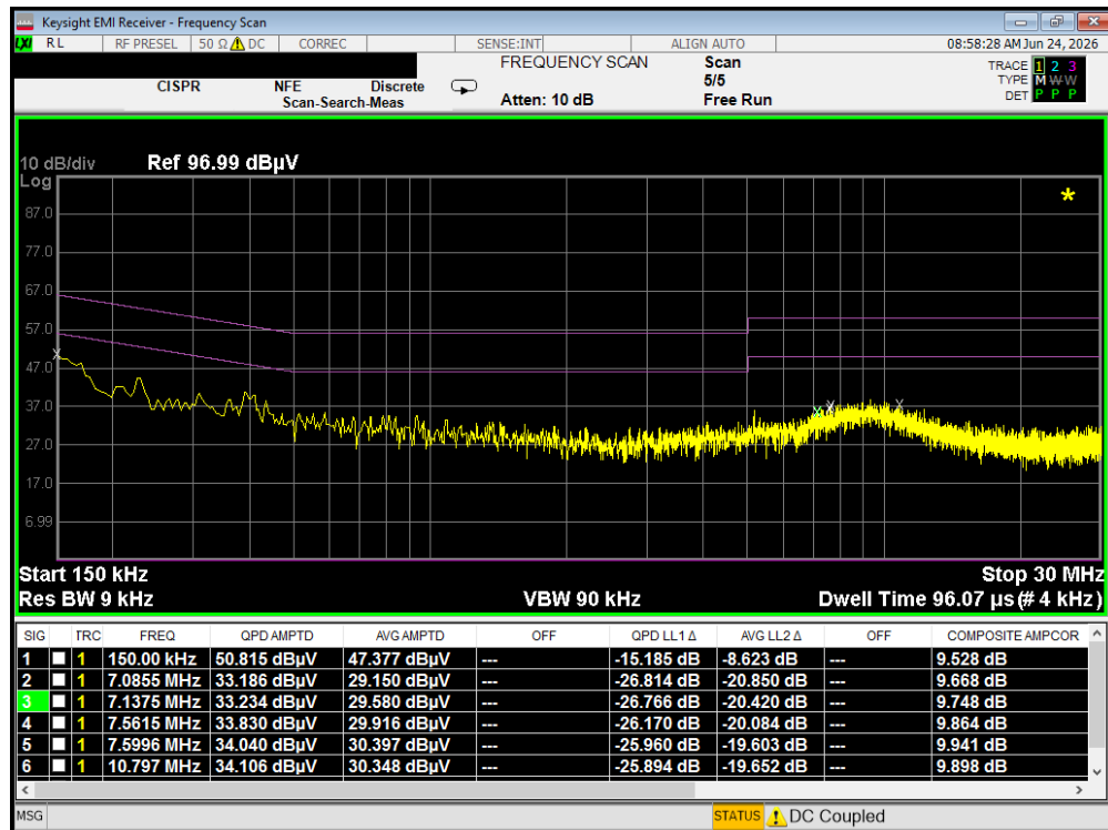
Plot 7-32. Line Conducted Plot with 802.11a UNII Band 2C – Ch.120 (N)
