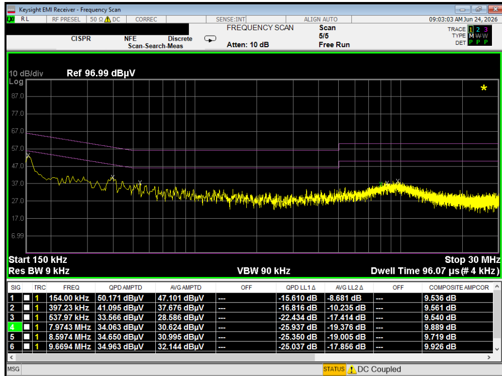
Plot 7-36. Line Conducted Plot with 802.11a UNII Band 4 – Ch.173 (N)
