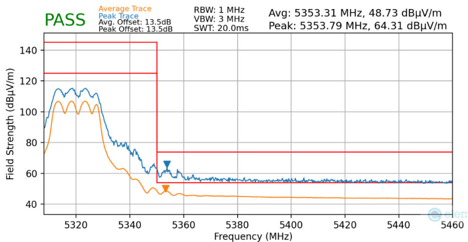
Plot 7-15. Upper Band Edge Plot MIMO (UNII Band 2A)
