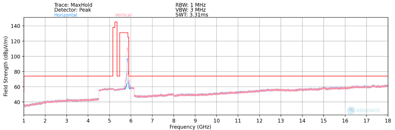
Plot 7-9. Radiated Spurious Plot above 1GHz MIMO (802.11n – UNII Band 4 Ch. 167)
