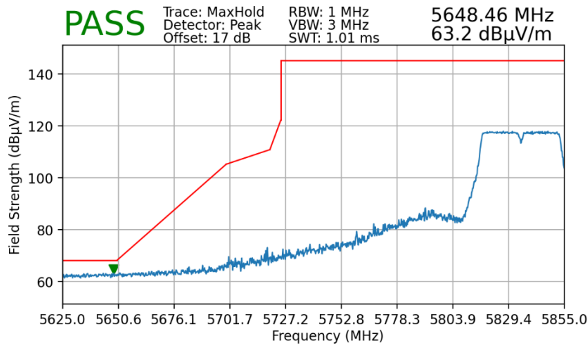
Plot 7-23. Lower Band Edge Plot MIMO (Peak – UNII Band 4)
