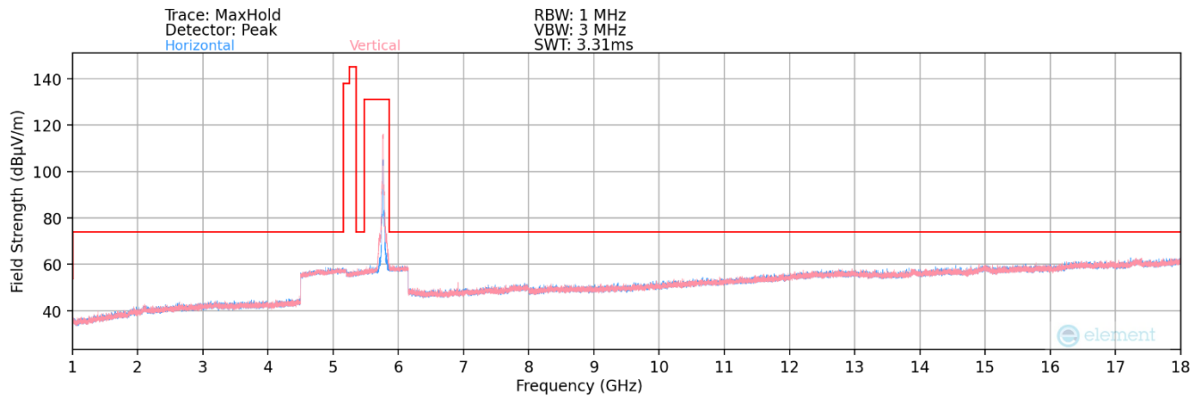
Plot 7-8. Radiated Spurious Plot above 1GHz MIMO (802.11n – UNII Band 3 Ch. 153)
