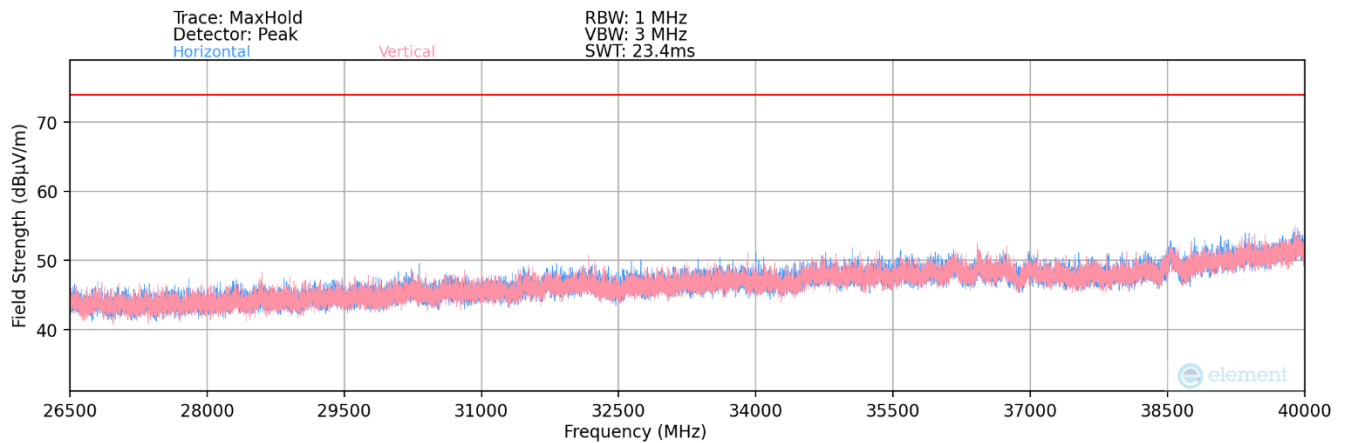
Plot 7-12. Radiated Spurious Plot 26.5GHz – 40GHz MIMO (802.11n – Ch.40)
