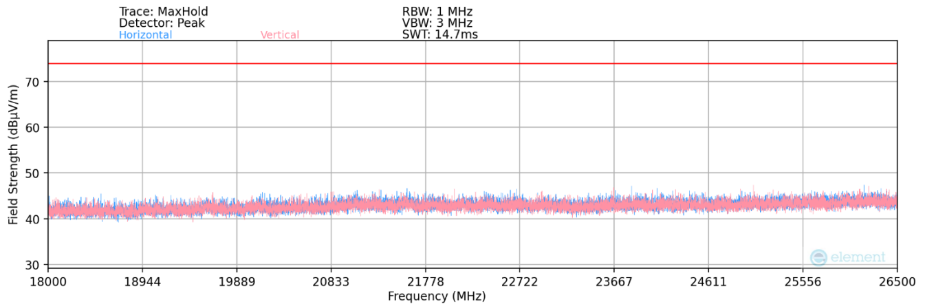
Plot 7-11. Radiated Spurious Plot 18GHz – 26.5GHz MIMO (802.11n – Ch.40)
