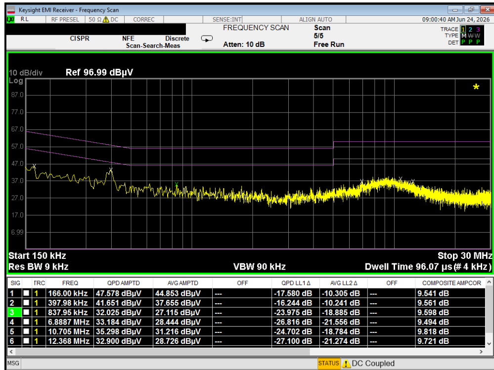
Plot 7-33. Line Conducted Plot with 802.11a UNII Band 3 – Ch.157 (L1)
