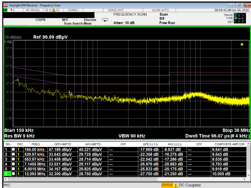
Plot 7-34. Line Conducted Plot with 802.11a UNII Band 3 – Ch.157 (N)
