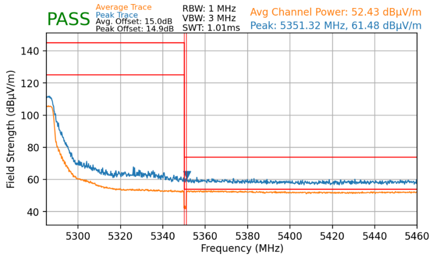
Plot 7-21. Upper Band Edge Plot MIMO (Average – UNII Band 2A)
