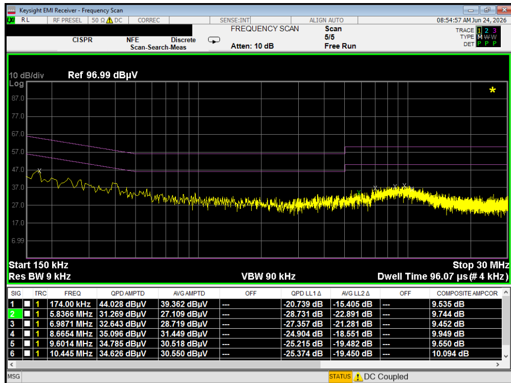
Plot 7-30. Line Conducted Plot with 802.11a UNII Band 2A – Ch.56 (N)
