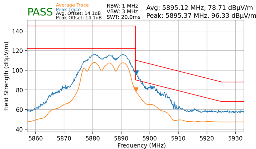
Plot 7-20. Upper Band Edge Plot MIMO (UNII Band 4)
