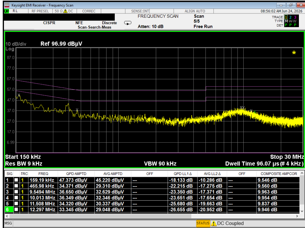
Plot 7-29. Line Conducted Plot with 802.11a UNII Band 2A – Ch.56 (L1)
