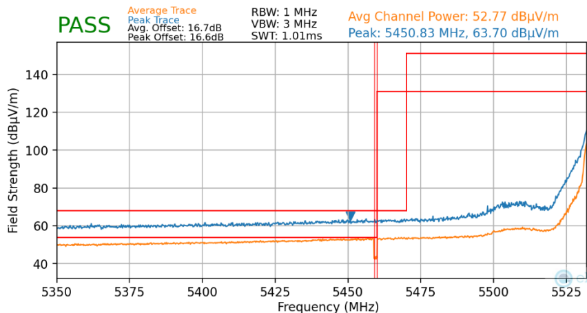
Plot 7-22. Lower Band Edge Plot MIMO (UNII Band 2C)
