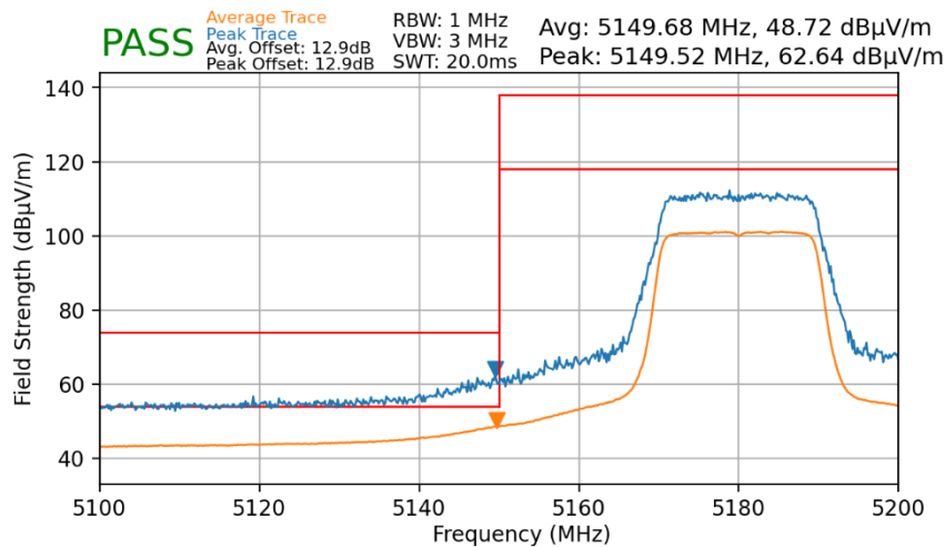
Plot 7-13. Lower Band Edge Plot MIMO (UNII Band 1)
