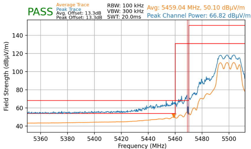
Plot 7-17. Lower Band Edge Plot MIMO (UNII Band 2C)
