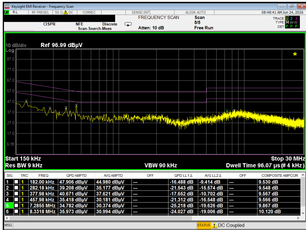
Plot 7-27. Line Conducted Plot with 802.11a UNII Band 1 – Ch.40 (L1)
