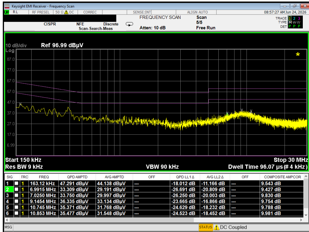
Plot 7-31. Line Conducted Plot with 802.11a UNII Band 2C – Ch.120 (L1)
