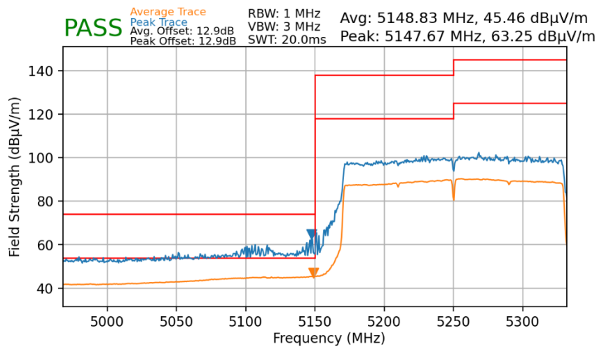
Plot 7-26. Lower Band Edge Plot MIMO (UNII Band 1)
