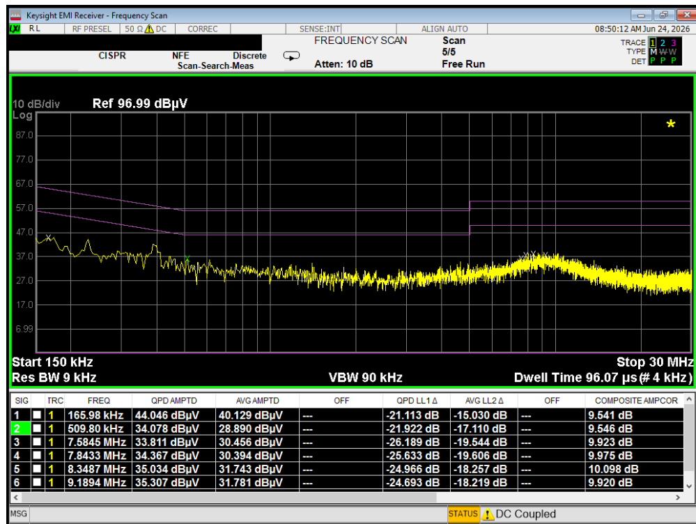
Plot 7-28. Line Conducted Plot with 802.11a UNII Band 1 – Ch.40 (N)
