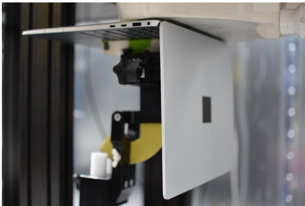
SAR Test Setup Photo 1 – Motion, Bottom Side at 0 mm – Antenna Chain 0 & Chain 1
