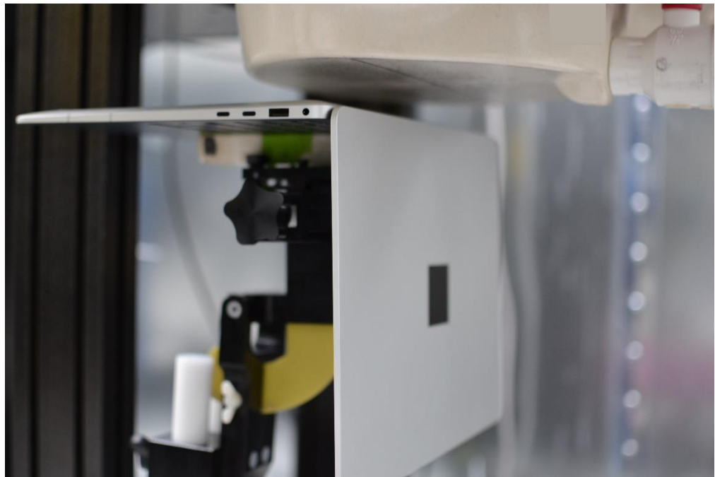
SAR Test Setup Photo 8 – No Motion, Bottom Side at 25 mm – Antenna Chain 0 & Chain 1
