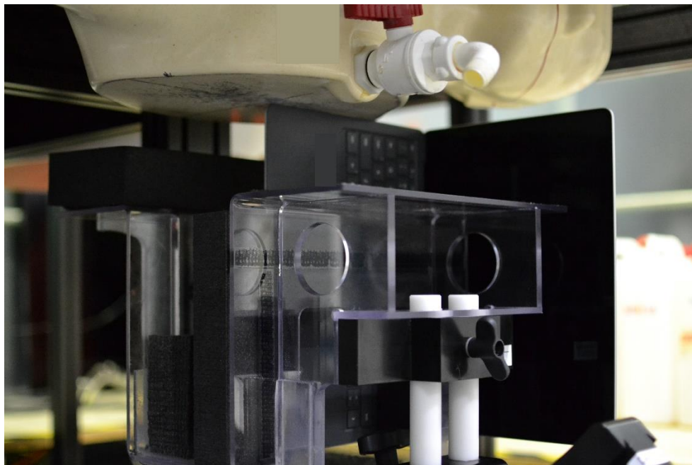
SAR Test Setup Photo 15 – Motion, Left Edge at 0 mm
