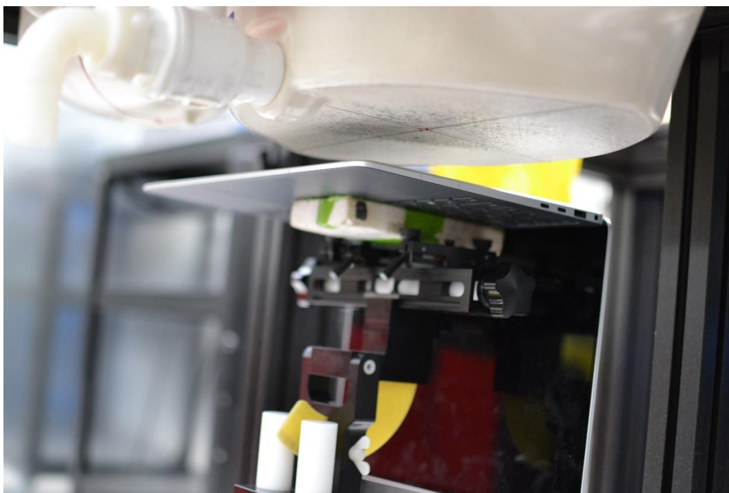
SAR Test Setup Photo 2 – No Motion, Bottom Side at 25 mm – Antenna 1 & 2
