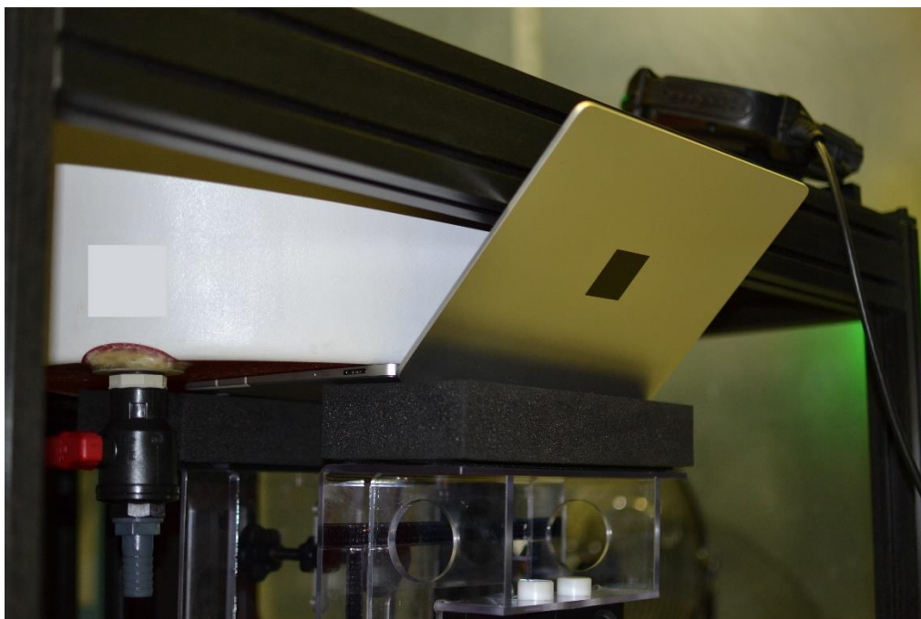
SAR Test Setup Photo 19 – Motion, Top Side at 0 mm
