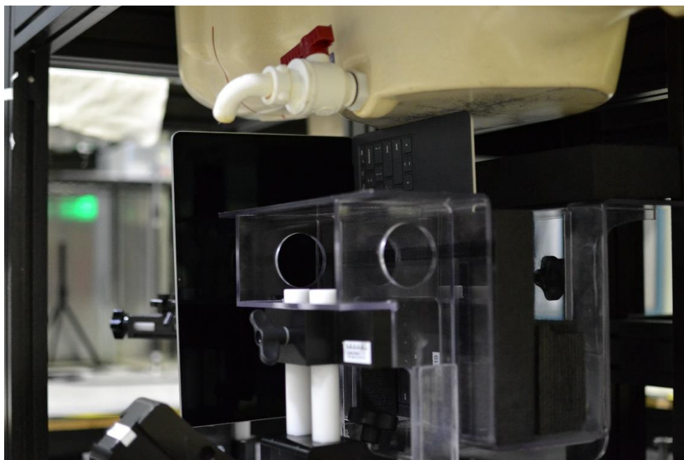
SAR Test Setup Photo 17 – Motion, Right Edge at 0 mm
