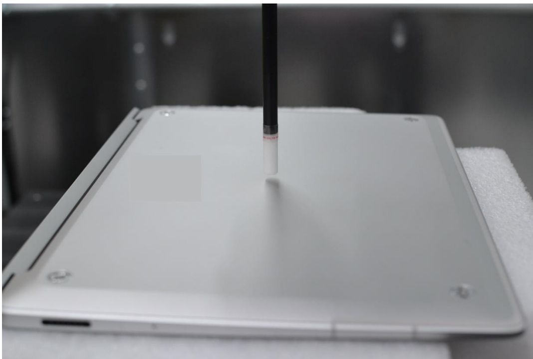
Near Field Power Density Test Setup Photo 21 – Bottom Side at 2 mm
