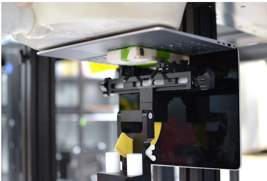
SAR Test Setup Photo 3 – Motion, Bottom Side at 0 mm – Antenna 3 & 4
