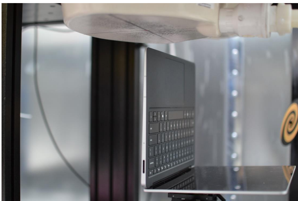
SAR Test Setup Photo 14 – No Motion, Front Edge at 25 mm – Antenna 5 & 6
