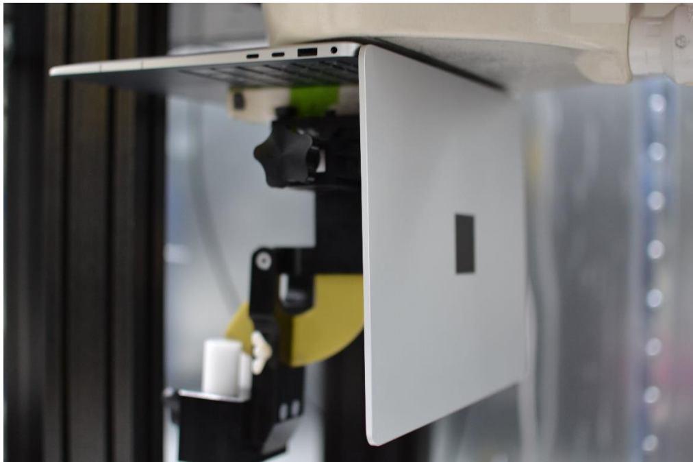
SAR Test Setup Photo 7 – Motion, Bottom Side at 0 mm – Antenna Chain 0 & Chain 1
