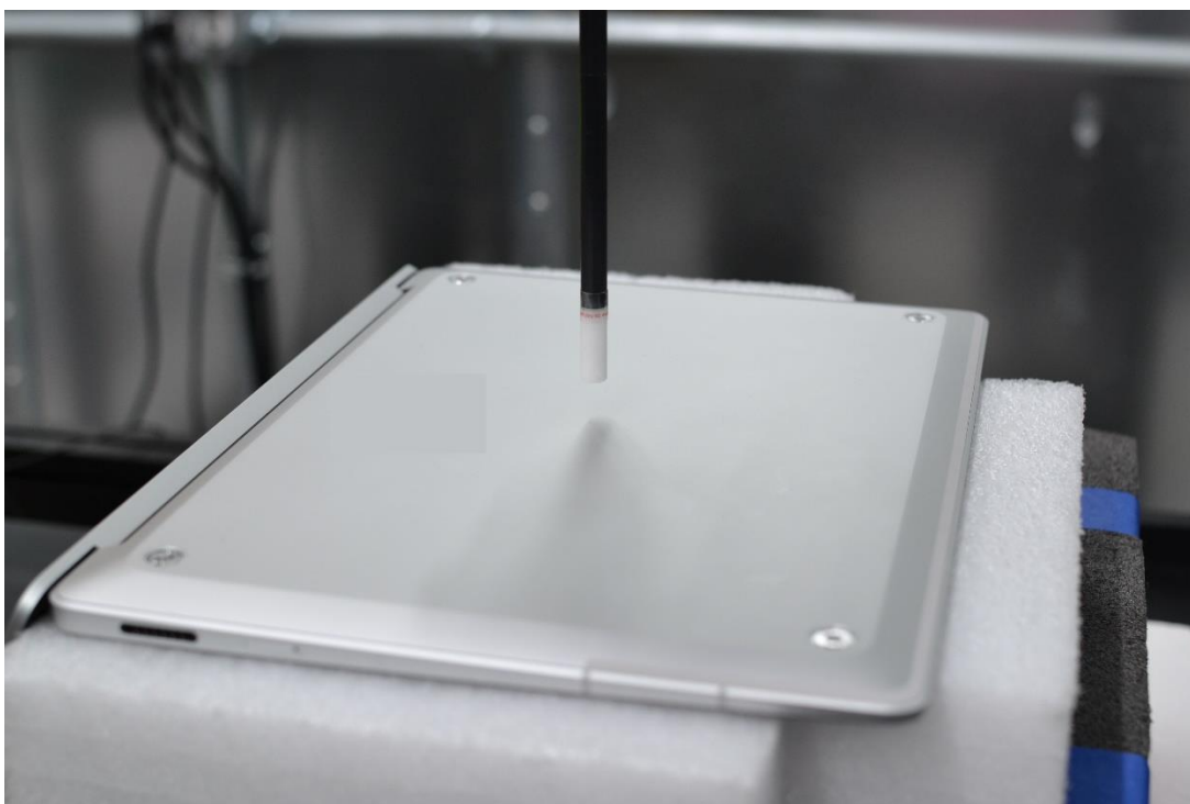
Near Field Power Density Test Setup Photo 22 – Bottom Side at 9.52 mm
