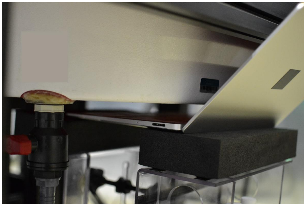
SAR Test Setup Photo 20 – No Motion, Top Side at 25 mm
