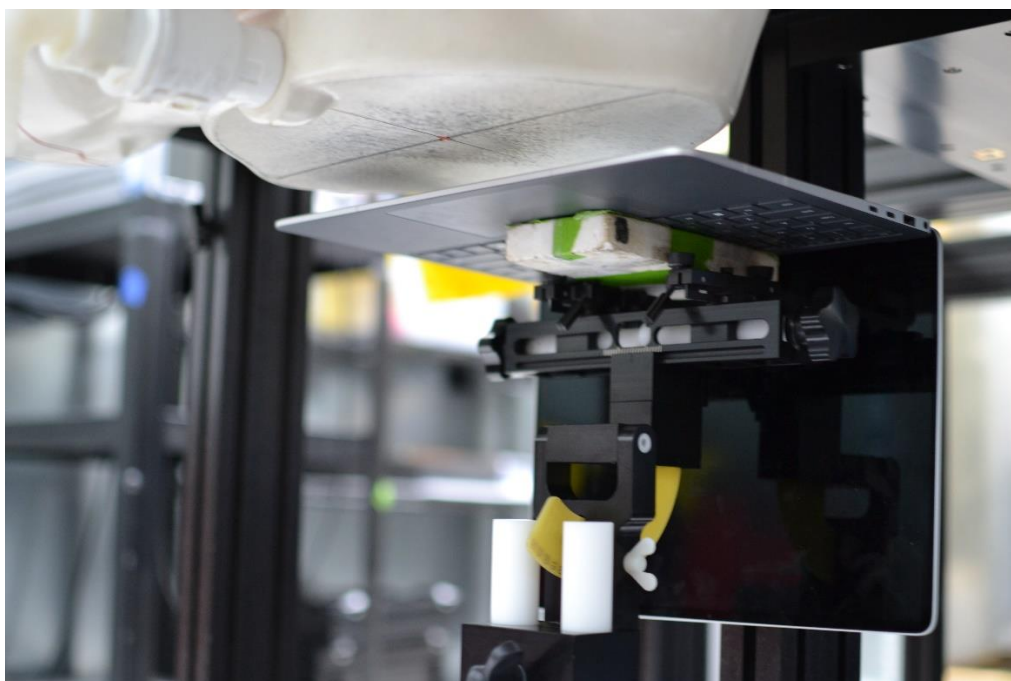
SAR Test Setup Photo 4 – No Motion, Bottom Side at 25 mm – Antenna 3 & 4
